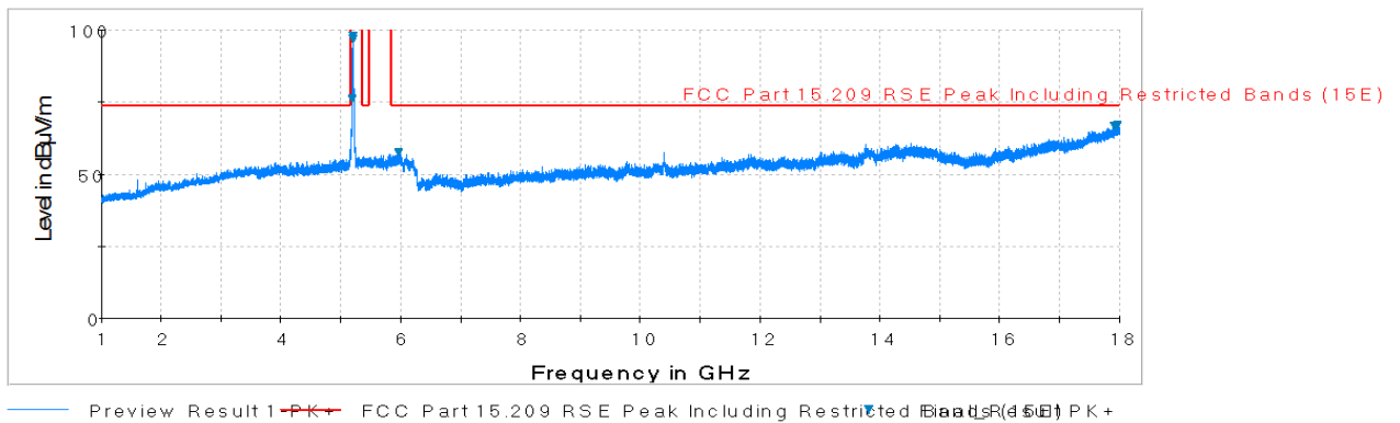
Plot 7-68. Radiated Spurious Plot above 1GHz (802.11a – U1 Ch. 40, Ant. Pol. V)
