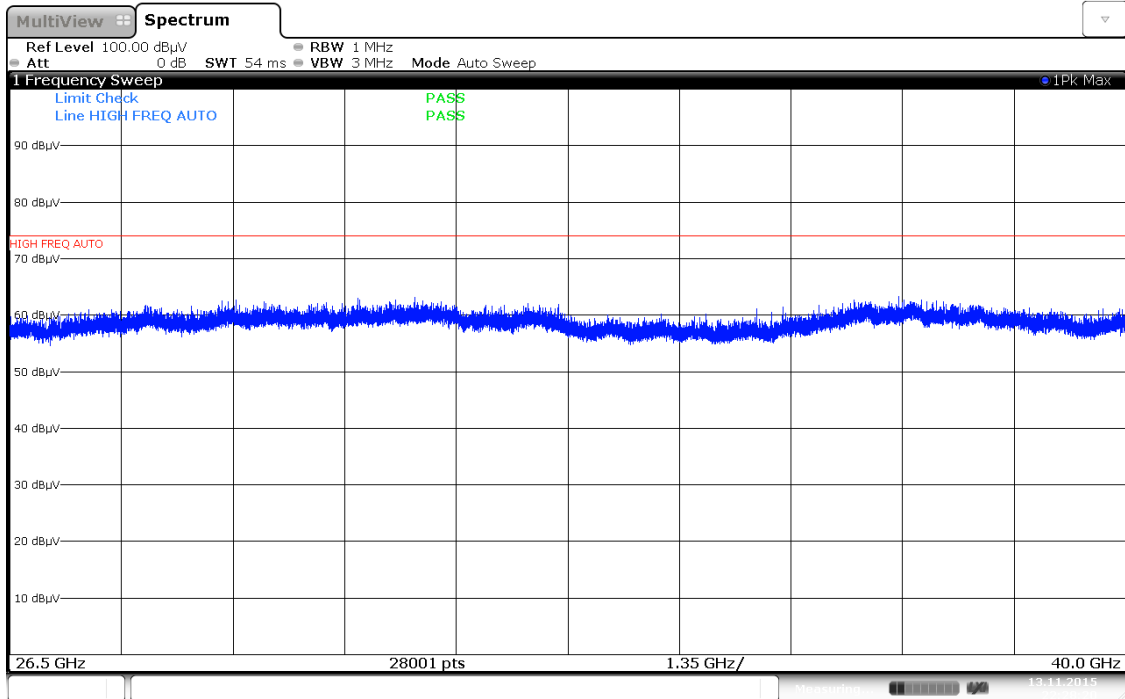
Plot 7-76. Radiated Spurious Plot above 18GHz (802.11a – Ant. Pol. H, 26.5GHz – 40GHz)
