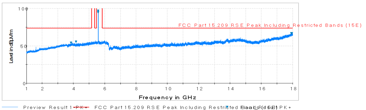
Plot 7-71. Radiated Spurious Plot above 1GHz (802.11a – U2C Ch. 120, Ant. Pol. H)
