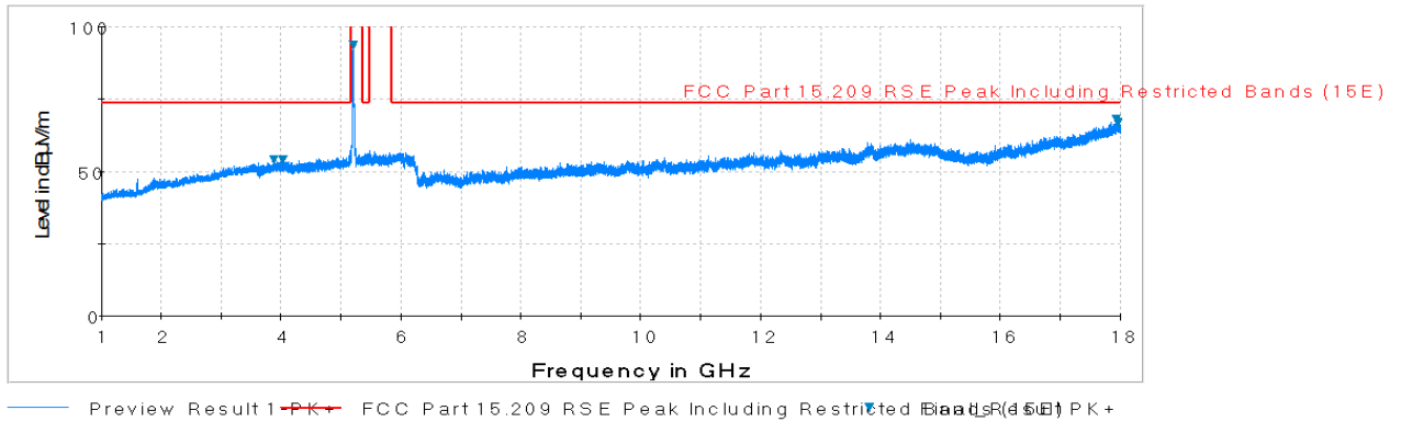
Plot 7-67. Radiated Spurious Plot above 1GHz (802.11a – U1 Ch. 40, Ant. Pol. H)
