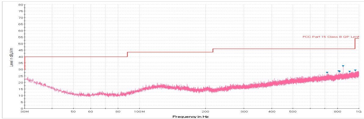
Plot 7-94. Radiated Spurious Plot below 1GHz (802.11a – U3 Ch. 157, Ant. Pol. V)
