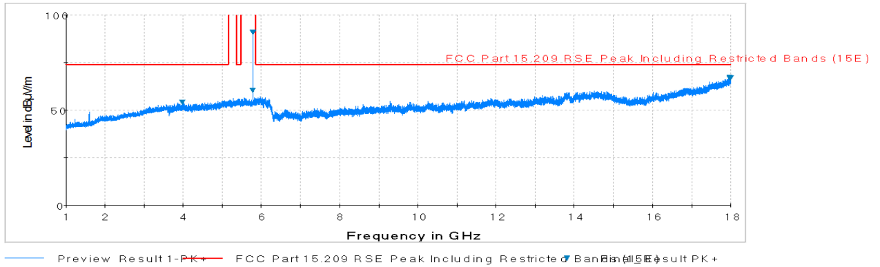
Plot 7-73. Radiated Spurious Plot above 1GHz (802.11a – U3 Ch. 157, Ant. Pol. H)
