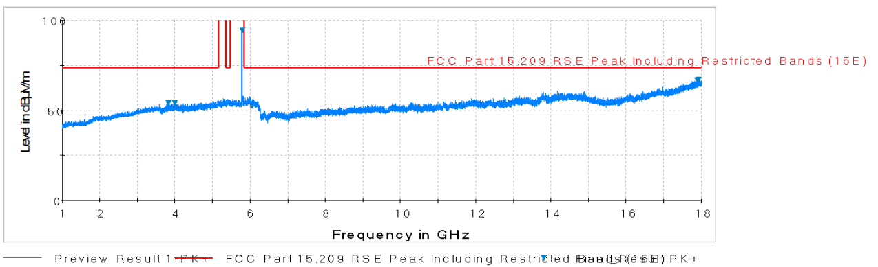
Plot 7-74. Radiated Spurious Plot above 1GHz (802.11a – U3 Ch. 157, Ant. Pol. V)
