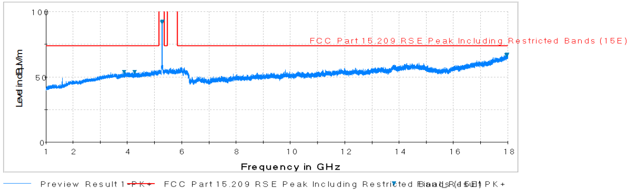
Plot 7-70. Radiated Spurious Plot above 1GHz (802.11a – U2A Ch. 56, Ant. Pol. V)
