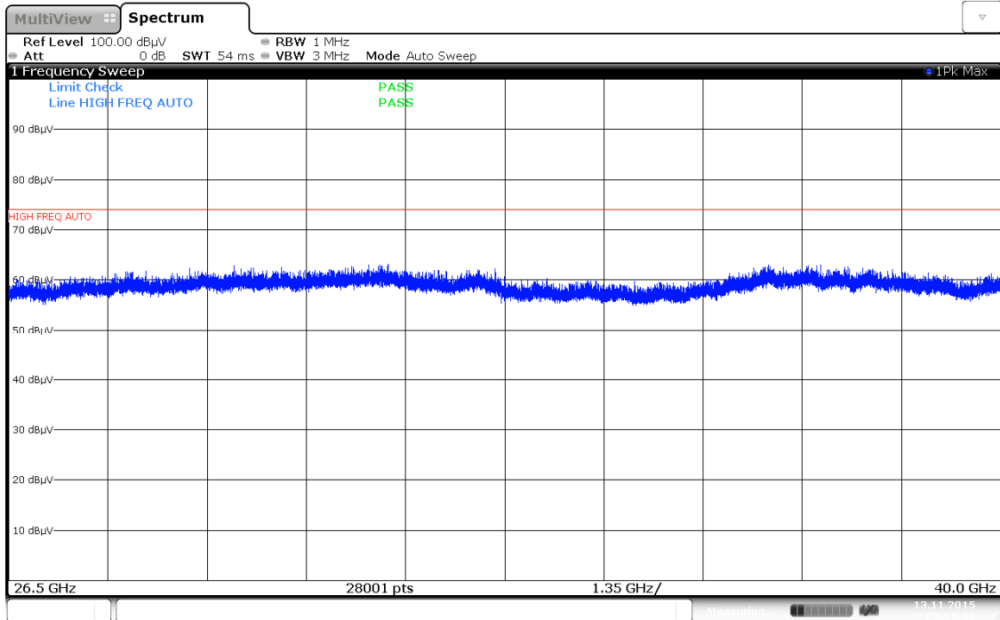
Plot 7-78. Radiated Spurious Plot above 18GHz (802.11a – Ant. Pol. V, 26.5GHz – 40GHz)
