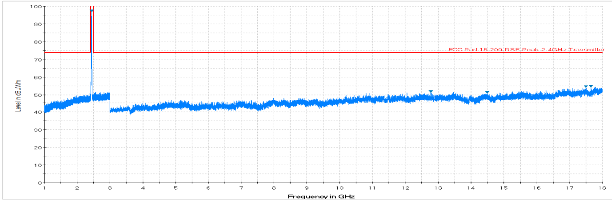
Plot 7-37. Radiated Spurious Plot above 1GHz (802.11b – Ch. 6, Ant. Pol. V)
