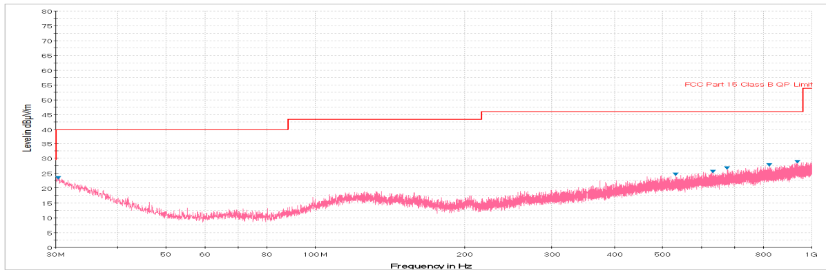
Plot 7-48. Radiated Spurious Plot below 1GHz (Pol. H)
