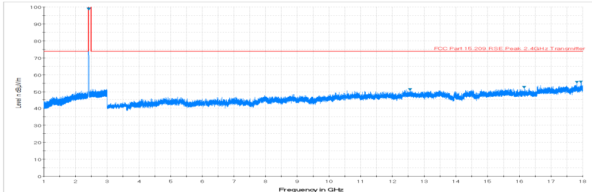
Plot 7-34. Radiated Spurious Plot above 1GHz (802.11b – Ch. 1, Ant. Pol. H)
