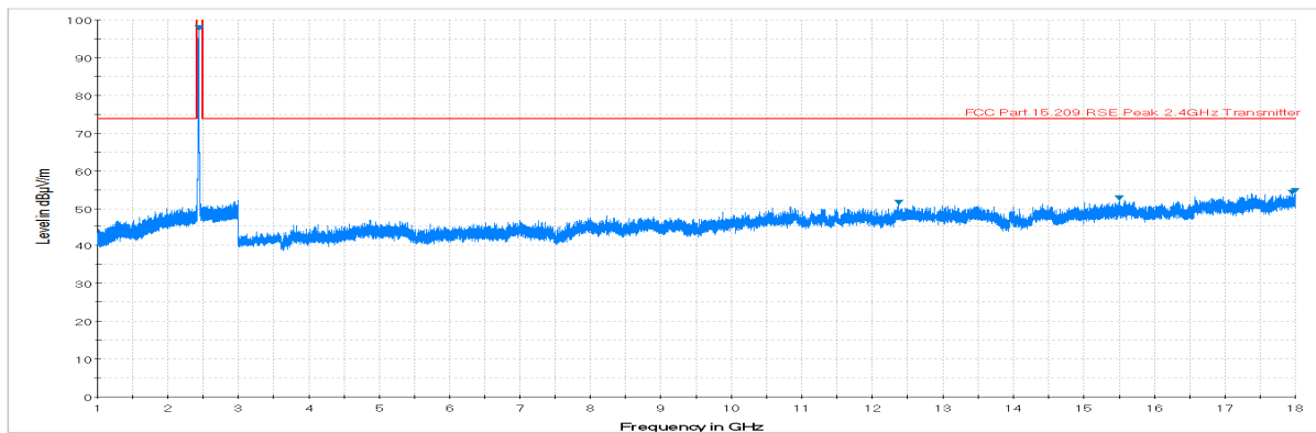
Plot 7-36. Radiated Spurious Plot above 1GHz (802.11b – Ch. 6, Ant. Pol. H)
