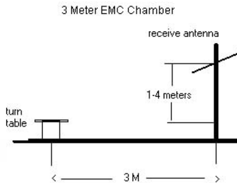
Figure 7-7. Test Instrument & Measurement Setup
