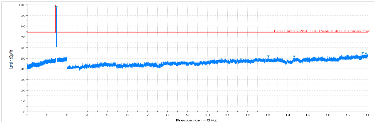
Plot 7-39. Radiated Spurious Plot above 1GHz (802.11b – Ch. 11, Ant. Pol. V)
