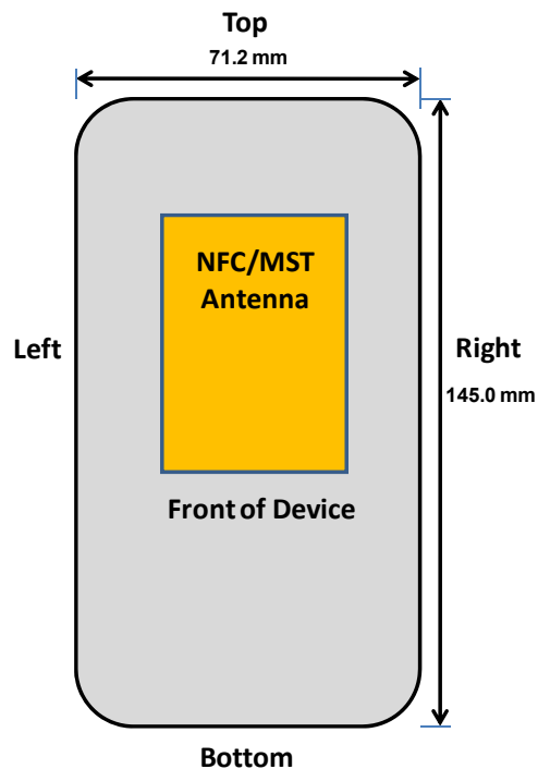
Figure F-2 NFC Antenna Locations
