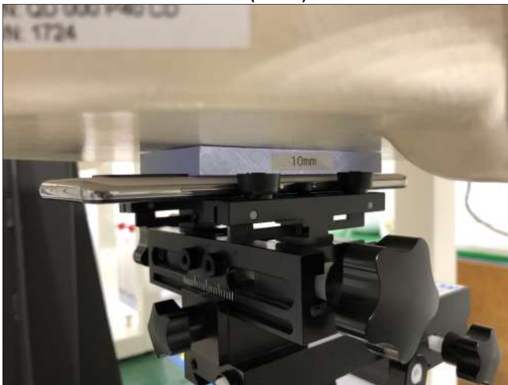
Rear (10mm)
