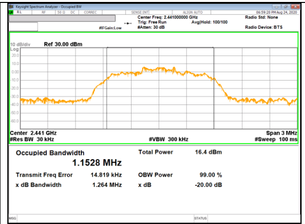
20 dB bandwidth / 39 CHANNEL
