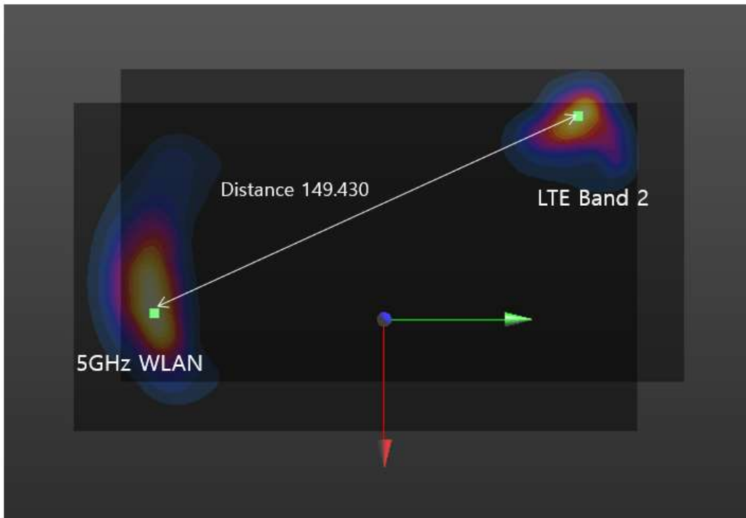
Plot #4 LTE Band 2 + WLAN 5GHz
