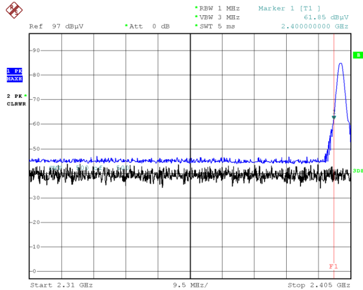
Radiated Band Edges plot – Ch.0
