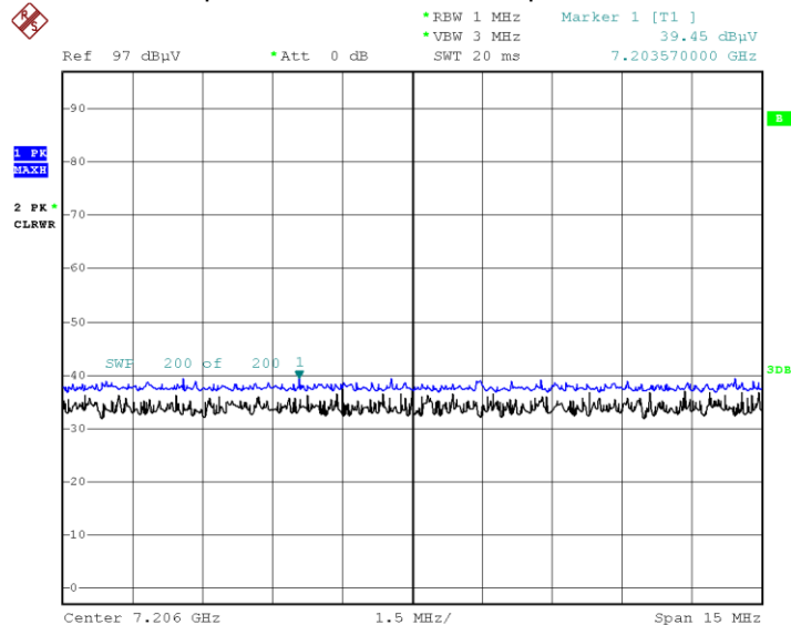
Radiated Spurious Emissions Peak plot – Ch.0 3rd Harmonic
