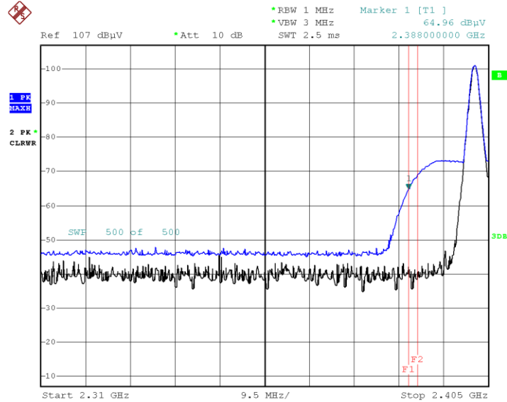
Radiated Restricted Band Edges plot – Peak & Average Reading (GFSK, Ch.0, H) 2 310 MHz ~ 2 388 MHz
