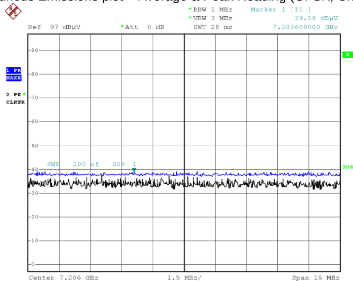
Radiated Spurious Emissions plot – Average & Peak Reading (GFSK, Ch.0 3rd Harmonic, Z-H)
