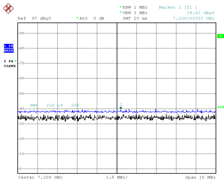
Radiated Spurious Emissions plot – Average & Peak Reading ( \pi/4 DQPSK, Ch.0 3rd Harmonic, Z-H)
