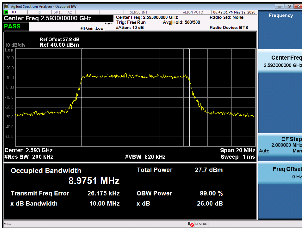
Occupied Bandwidth Plot (10 MHz Ch.40620 64-QAM RB 50) (POWER CLASS 3)
