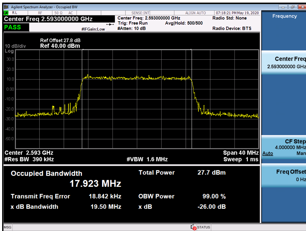
Occupied Bandwidth Plot (20 MHz Ch.40620 64-QAM RB 100) (POWER CLASS 3)
