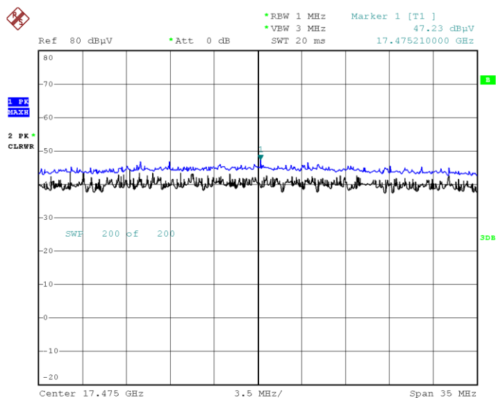
Peak Reading (802.11a, Ch.165 3rd Harmonic, Y-H)
