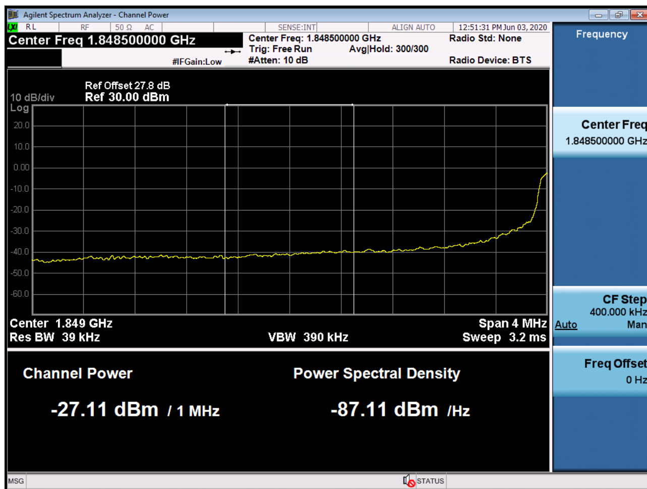
Sub6 n2. Lower Extended Band Edge Plot (20M BW Ch.372000 BPSK_RB100_0) -3
