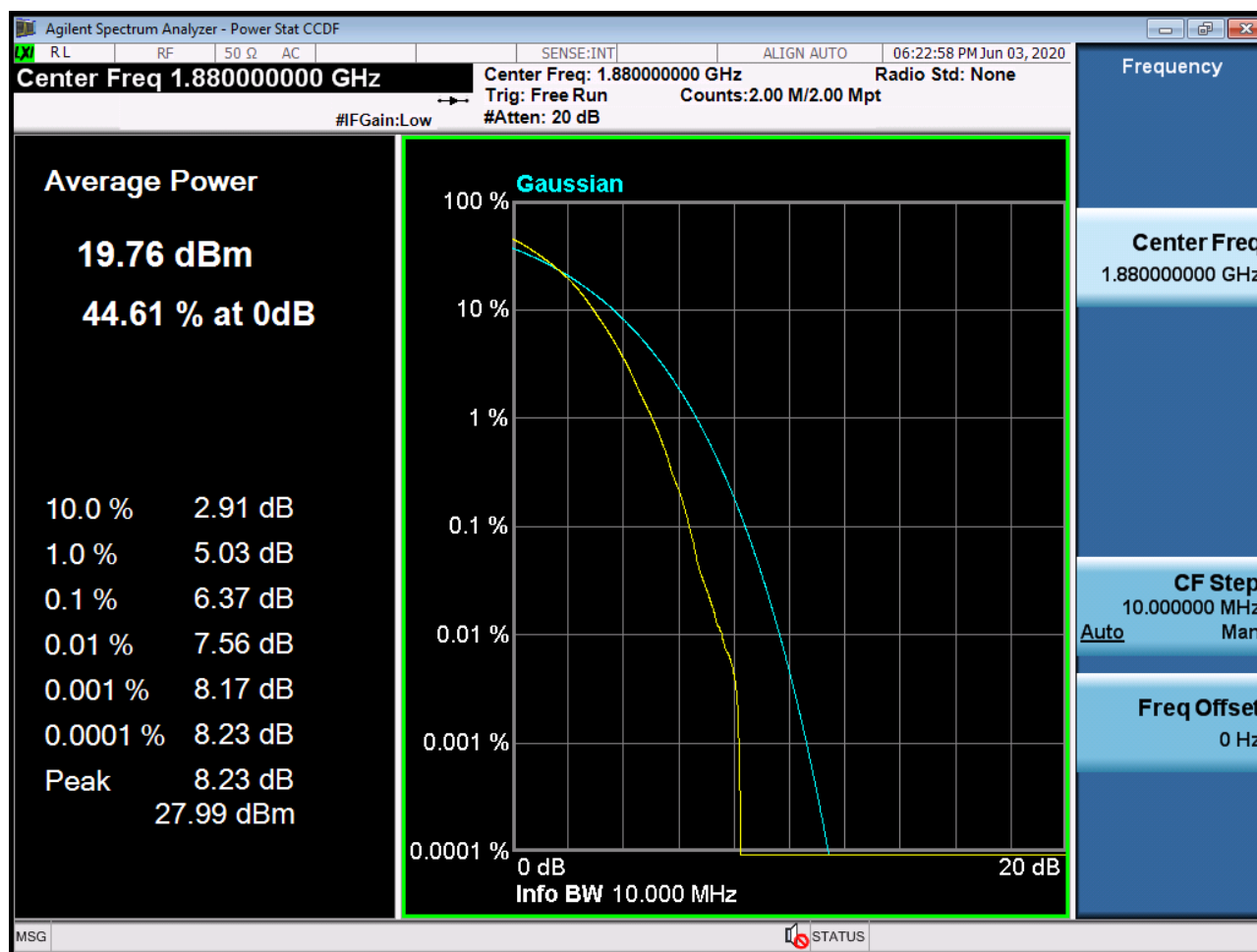
Sub6 n2. PAR Plot (10M BW Ch.376000 256QAM RB 50_0)
