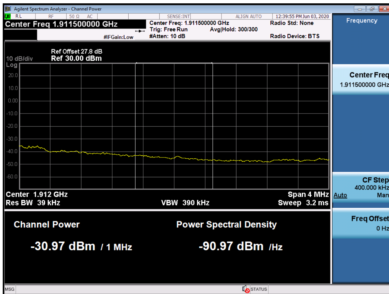
Sub6 n2. Upper Extended Band Edge Plot (15M BW Ch.380500 BPSK_RB75_0) -3
