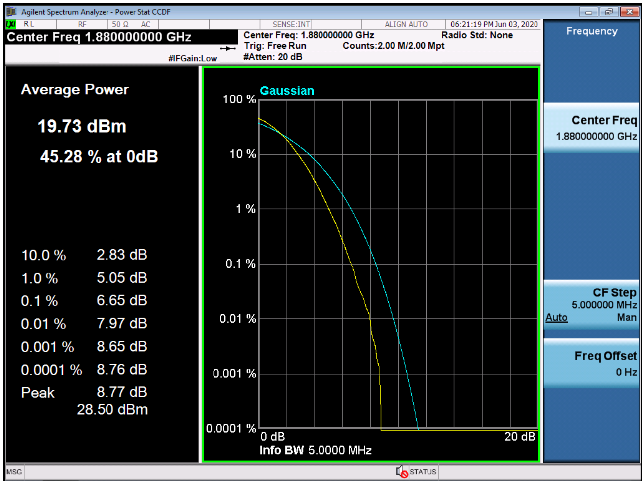
Sub6 n2. PAR Plot (5M BW Ch.376000 256QAM RB 25_0)
