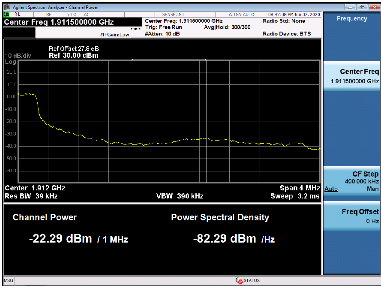
Sub6 n2. Upper Extended Band Edge Plot (5M BW Ch.381500 BPSK_RB25_0) -3
