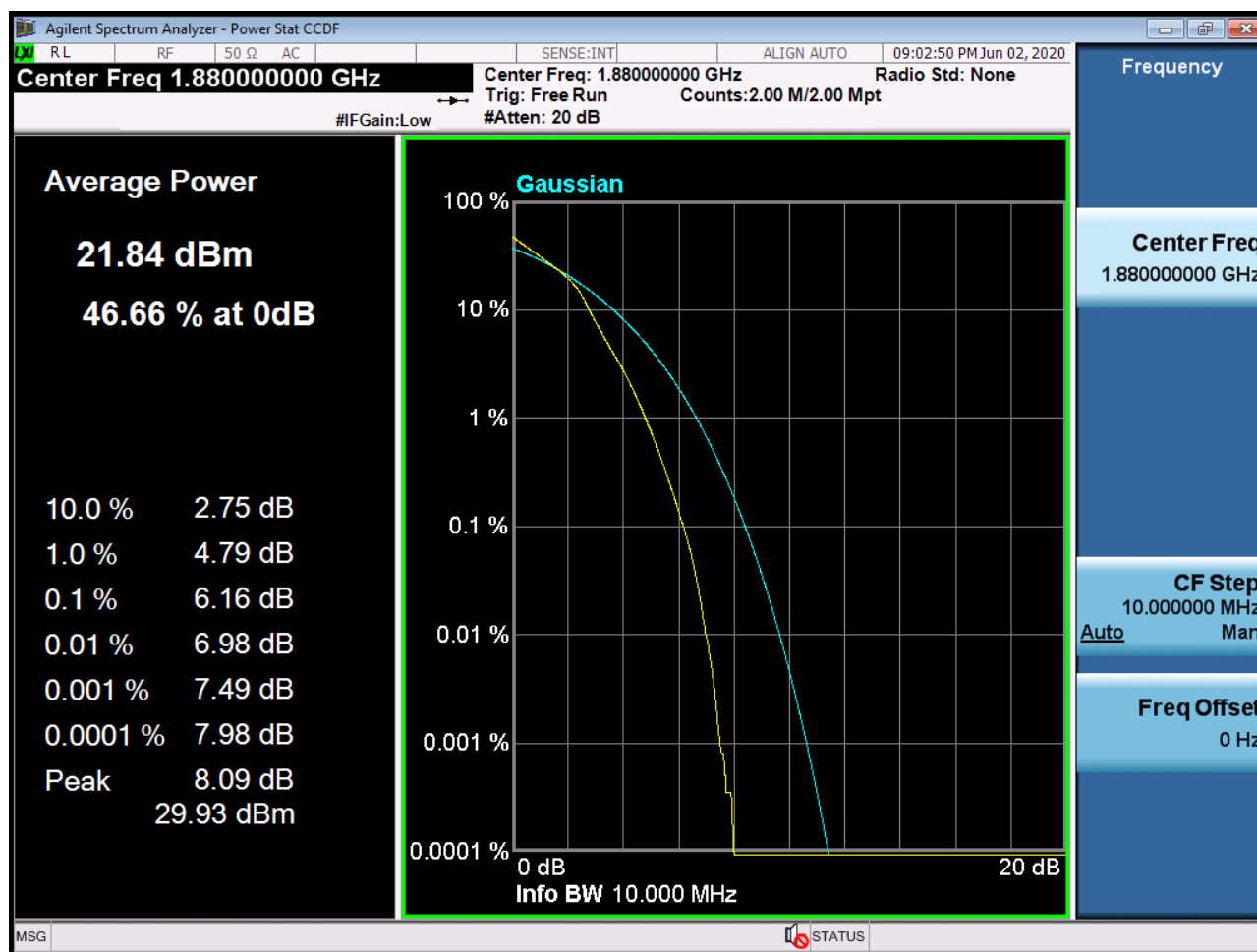
Sub6 n2. PAR Plot (10M BW Ch.376000 16QAM RB 50_0)
