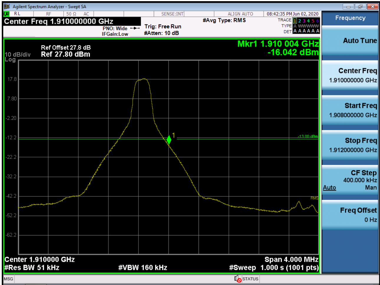
Sub6 n2. Upper Band Edge Plot (5M BW Ch.381500 BPSK_RB1_Offset 24) -1
