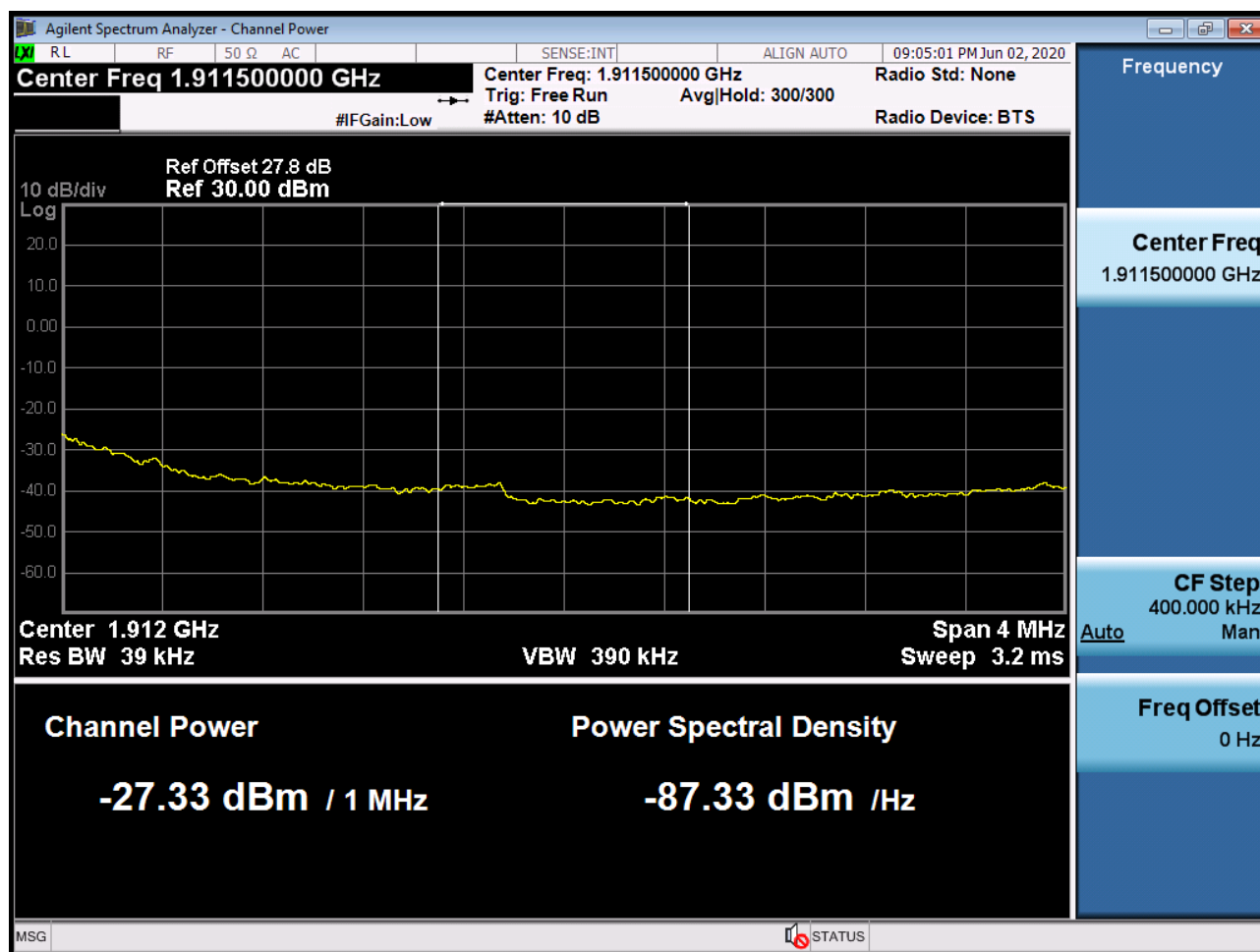
Sub6 n2. Upper Extended Band Edge Plot (10M BW Ch.381000 BPSK_RB50_0) -3
