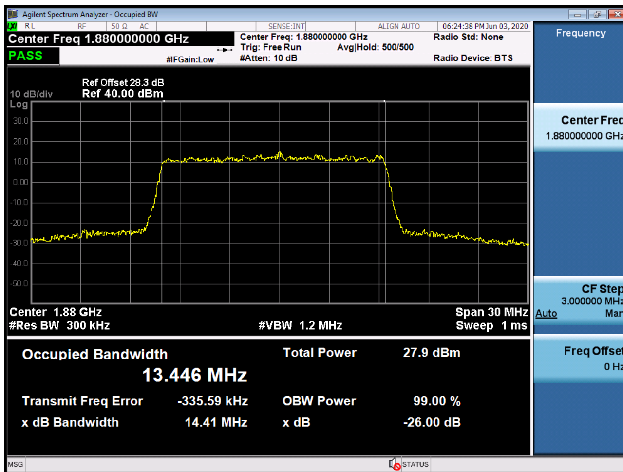
Sub6 n2. Occupied Bandwidth Plot (15M BW Ch.376000 256QAM RB 75_0)
