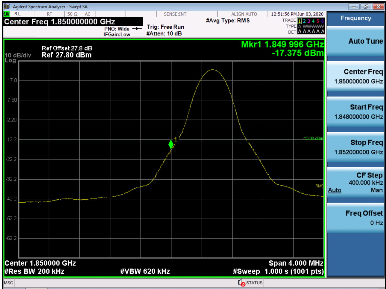
Sub6 n2. Lower Band Edge Plot (20M BW Ch.372000 BPSK_RB1_Offset 0) -1
