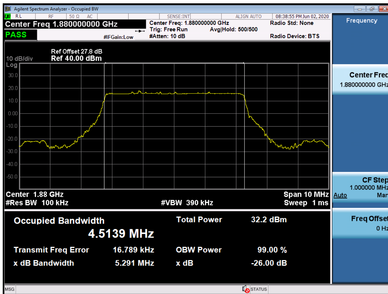
Sub6 n2. Occupied Bandwidth Plot (5M BW Ch.376000 BPSK RB 25_0)
