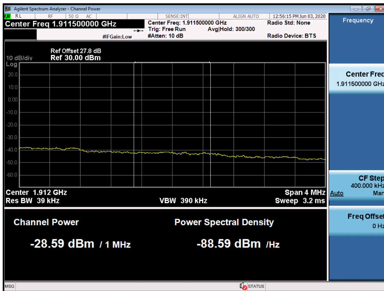
Sub6 n2. Upper Extended Band Edge Plot (20M BW Ch.380000 BPSK_RB100_0) -3
