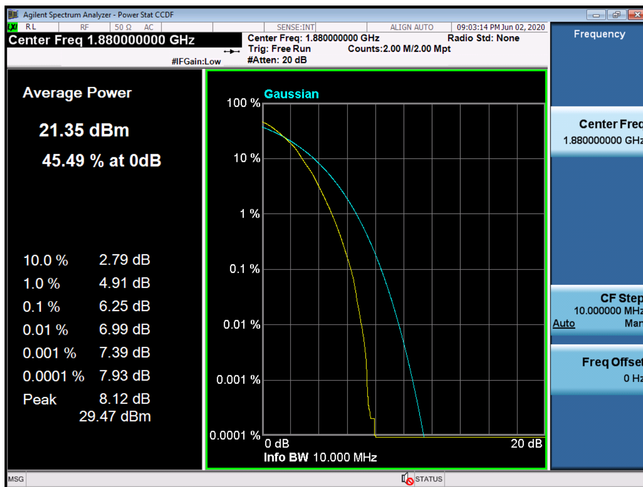
Sub6 n2. PAR Plot (10M BW Ch.376000 64QAM RB 50_0)
