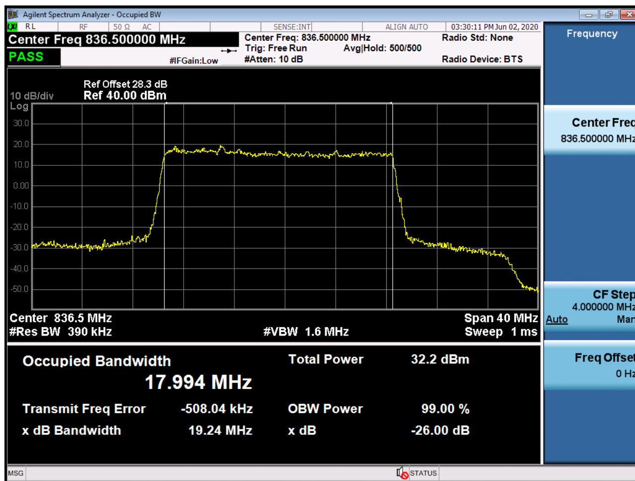
Sub6 n5. Occupied Bandwidth Plot (20M BW Ch.167300 BPSK_RB50_0)
