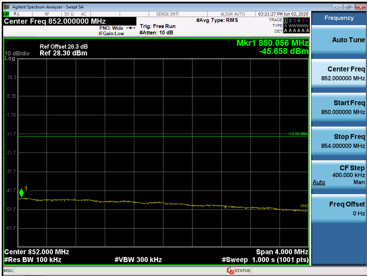
Sub6 n5. Upper Extended Band Edge Plot (15M BW Ch.168300 BPSK_RB25_0)
