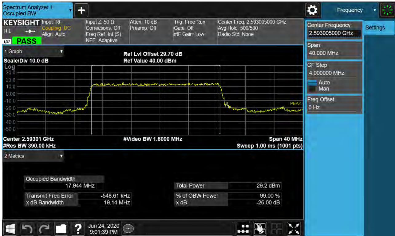
Sub6 n41. Occupied Bandwidth Plot (20 MHz Ch.518601 BPSK RB 25) _SCS 15 kHz
