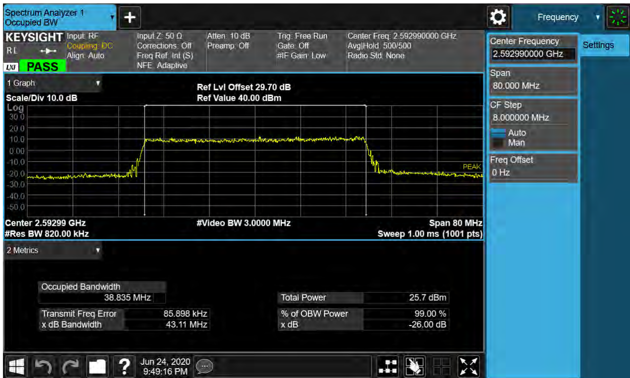
Sub6 n41. Occupied Bandwidth Plot (40 MHz Ch.518601 256-QAM RB 25) _SCS 15 kHz
