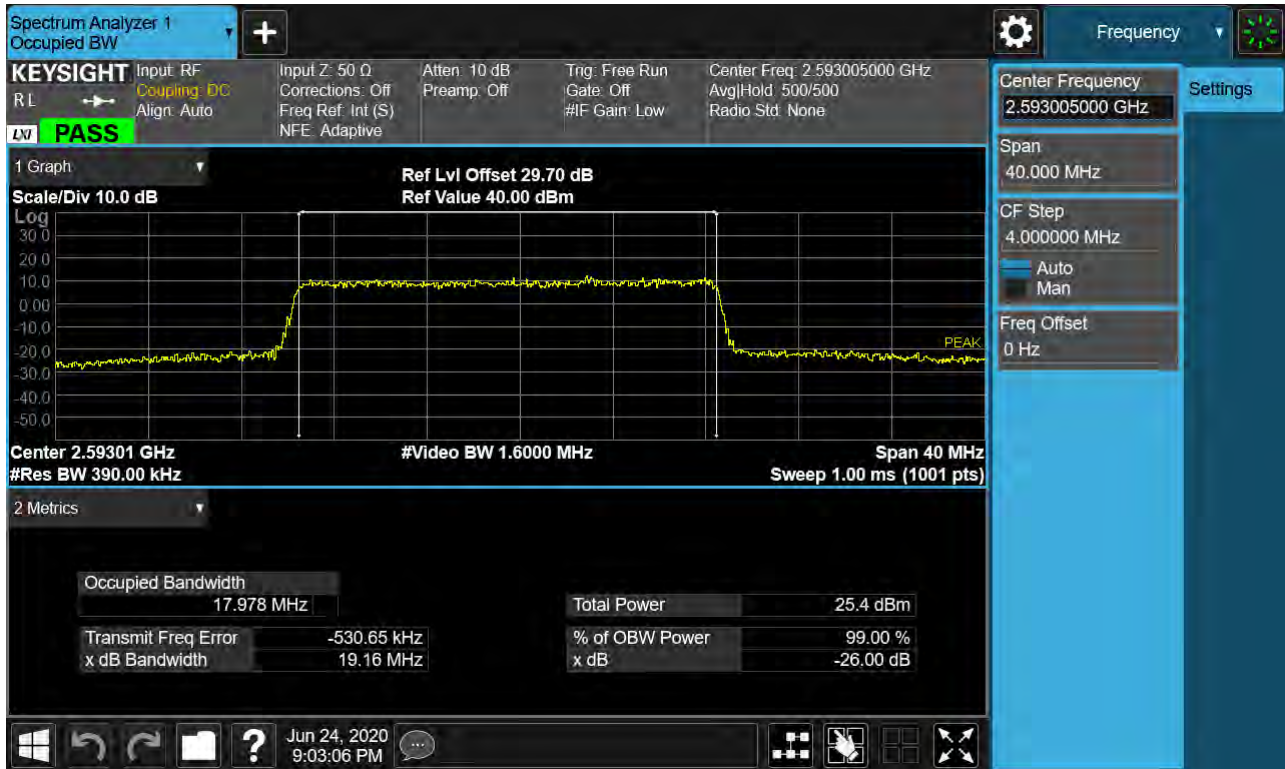
Sub6 n41. Occupied Bandwidth Plot (20 MHz Ch.518601 256-QAM RB 25) _SCS 15 kHz
