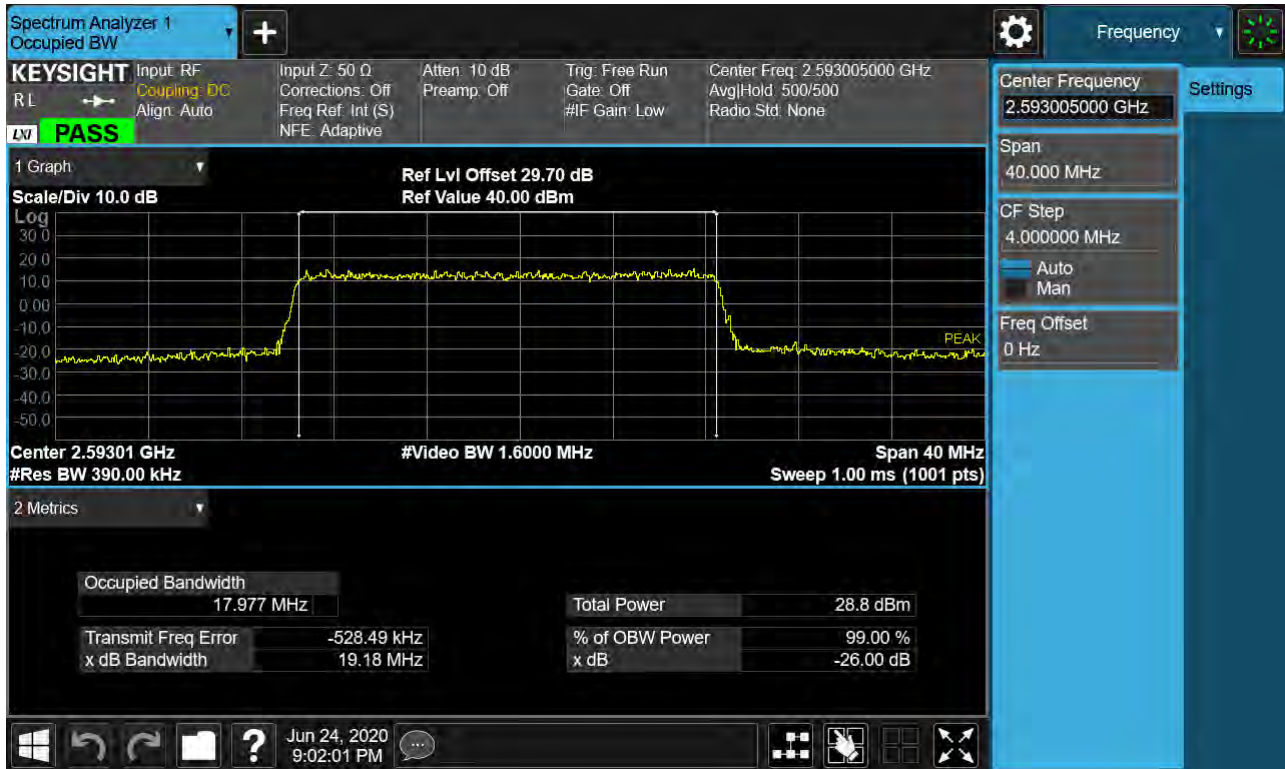
Sub6 n41. Occupied Bandwidth Plot (20 MHz Ch.518601 QPSK RB 25) _SCS 15 kHz
