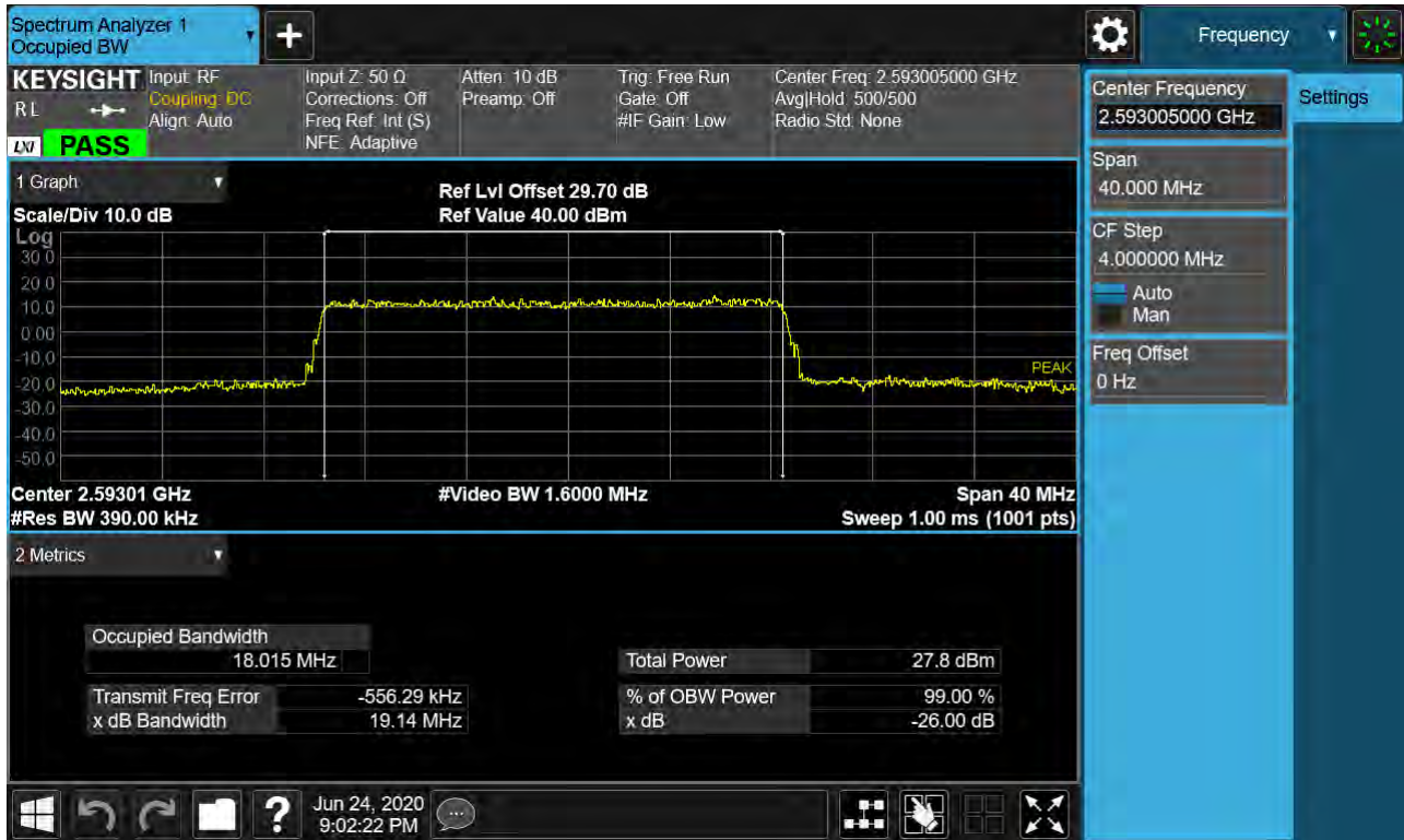
Sub6 n41. Occupied Bandwidth Plot (20 MHz Ch.518601 16-QAM RB 25)_SCS 15 kHz
