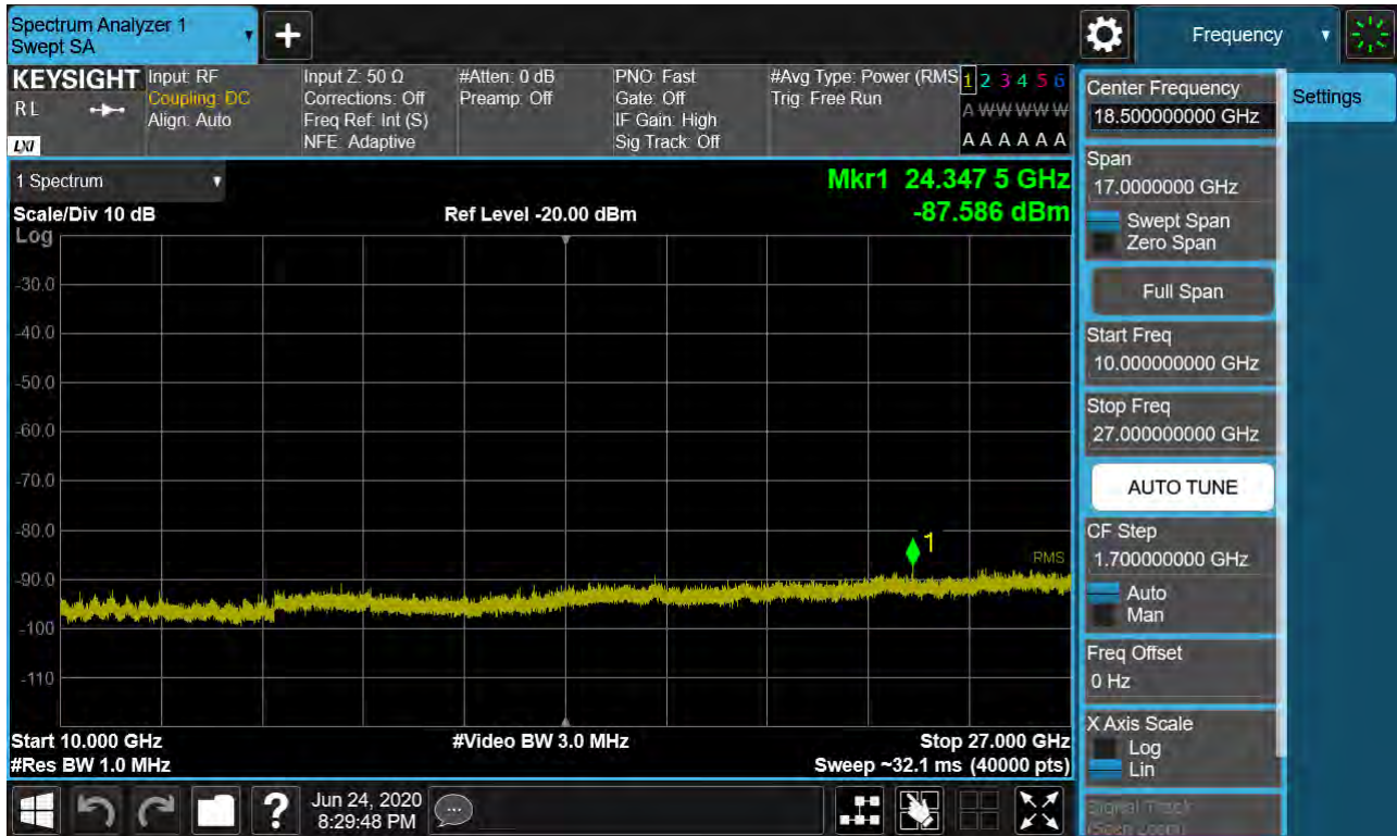
Sub6 n41. Conducted Spurious Plot 2 (50 MHz Ch.532998 BPSK RB 1, Offset 0)
