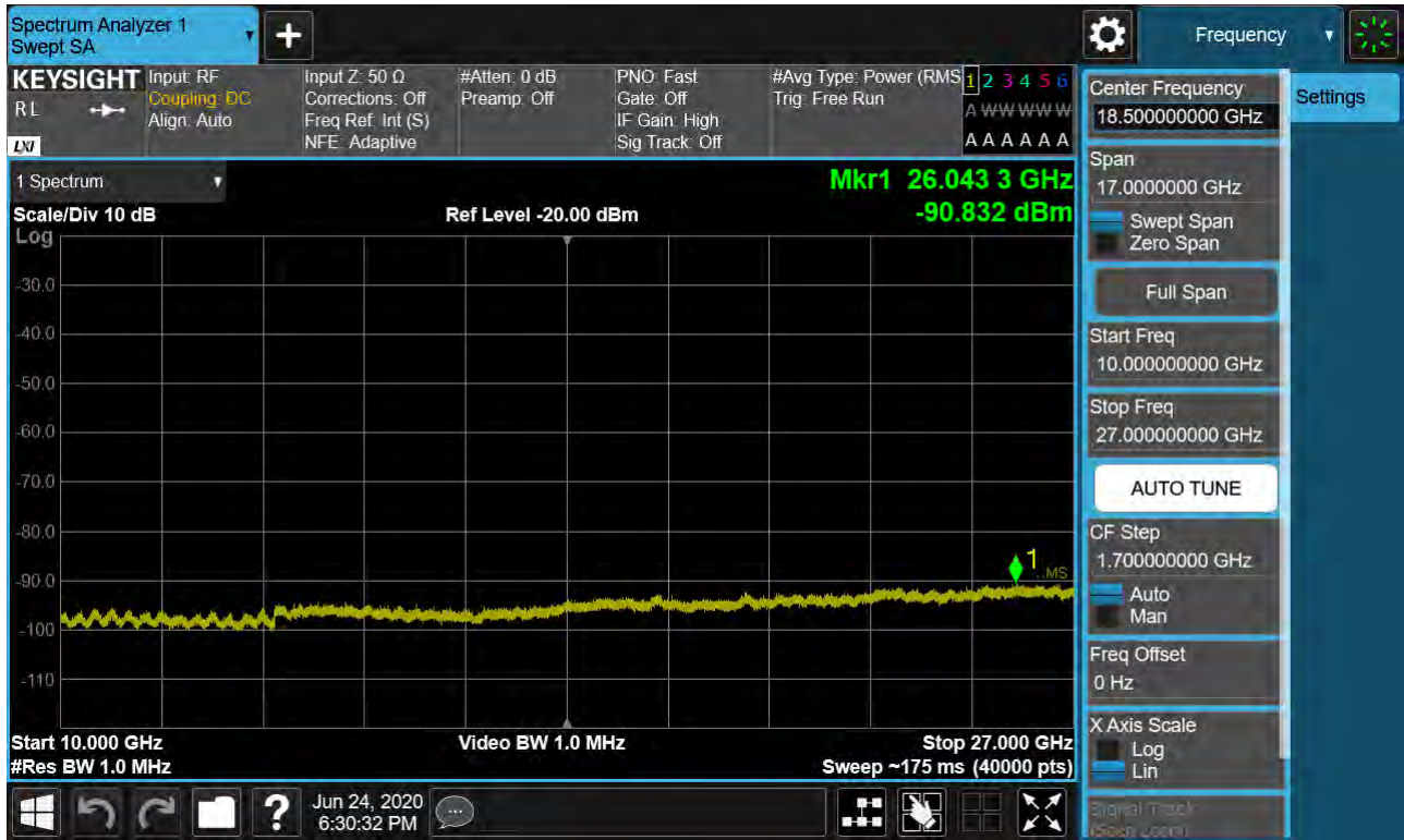
Sub6 n41. Conducted Spurious Plot 2 (90 MHz Ch.508200 BPSK RB 1, Offset 0)
