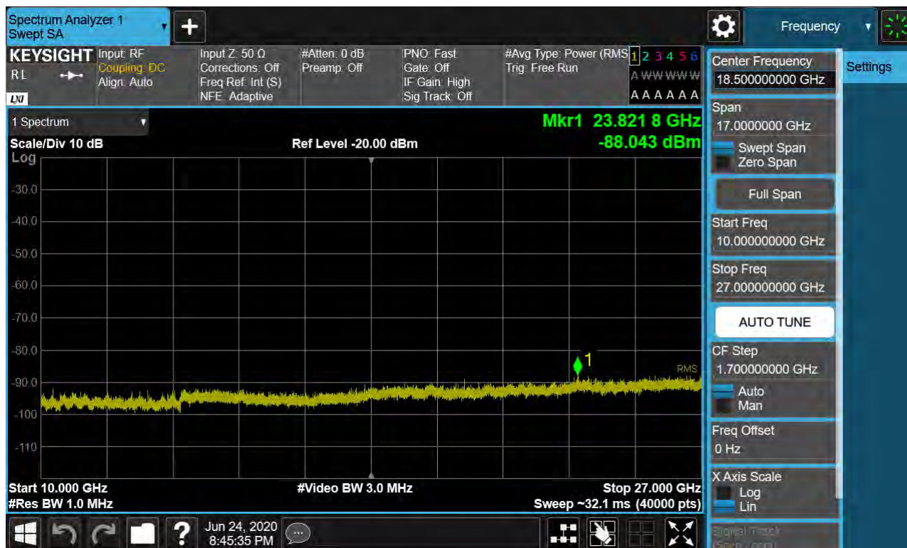
Sub6 n41. Conducted Spurious Plot 2 (60 MHz Ch. 518598 BPSK RB 1, Offset 0)
