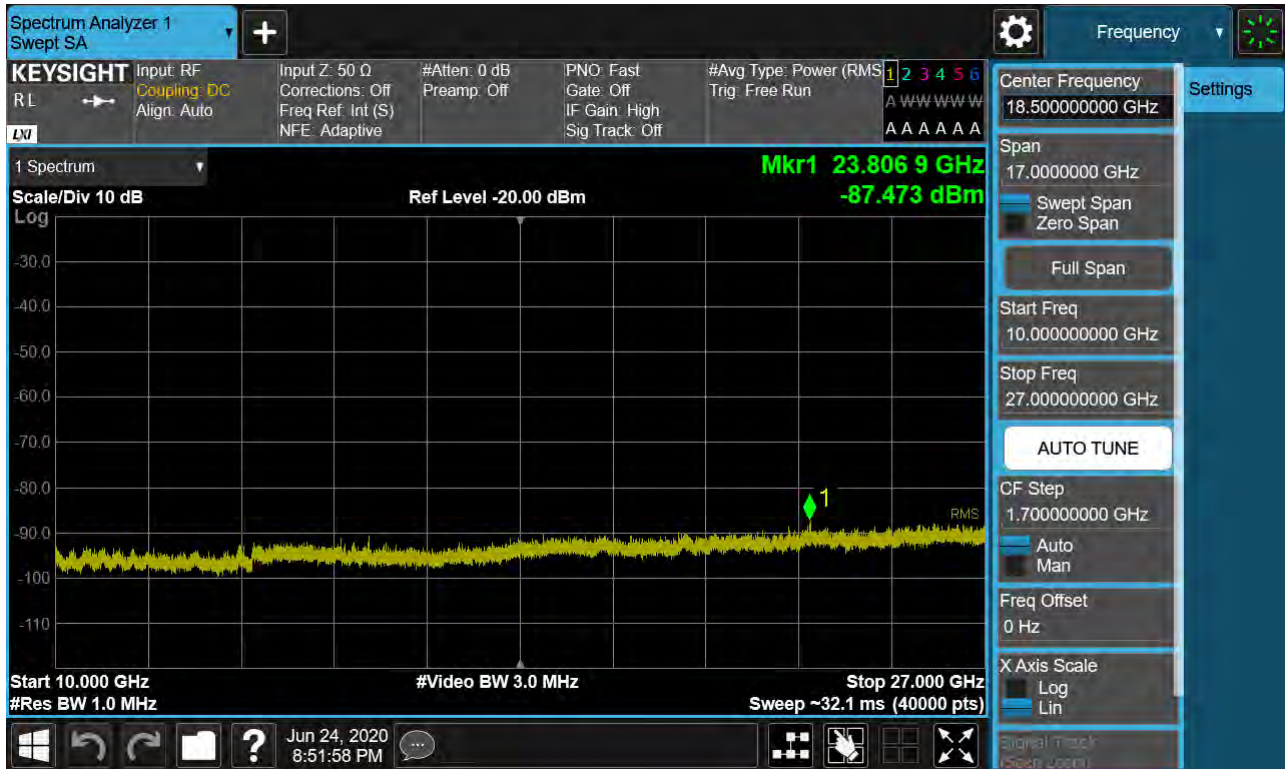
Sub6 n41. Conducted Spurious Plot 2 (60 MHz Ch.531996 BPSK RB 1, Offset 0)
