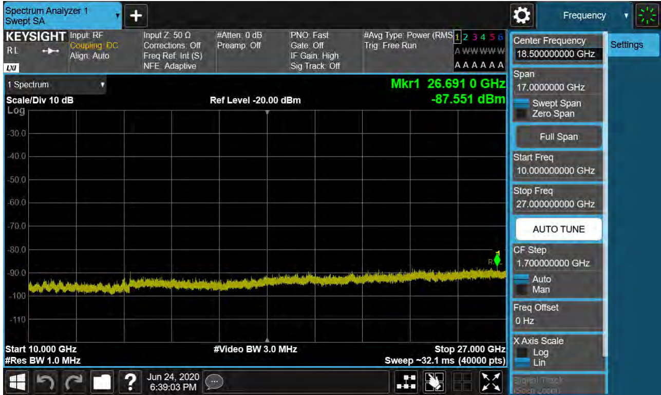
Sub6 n41. Conducted Spurious Plot 2 (90 MHz Ch. 518598 BPSK RB 1, Offset 0)
