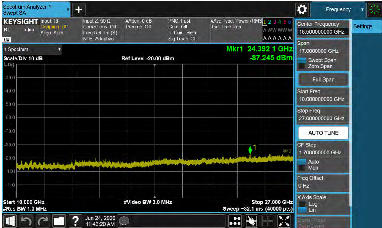
Sub6 n41. Conducted Spurious Plot 2 (100 MHz Ch.509202 BPSK RB 1, Offset 0)
