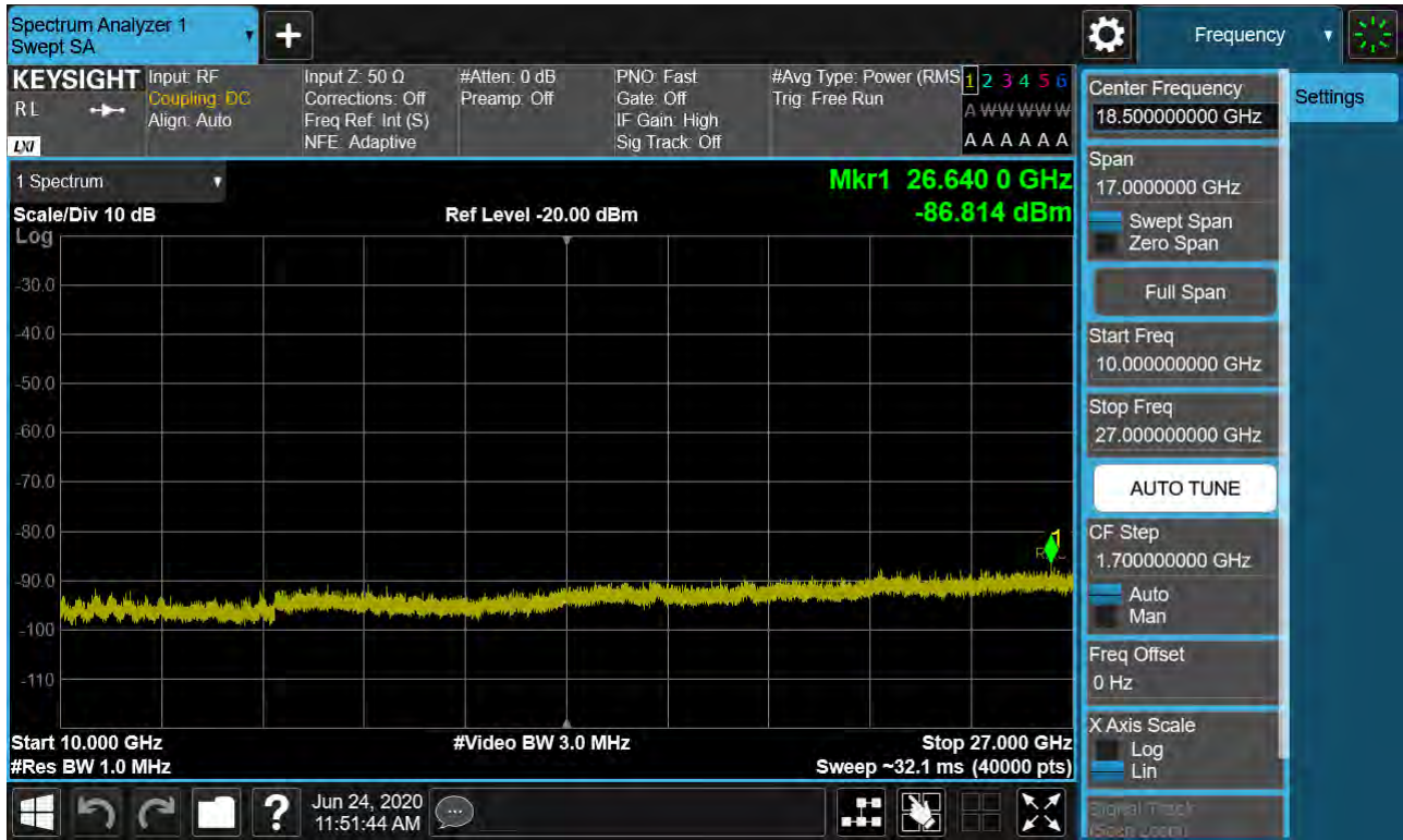
Sub6 n41. Conducted Spurious Plot 2 (100 MHz Ch. 518598 BPSK RB 1, Offset 0)
