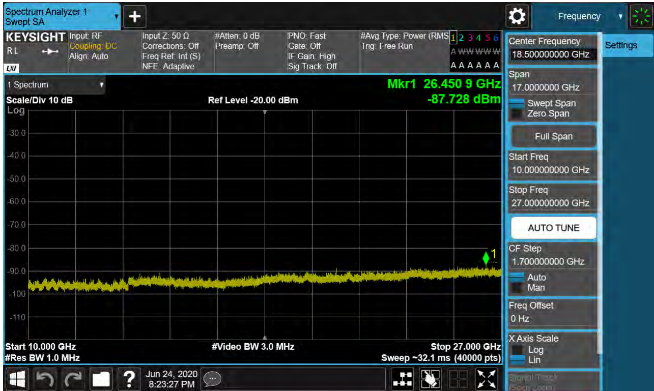
Sub6 n41. Conducted Spurious Plot 2 (50 MHz Ch. 518598 BPSK RB 1, Offset 0)
