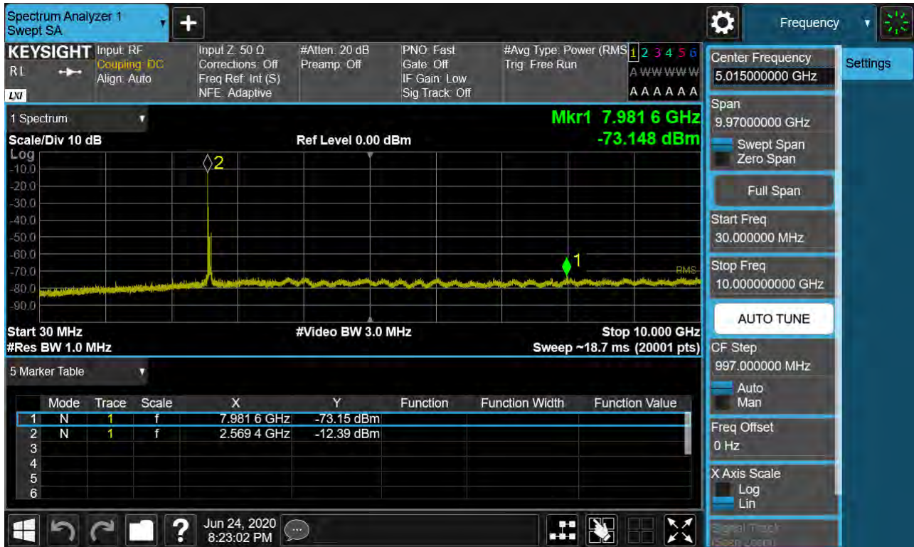
Sub6 n41. Conducted Spurious Plot 1 (50 MHz Ch.518598 BPSK RB 1, Offset 0)
