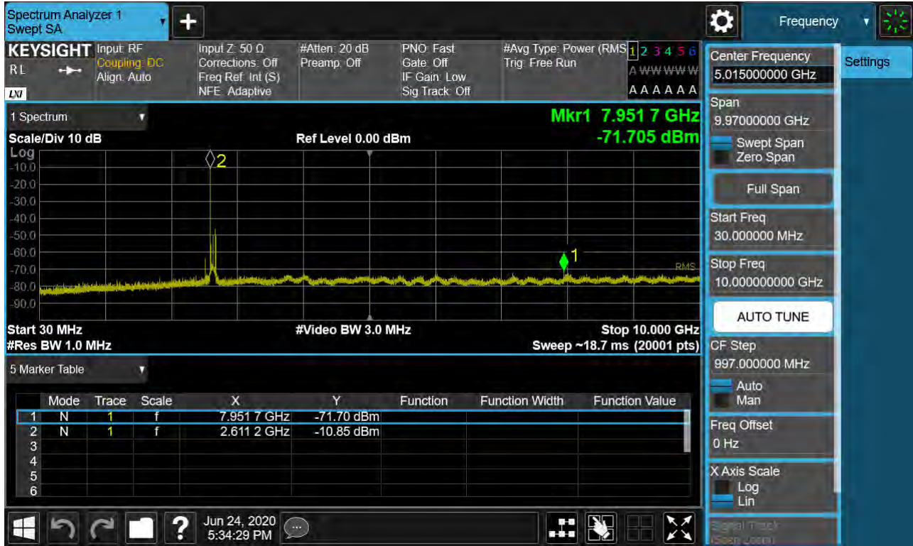
Sub6 n41. Conducted Spurious Plot 1 (80 MHz Ch.529998 BPSK RB 1, Offset 0)
