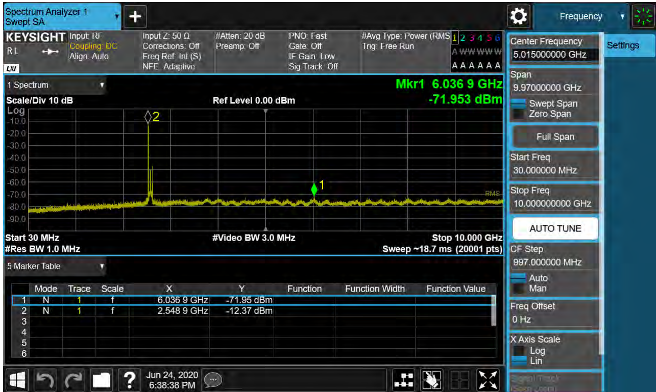
Sub6 n41. Conducted Spurious Plot 1 (90 MHz Ch.518598 BPSK RB 1, Offset 0)
