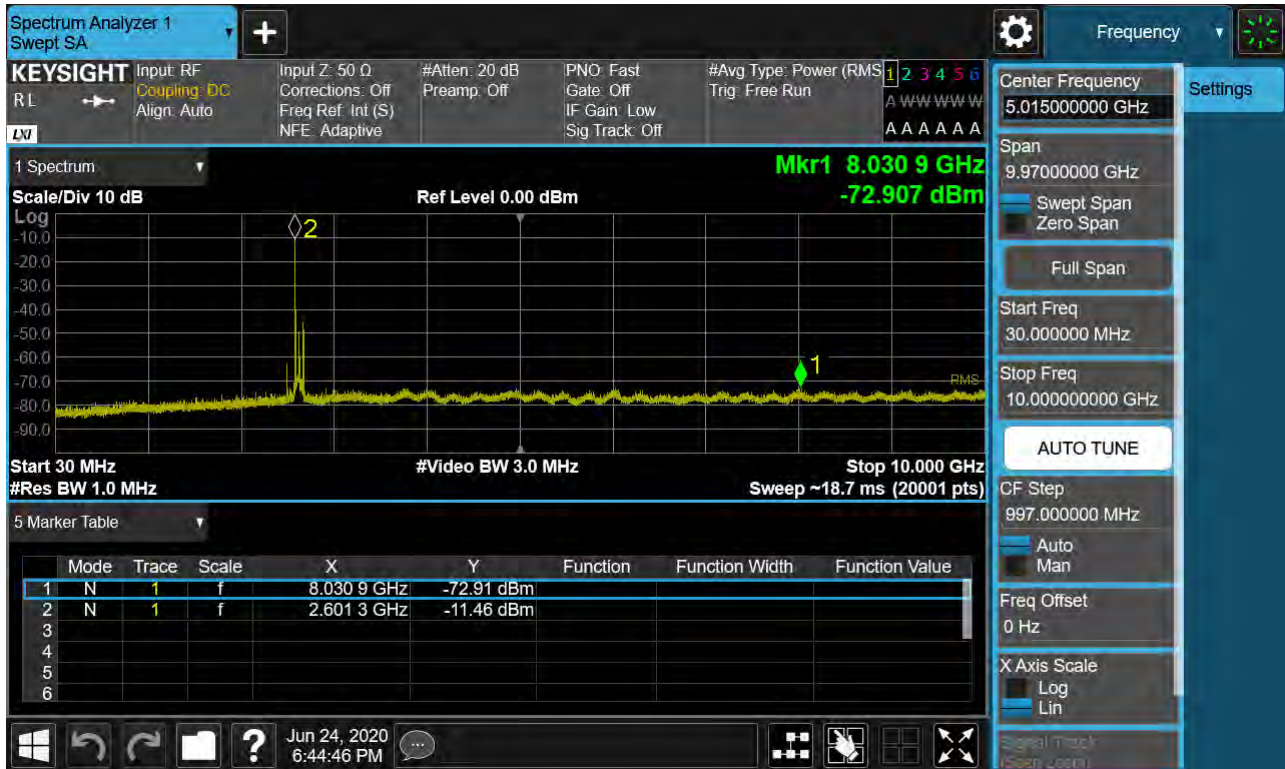
Sub6 n41. Conducted Spurious Plot 1 (90 MHz Ch.528996 BPSK RB 1, Offset 0)
