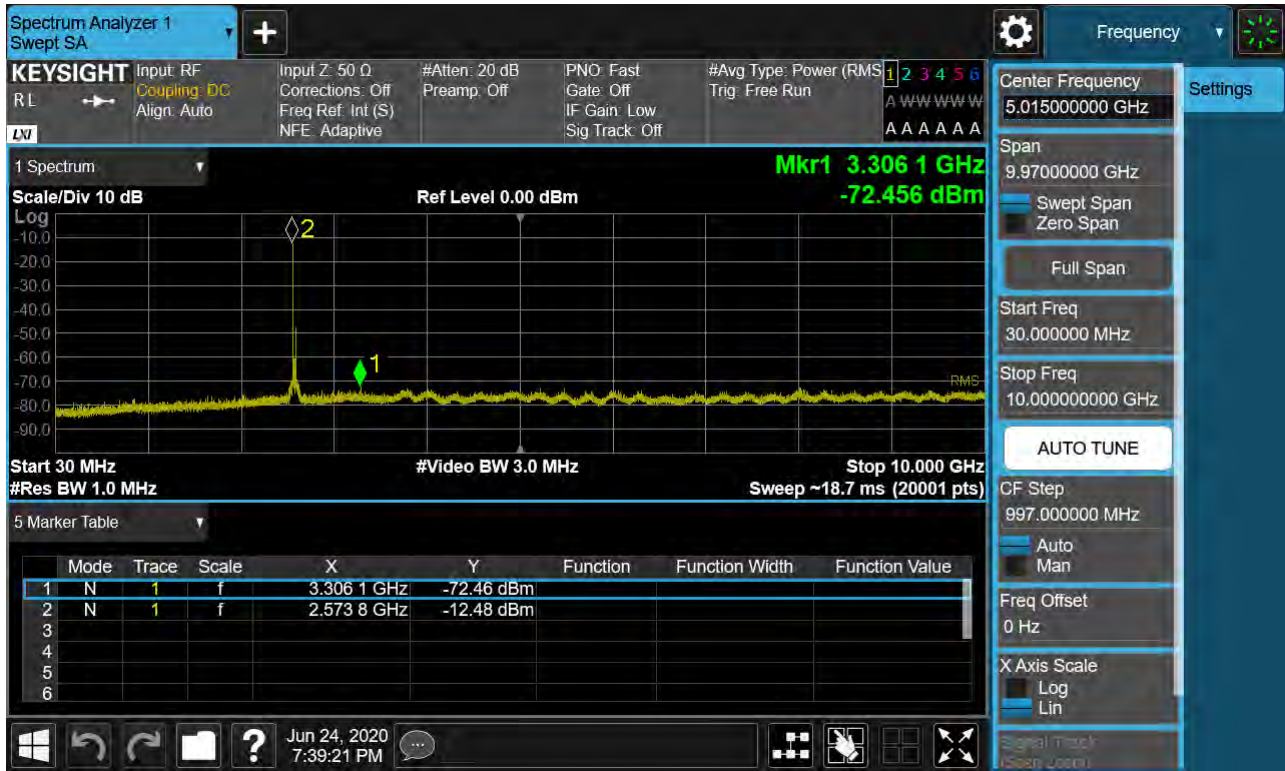
Sub6 n41. Conducted Spurious Plot 1 (40 MHz Ch.518598 BPSK RB 1, Offset 0)
