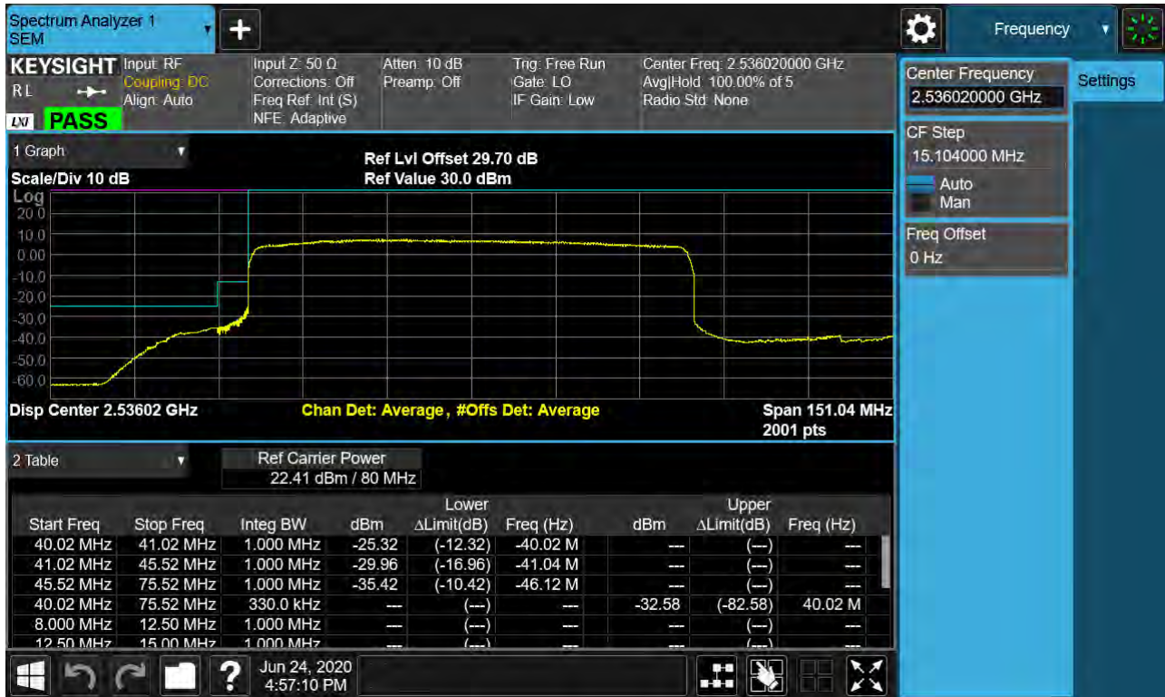
Sub6 n41. Low Channel Edge Plot (80 MHz Ch.507204 BPSK RB 25, Offset 0)-1
