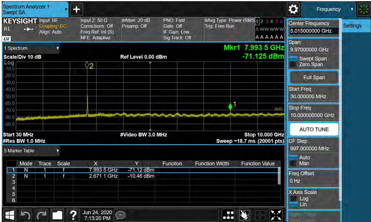
Sub6 n41. Conducted Spurious Plot 1 (20 MHz Ch.535998 BPSK RB 1, Offset 0)
