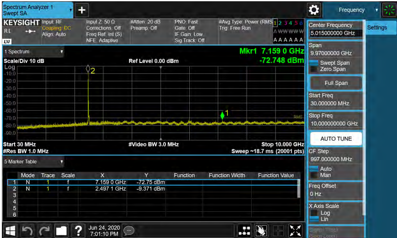
Sub6 n41. Conducted Spurious Plot 1 (20 MHz Ch.501204 BPSK RB 1, Offset 0)
