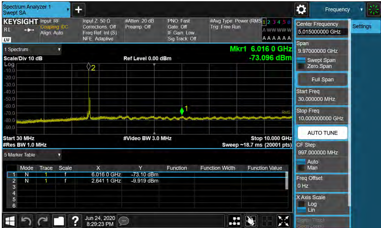
Sub6 n41. Conducted Spurious Plot 1 (50 MHz Ch.532998 BPSK RB 1, Offset 0)
