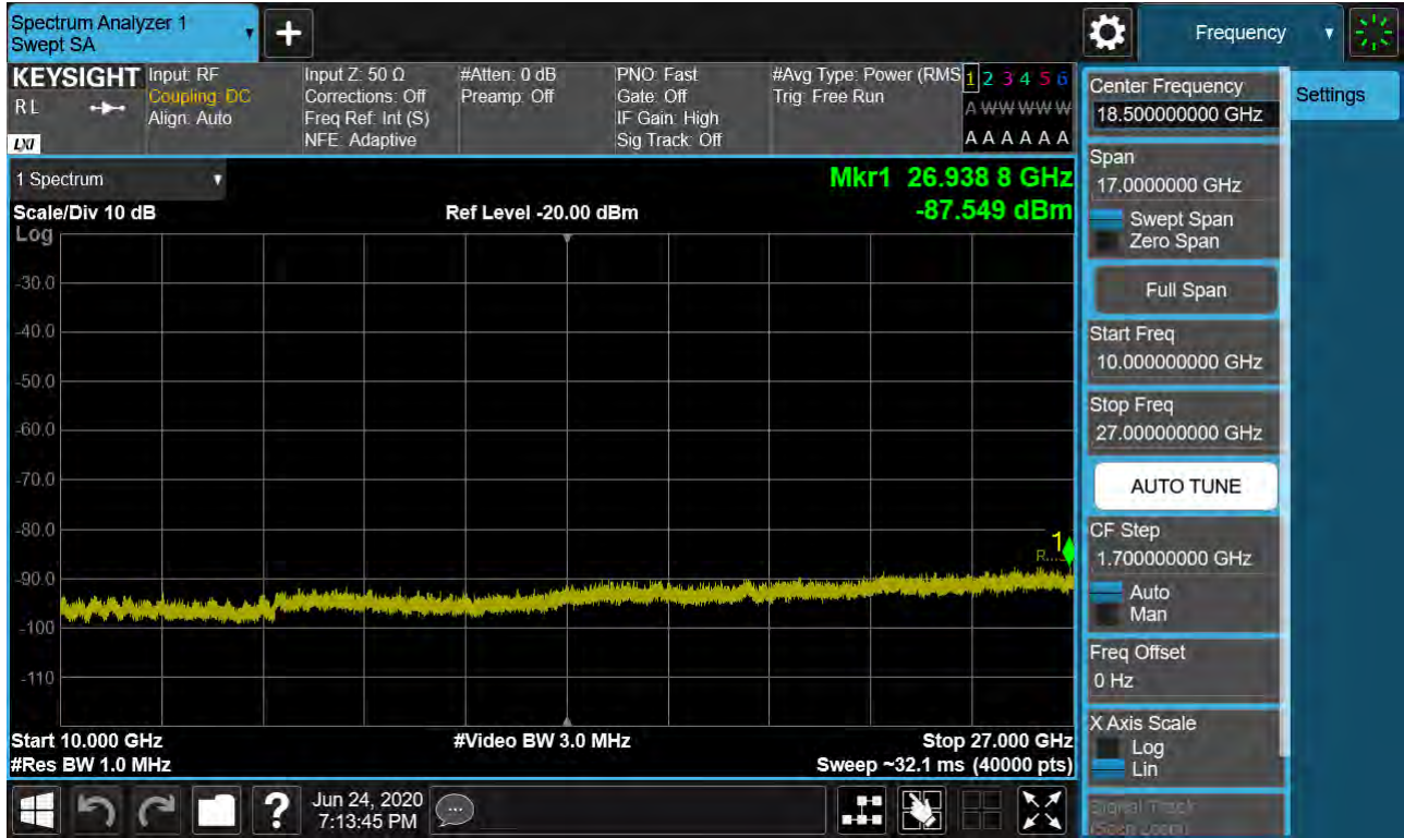
Sub6 n41. Conducted Spurious Plot 2 (20 MHz Ch.535998 BPSK RB 1, Offset 0)
