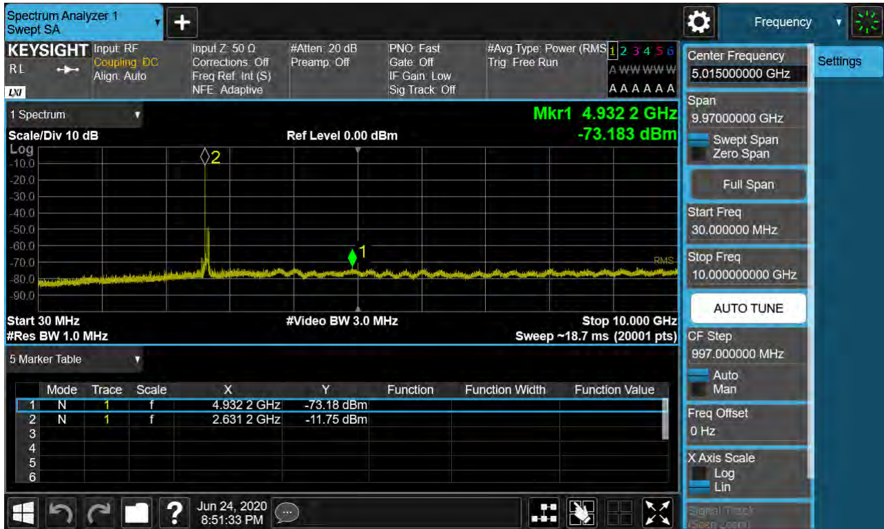
Sub6 n41. Conducted Spurious Plot 1 (60 MHz Ch.531996 BPSK RB 1, Offset 0)
