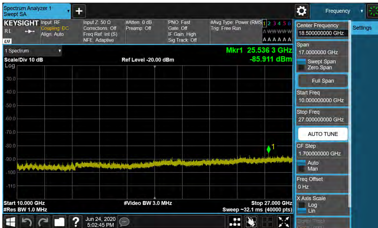
Sub6 n41. Conducted Spurious Plot 2 (80 MHz Ch.507204 BPSK RB 1, Offset 0)
