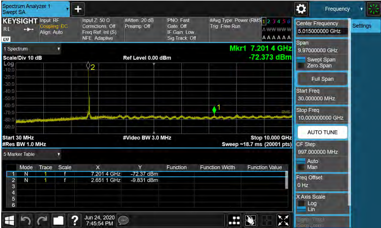
Sub6 n41. Conducted Spurious Plot 1 (40 MHz Ch.534000 BPSK RB 1, Offset 0)
