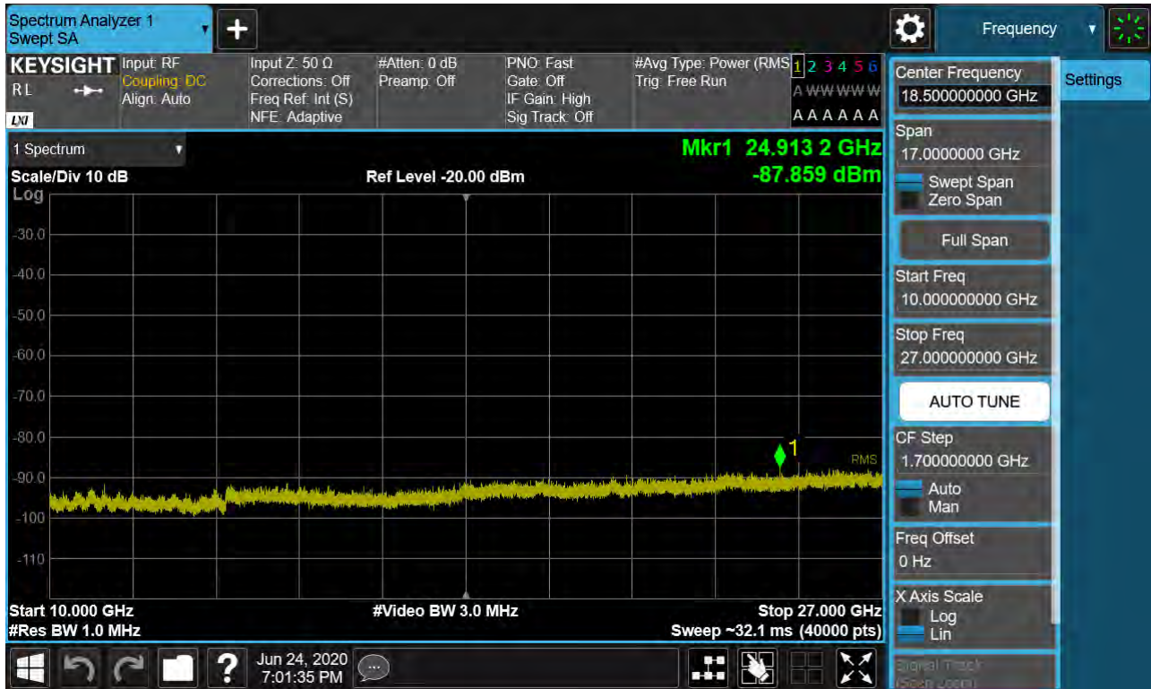
Sub6 n41. Conducted Spurious Plot 2 (20 MHz Ch.501204 BPSK RB 1, Offset 0)
