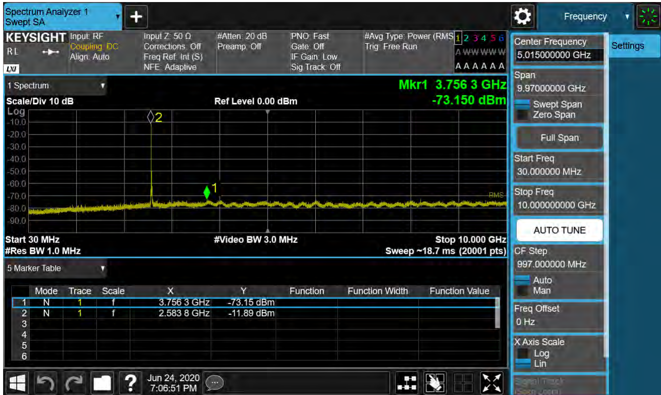
Sub6 n41. Conducted Spurious Plot 1 (20 MHz Ch.518598 BPSK RB 1, Offset 0)
