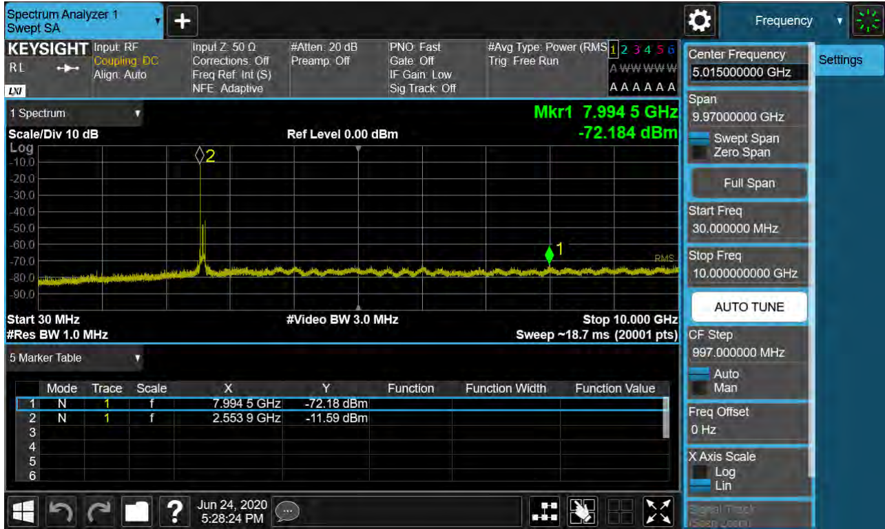
Sub6 n41. Conducted Spurious Plot 1 (80 MHz Ch.518598 BPSK RB 1, Offset 0)
