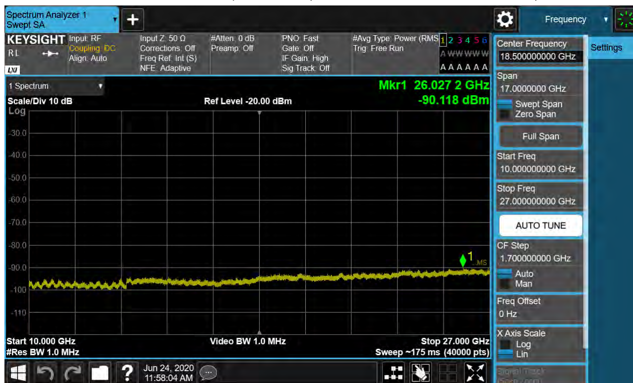
Sub6 n41. Conducted Spurious Plot 2 (100 MHz Ch.528000 BPSK RB 1, Offset 0)
