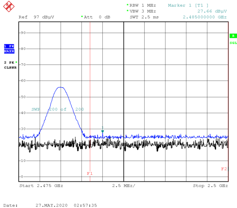
Radiated Band Edges plot – Ch.78
