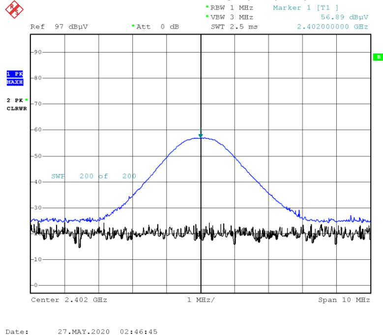
Fundamental Field Strength plot (Ch.0)
