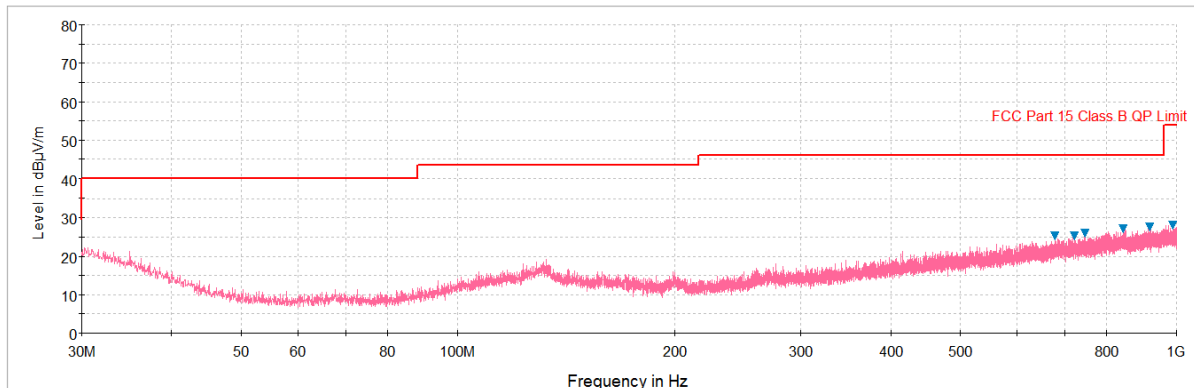
Plot 7-52. Radiated Spurious Plot below 1GHz (Pol. H)
