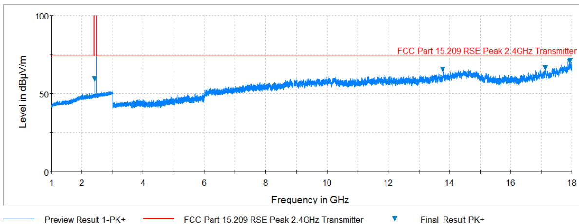
Plot 7-47. Radiated Spurious Plot above 1GHz (BT – Ch. 78, Ant. Pol. V)
