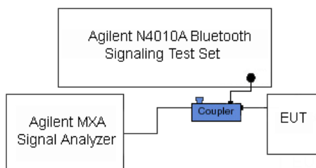
Figure 7-7. Test Instrument & Measurement Setup
