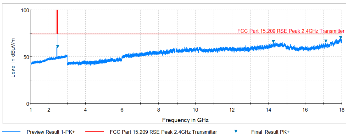
Plot 7-46. Radiated Spurious Plot above 1GHz (BT – Ch. 78, Ant. Pol. H)
