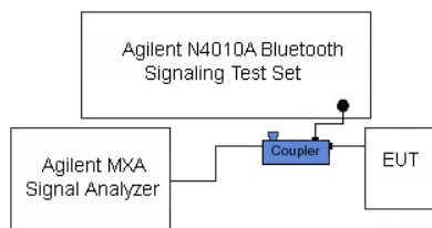
Figure 7-3. Test Instrument & Measurement Setup
