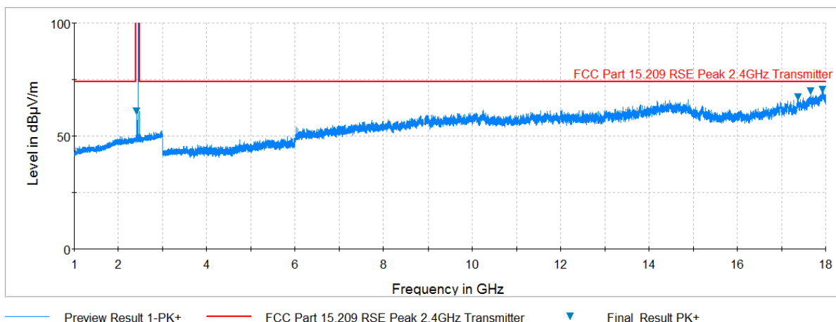
Plot 7-45. Radiated Spurious Plot above 1GHz (BT – Ch. 39, Ant. Pol. V)
