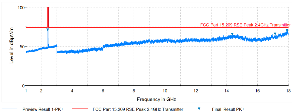
Plot 7-44. Radiated Spurious Plot above 1GHz (BT – Ch. 39, Ant. Pol. H)
