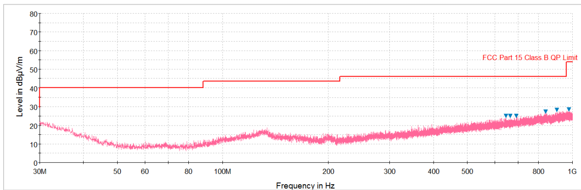
Plot 7-53. Radiated Spurious Plot below 1GHz (Pol. V)
