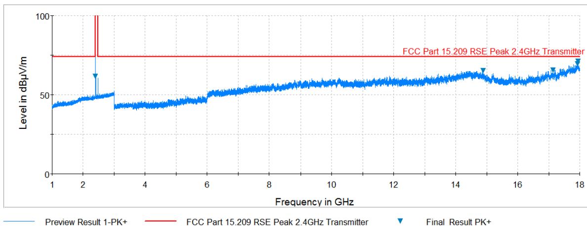
Plot 7-43. Radiated Spurious Plot above 1GHz (BT – Ch. 0, Ant. Pol. V)
