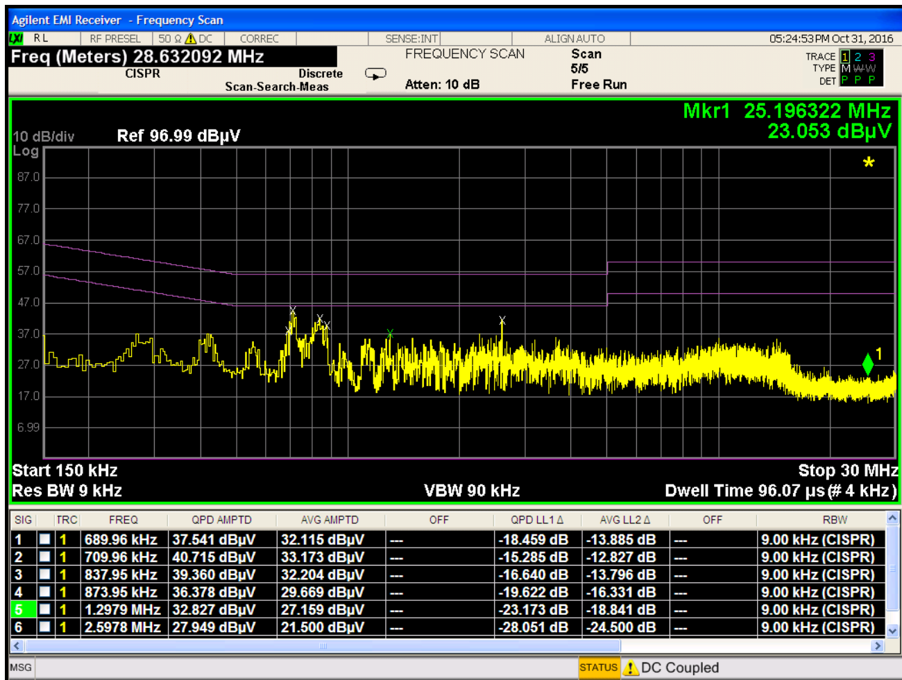
Plot 7-6. Line-Conducted Test Plot (L1)
