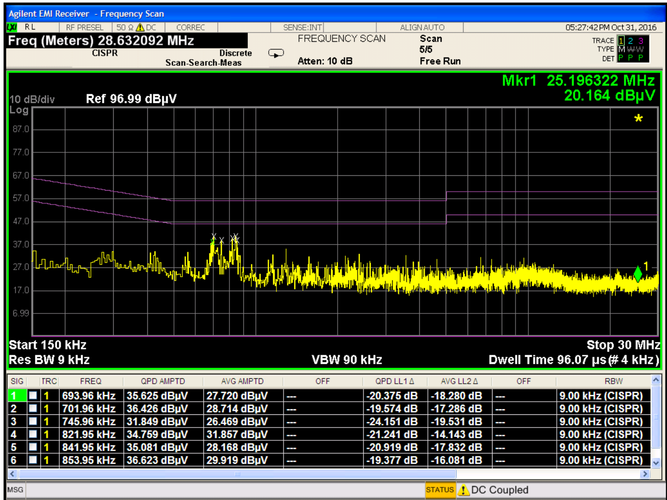
Plot 7-7. Line-Conducted Test Plot (N)
