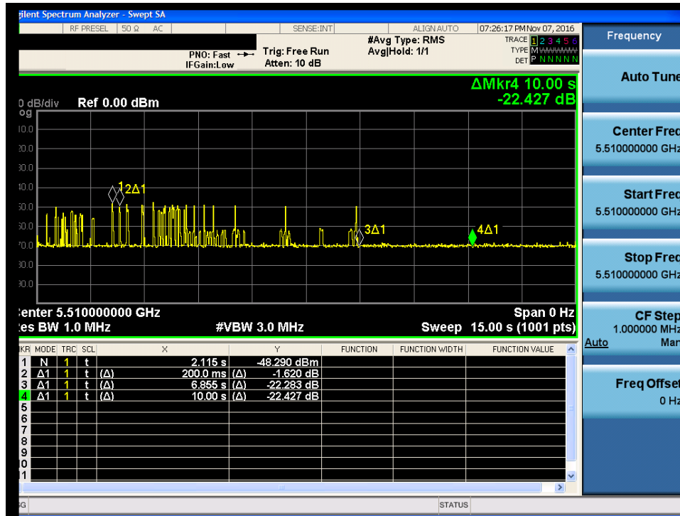
Figure 5-6. Band 2C Move Time
