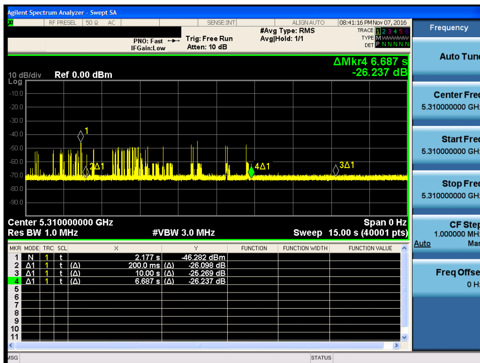
Figure 5-5. Band 2A Move Time
