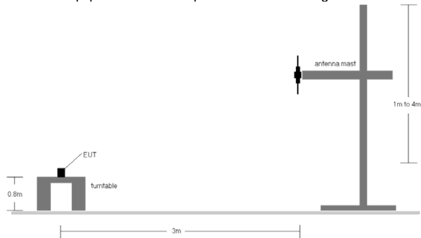
Figure 7-5. Radiated Test Setup <1GHz
