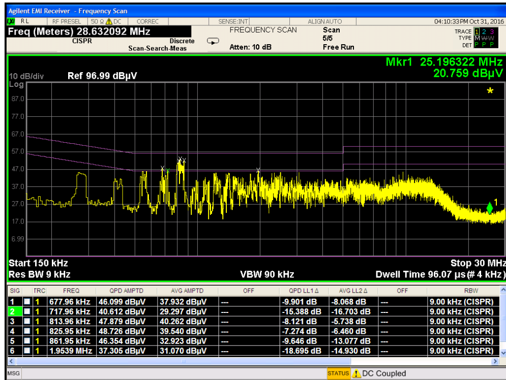
Plot 7-53. Line Conducted Plot with 802.11b (L1)
