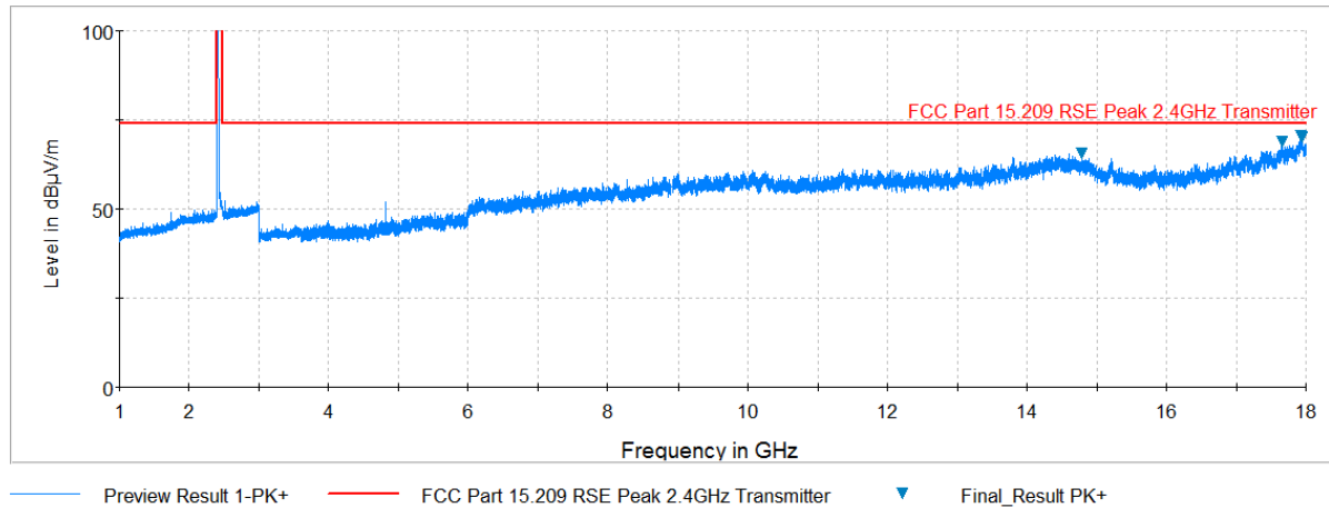
Plot 7-35. Radiated Spurious Plot above 1GHz (802.11b – Ch. 1, Ant. Pol. H)
