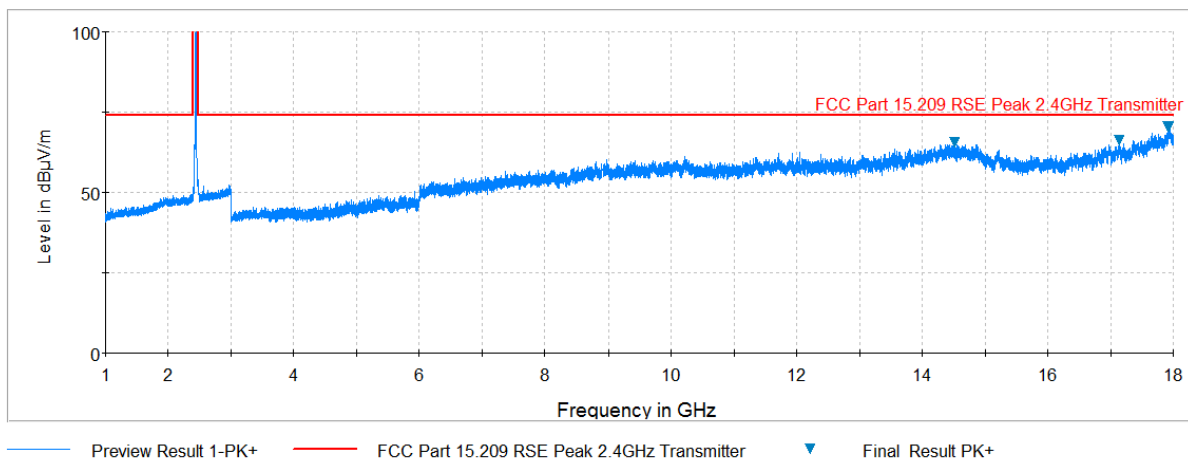
Plot 7-37. Radiated Spurious Plot above 1GHz (802.11b – Ch. 6, Ant. Pol. H)
