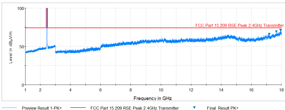
Plot 7-38. Radiated Spurious Plot above 1GHz (802.11b – Ch. 6, Ant. Pol. V)
