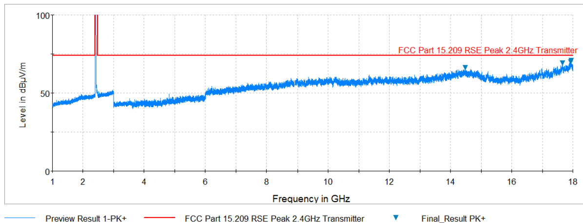
Plot 7-36. Radiated Spurious Plot above 1GHz (802.11b – Ch. 1, Ant. Pol. V)
