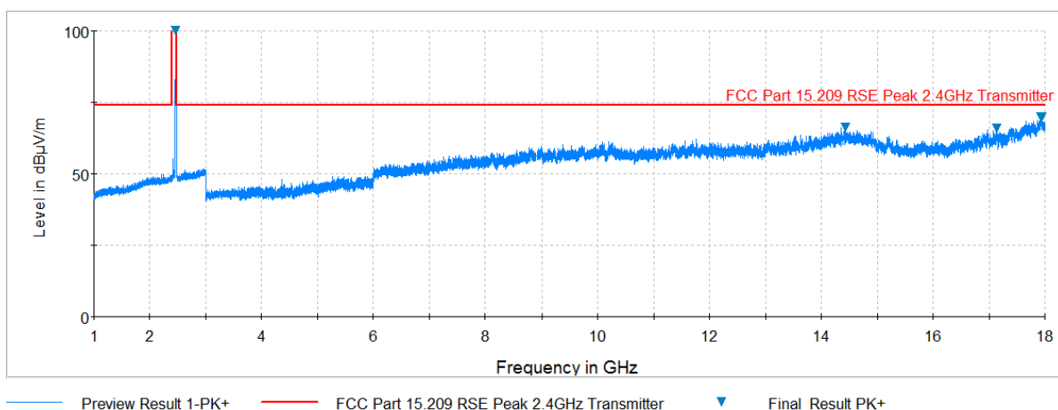
Plot 7-39. Radiated Spurious Plot above 1GHz (802.11b – Ch. 11, Ant. Pol. H)
