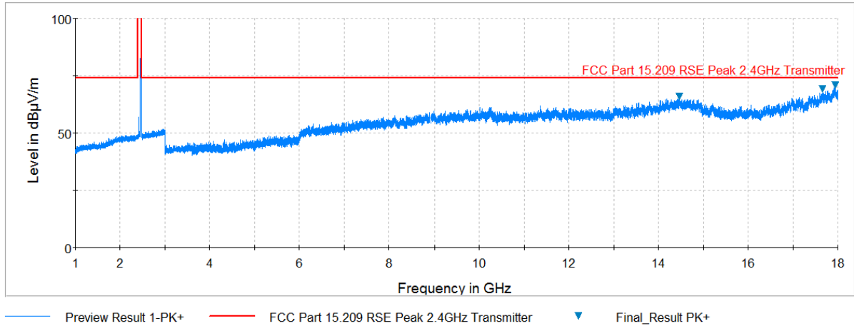
Plot 7-40. Radiated Spurious Plot above 1GHz (802.11b – Ch. 11, Ant. Pol. V)
