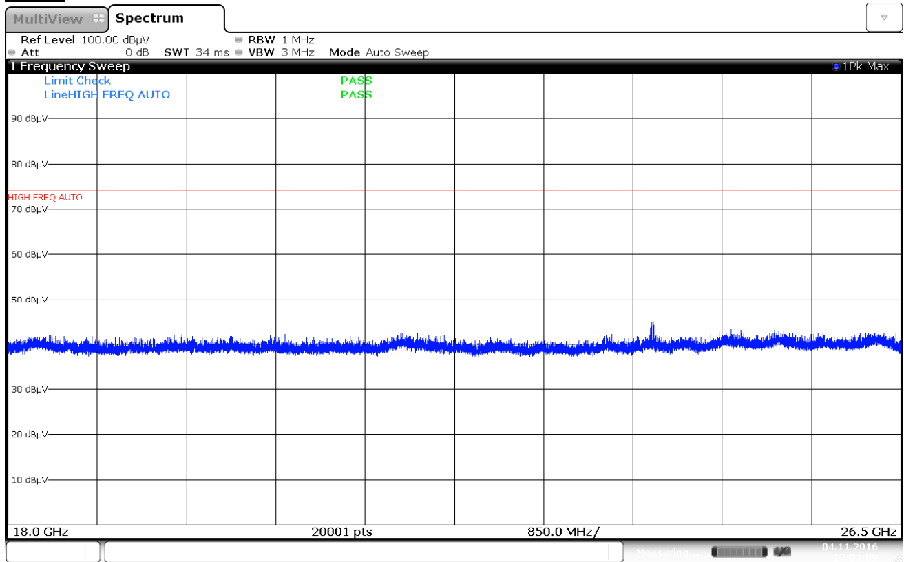
Plot 7-41. Radiated Spurious Plot above 18GHz (Pol. H)
