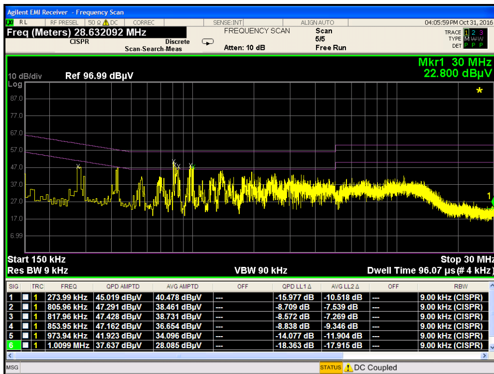
Plot 7-54. Line Conducted Plot with 802.11b (N)
