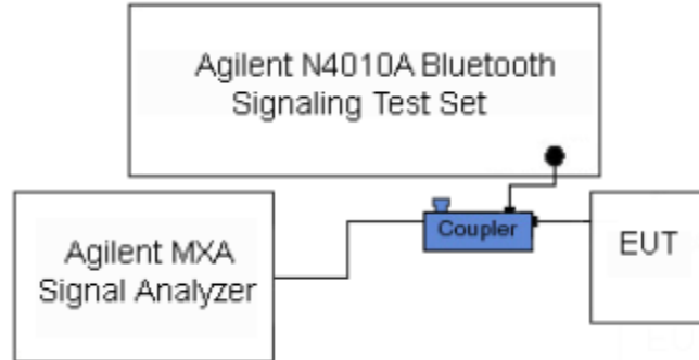
Figure 9-7 Power Measurement Setup
