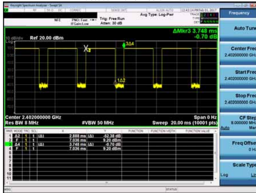
Figure 9-6 Bluetooth Transmission Plot
