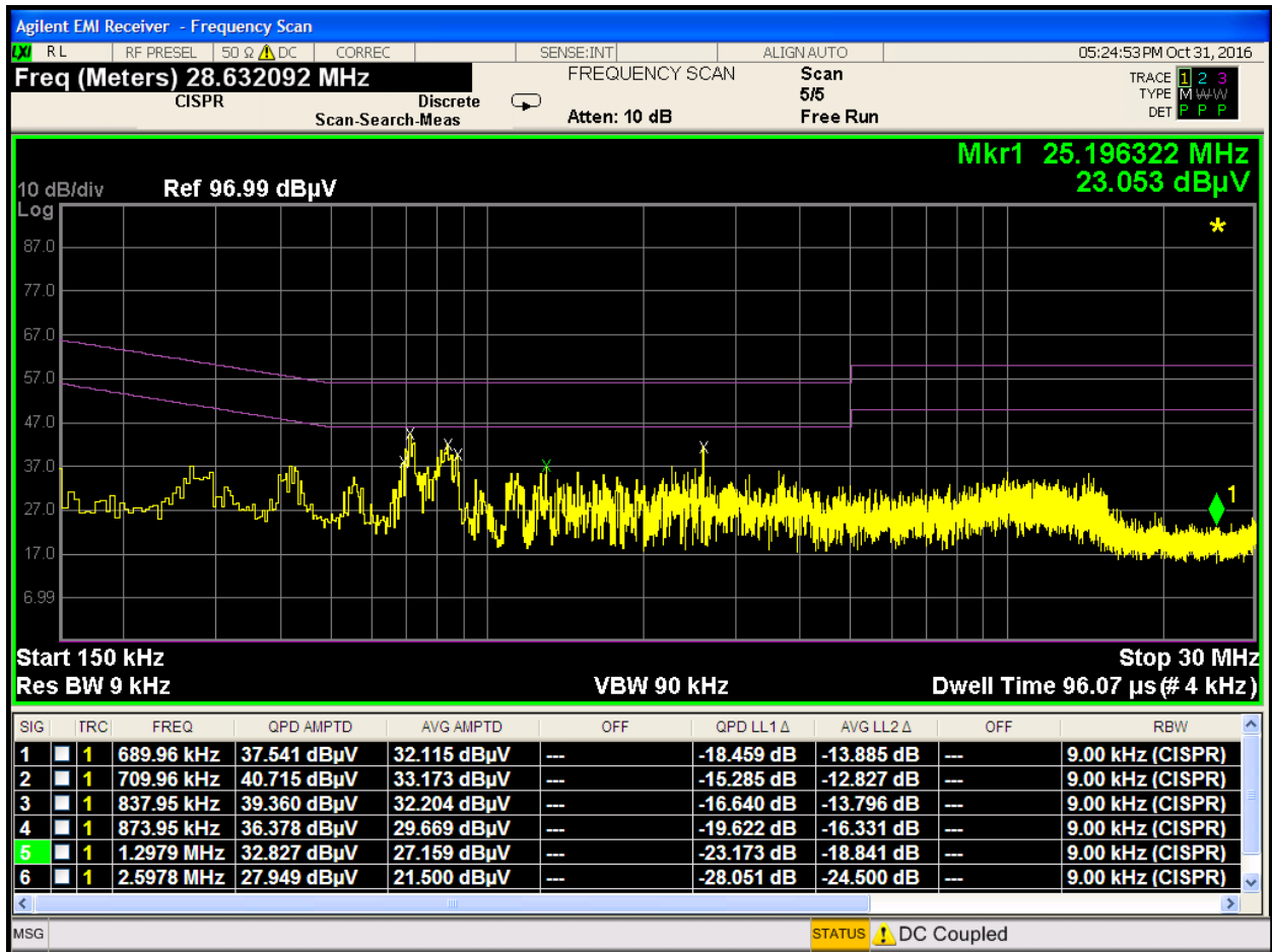
Plot 7-6. Line-Conducted Test Plot (L1)
