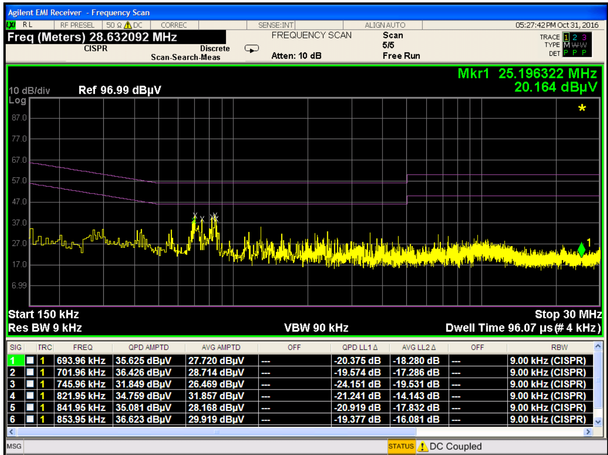
Plot 7-7. Line-Conducted Test Plot (N)
