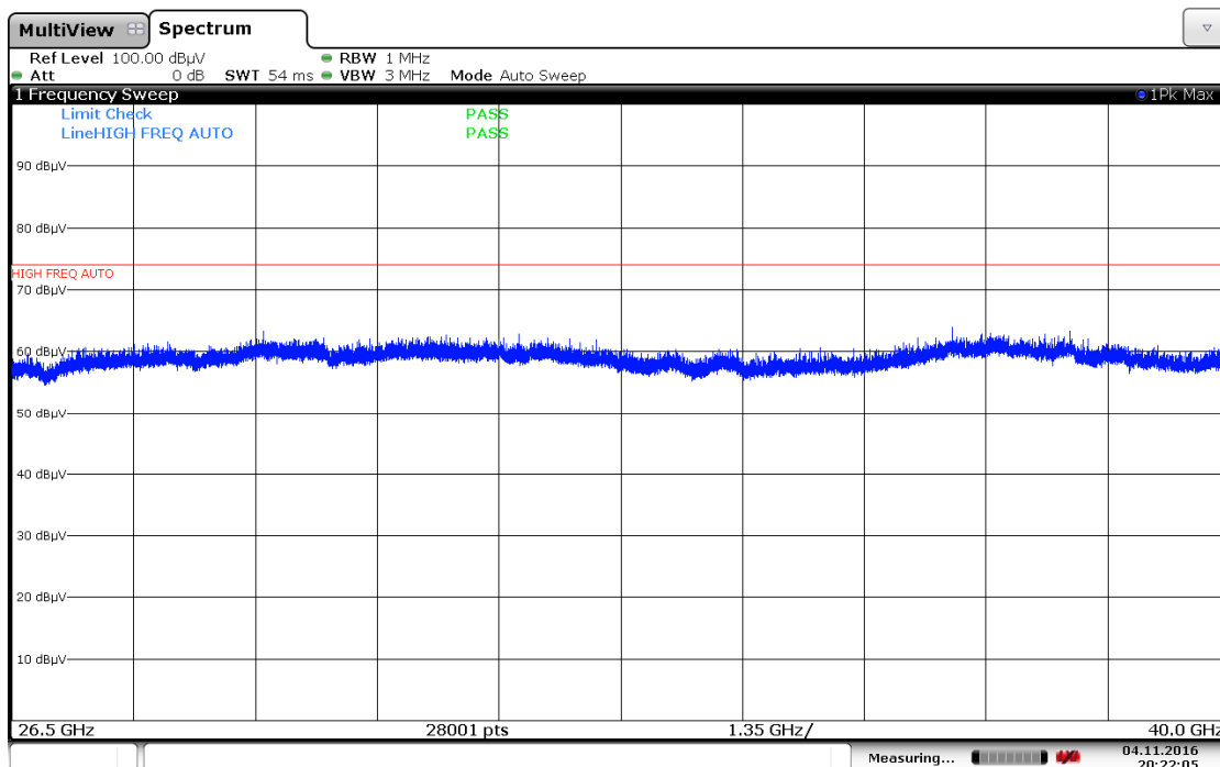
Plot 7-90. Radiated Spurious Plot above 26.5GHz (802.11a – Ant. Pol. V)
