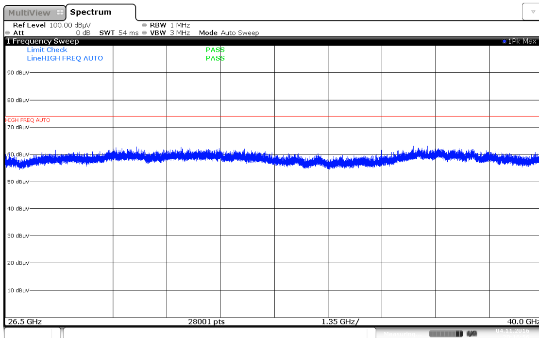
Plot 7-89. Radiated Spurious Plot above 26.5GHz (802.11a – Ant. Pol. H)
