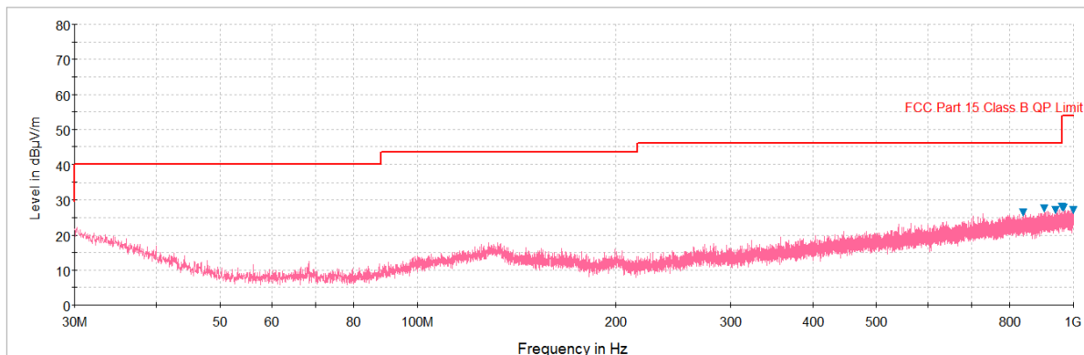
Plot 7-51. Radiated Spurious Plot below 1GHz (Pol. H)
