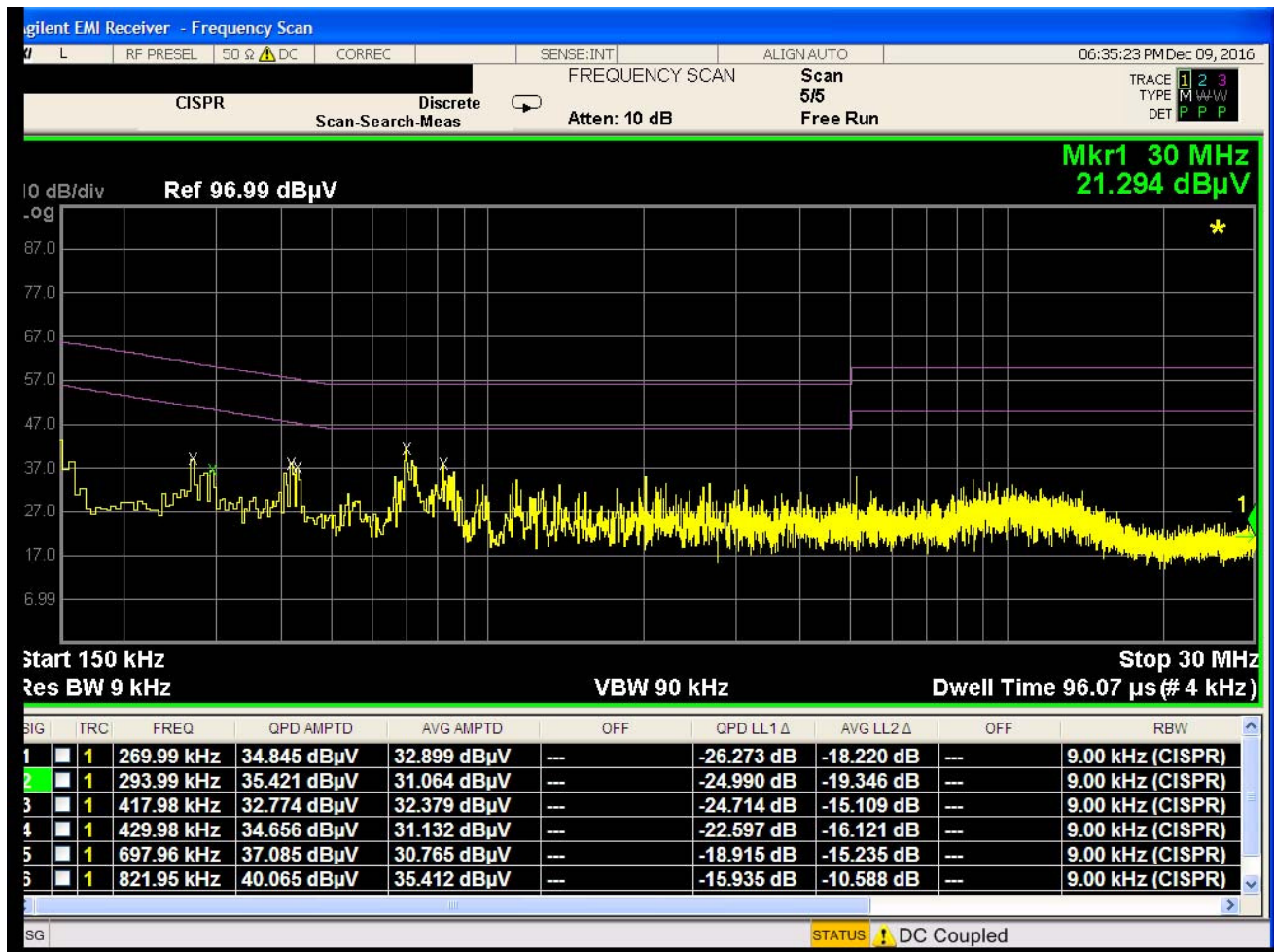
Plot 7-2. Line Conducted Plot (N)
