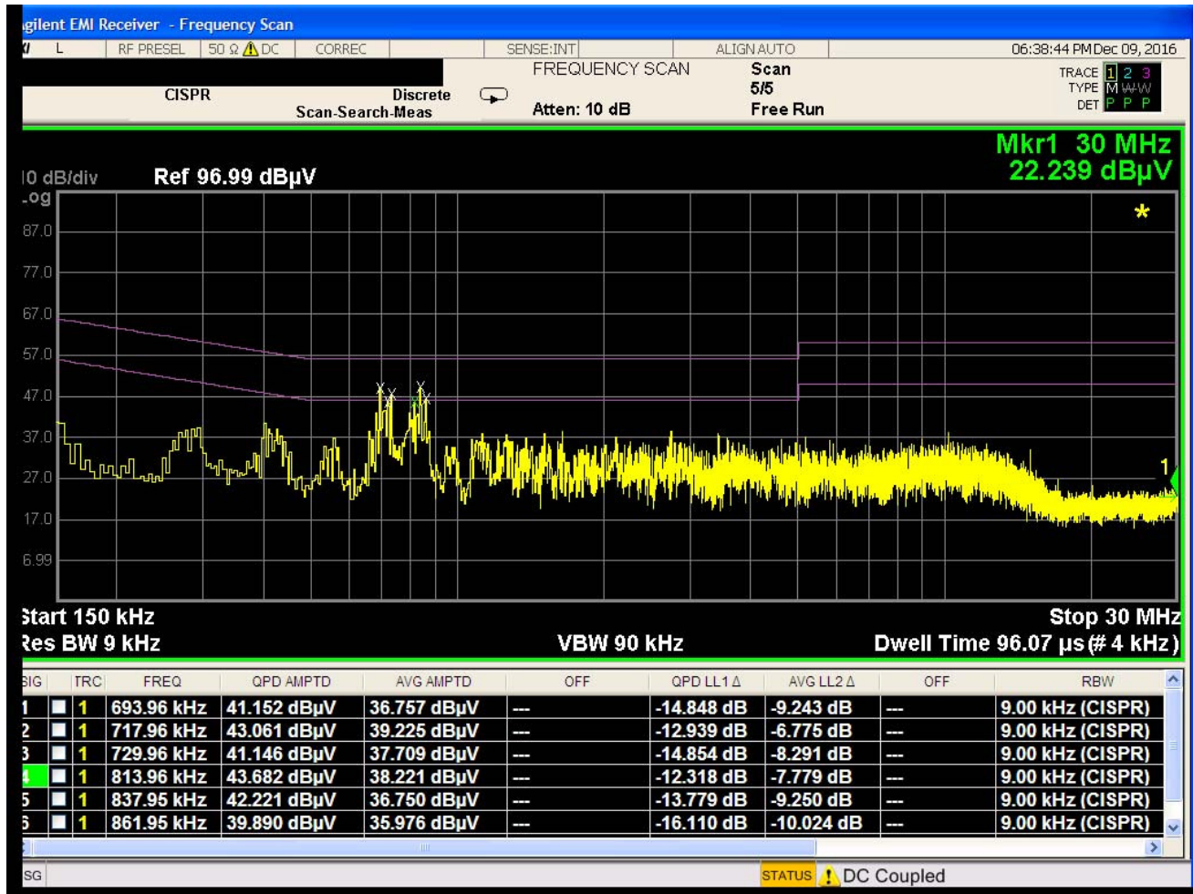
Plot 7-1. Line Conducted Plot (L1)
