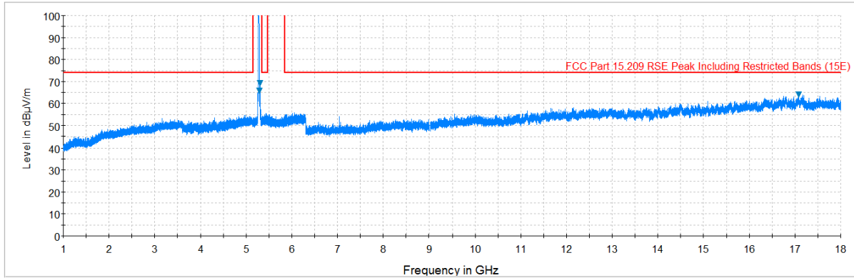
Plot 7-82. Radiated Spurious Plot above 1GHz (802.11a – U2A Ch. 56, Ant. Pol. V)
