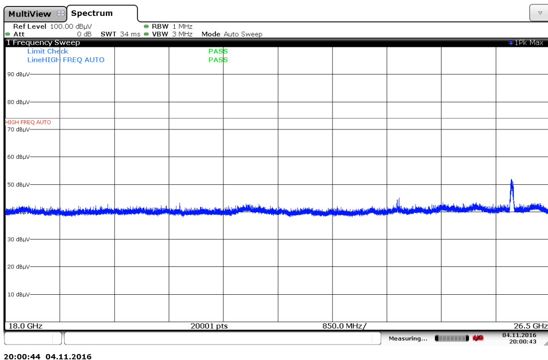
Plot 7-87. Radiated Spurious Plot above 18GHz (802.11a – Ant. Pol. H)
