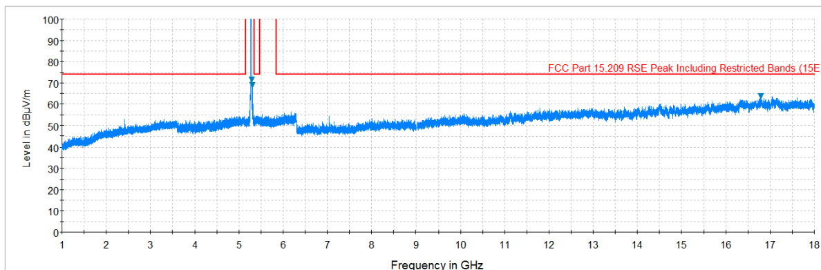
Plot 7-81. Radiated Spurious Plot above 1GHz (802.11a – U2A Ch. 56, Ant. Pol. H)
