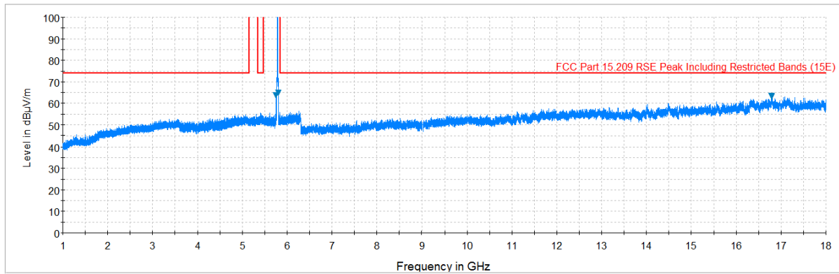
Plot 7-86. Radiated Spurious Plot above 1GHz (802.11a – U3 Ch. 157, Ant. Pol. V)
