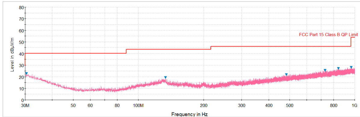
Plot 7-112. Radiated Spurious Plot below 1GHz (802.11a – U3 Ch. 157, Ant. Pol. H)
