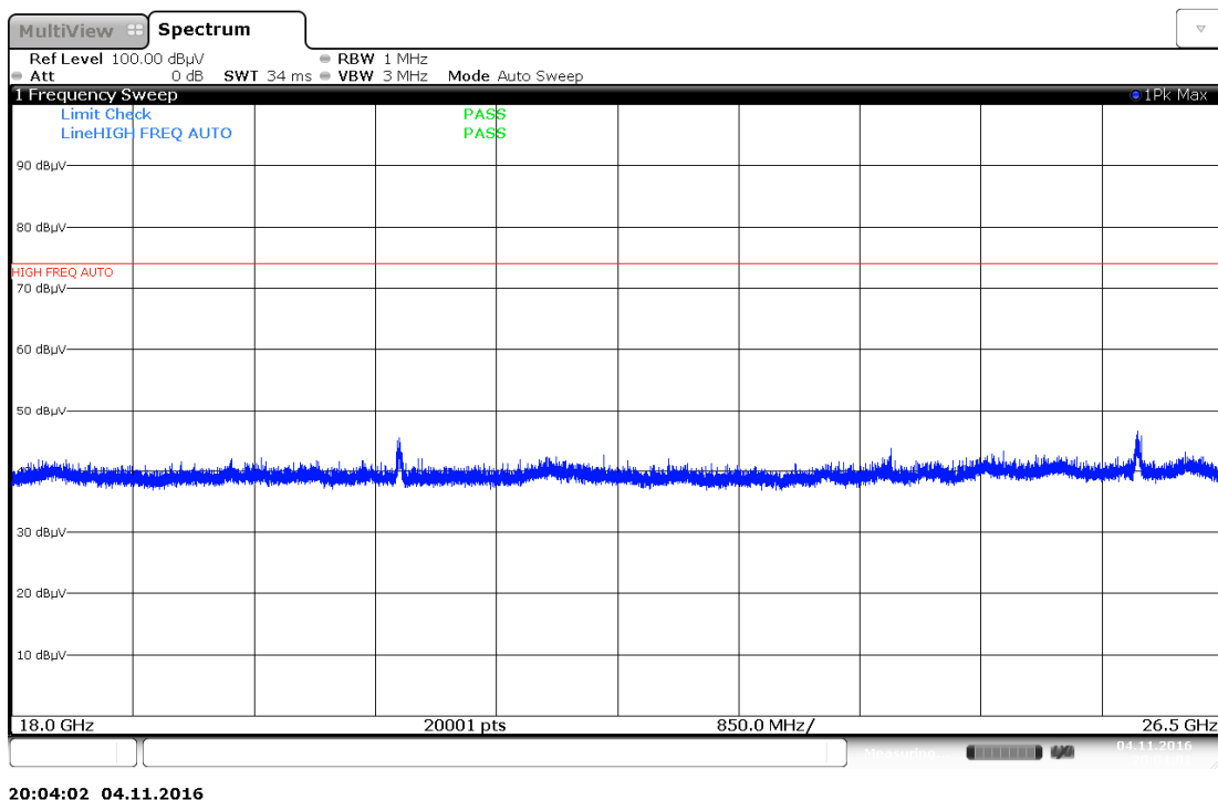
Plot 7-88. Radiated Spurious Plot above 18GHz (802.11a – Ant. Pol. V)
