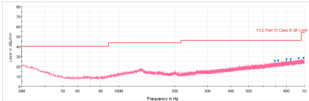
Plot 7-113. Radiated Spurious Plot below 1GHz (802.11a – U3 Ch. 157, Ant. Pol. V)
