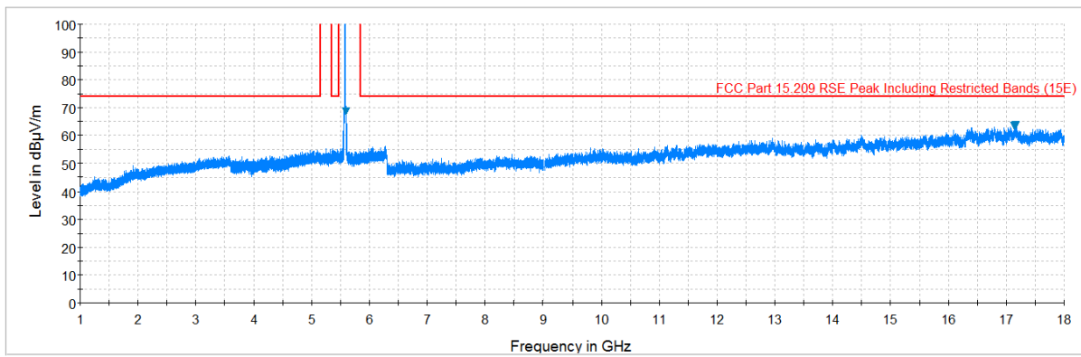
Plot 7-83. Radiated Spurious Plot above 1GHz (802.11a – U2C Ch. 116, Ant. Pol. H)
