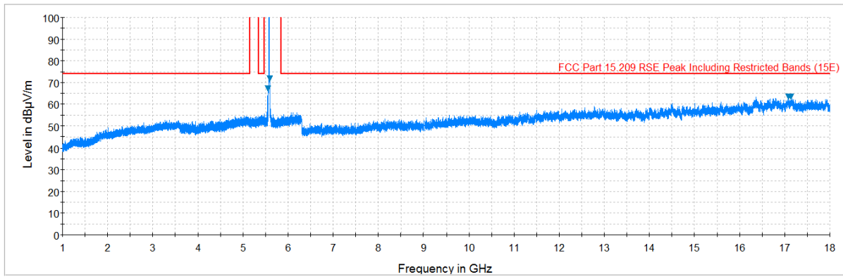
Plot 7-84. Radiated Spurious Plot above 1GHz (802.11a – U2C Ch. 116, Ant. Pol. V)
