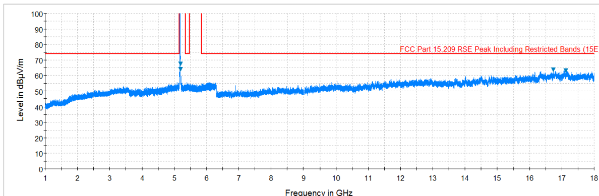
Plot 7-80. Radiated Spurious Plot above 1GHz (802.11a – U1 Ch. 40, Ant. Pol. V)
