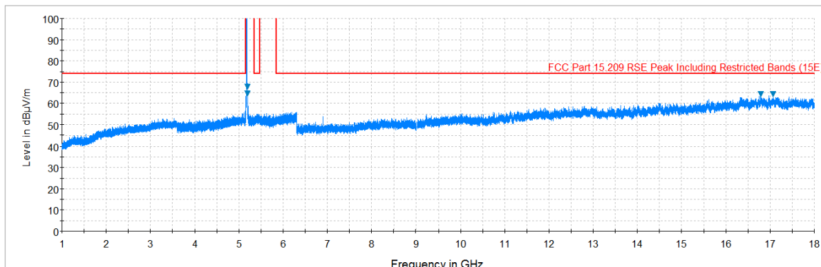
Plot 7-79. Radiated Spurious Plot above 1GHz (802.11a – U1 Ch. 40, Ant. Pol. H)
