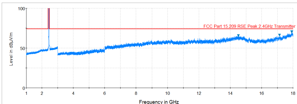
Plot 7-37. Radiated Spurious Plot above 1GHz (802.11b – Ch. 6, Ant. Pol. H)
