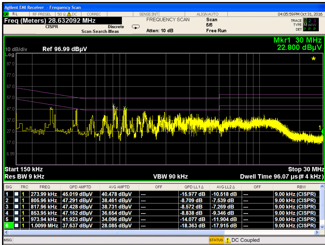
Plot 7-54. Line Conducted Plot with 802.11b (N)
