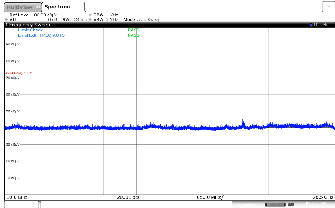
Plot 7-42. Radiated Spurious Plot above 18GHz (Pol. V)
