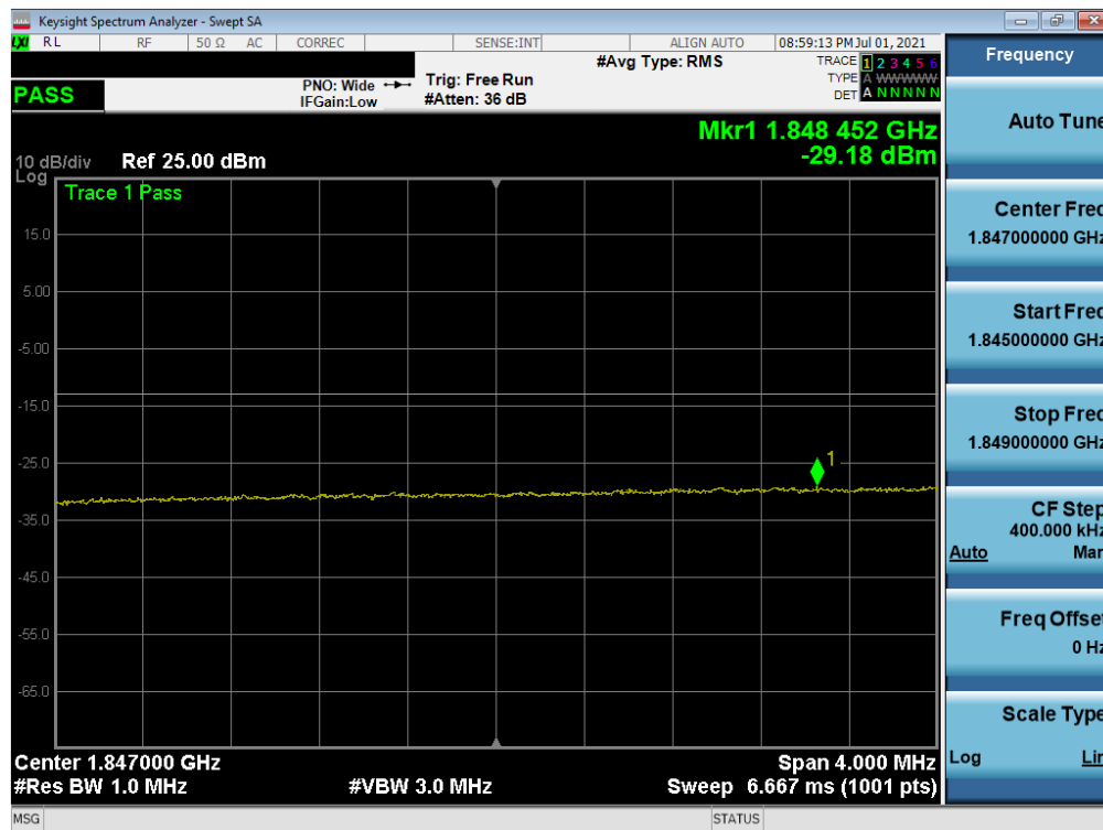
Plot 7-48. Extended Lower Band Edge Plot (LTE Band 2 - 15MHz QPSK – Full RB)
