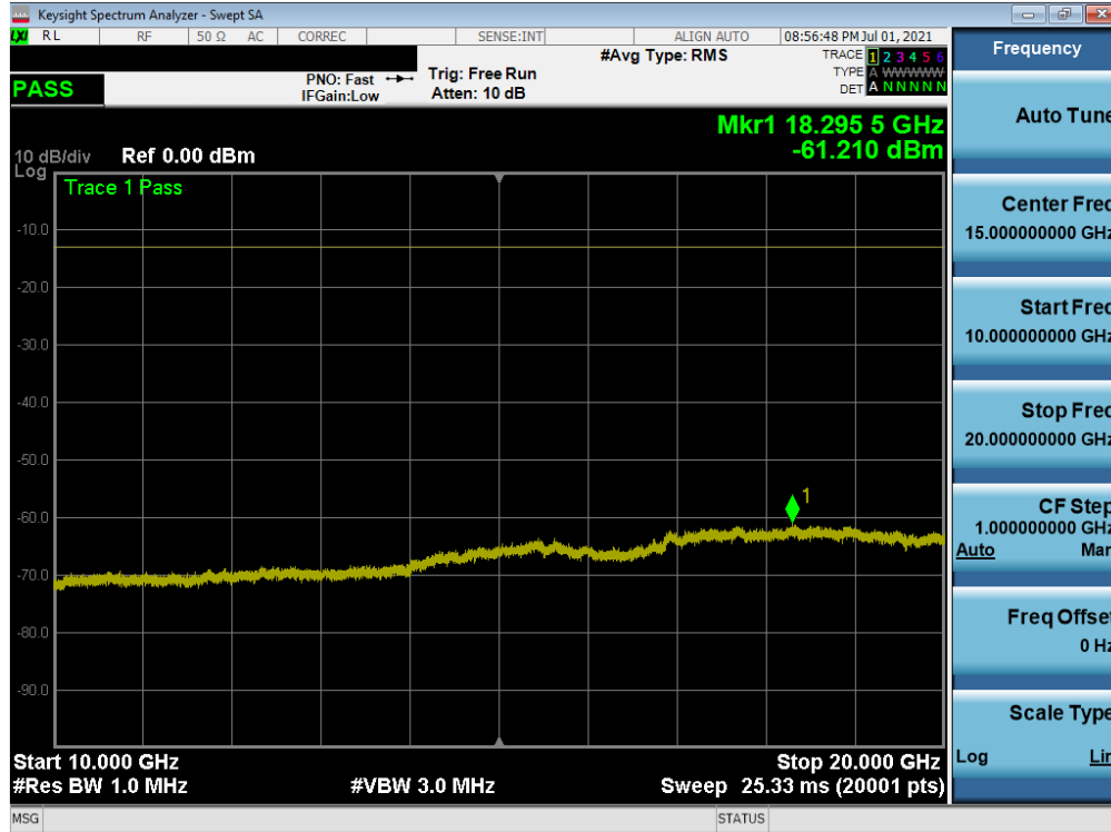
Plot 7-18. Conducted Spurious Plot (LTE Band 2 - 20MHz QPSK - 1RB - Low Channel)
