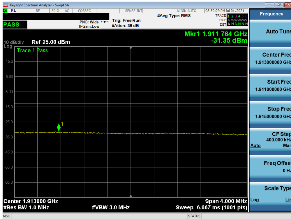
Plot 7-50. Extended Upper Band Edge Plot (LTE Band 2 - 15MHz QPSK – Full RB)
