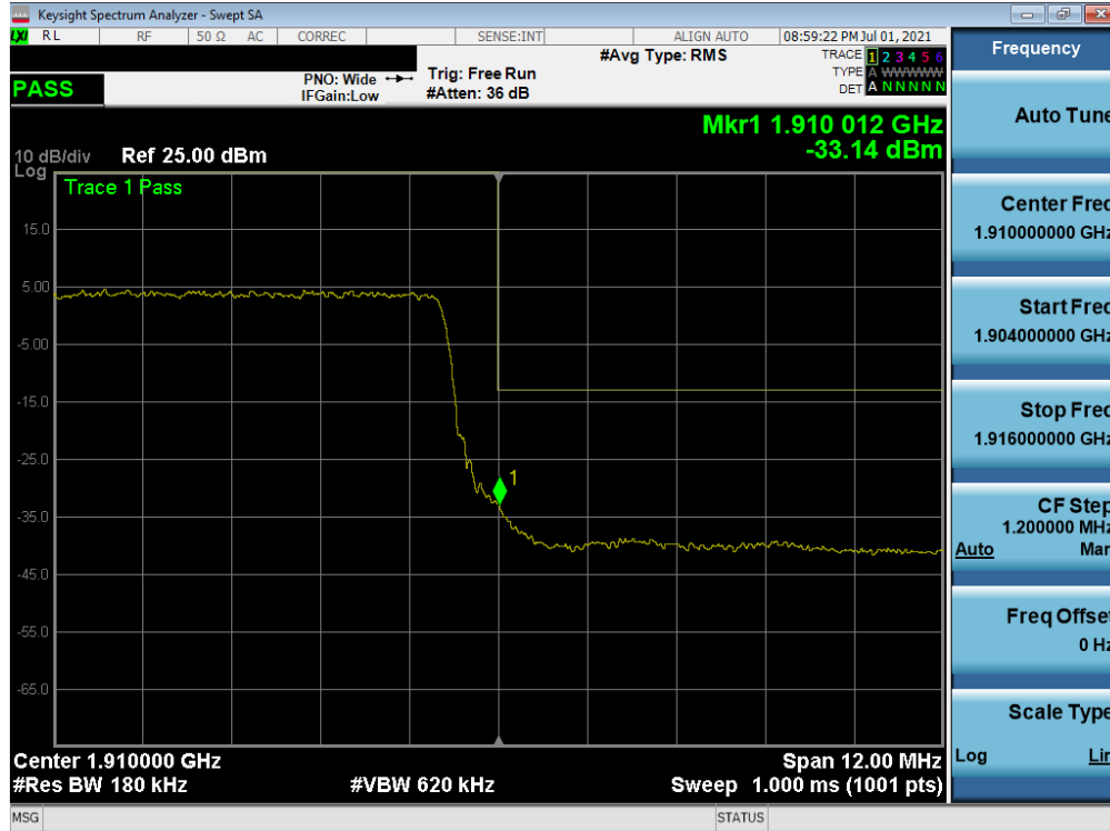
Plot 7-49. Upper Band Edge Plot (LTE Band 2 - 15MHz QPSK – Full RB)
