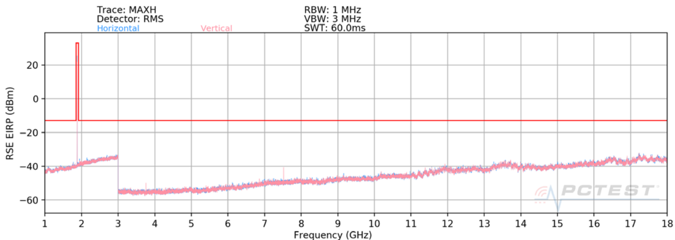
Plot 7-89. Radiated Spurious Plot (GPRS PCS)
