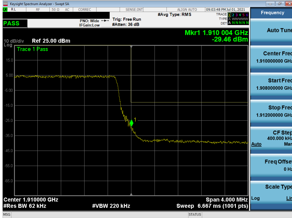
Plot 7-57. Upper Band Edge Plot (LTE Band 2 - 5MHz QPSK – Full RB)
