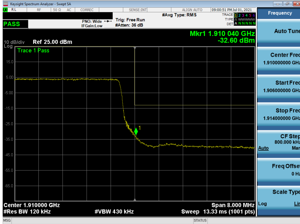
Plot 7-53. Upper Band Edge Plot (LTE Band 2 - 10MHz QPSK – Full RB)
