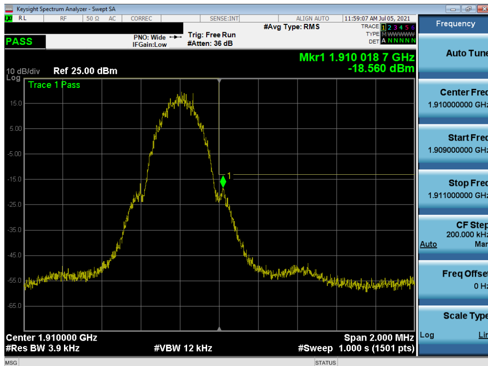
Plot 7-68. Upper Band Edge Plot (GPRS PCS – Ch. 810)
