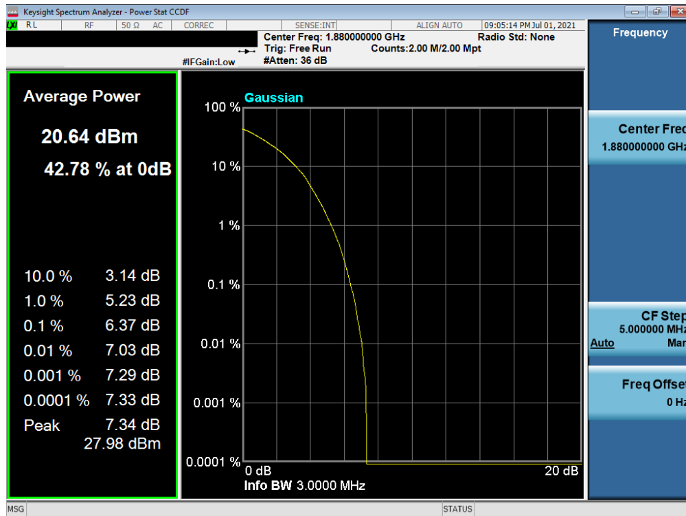
Plot 7-82. PAR Plot (LTE Band 2 - 3MHz 64-QAM - Full RB)
