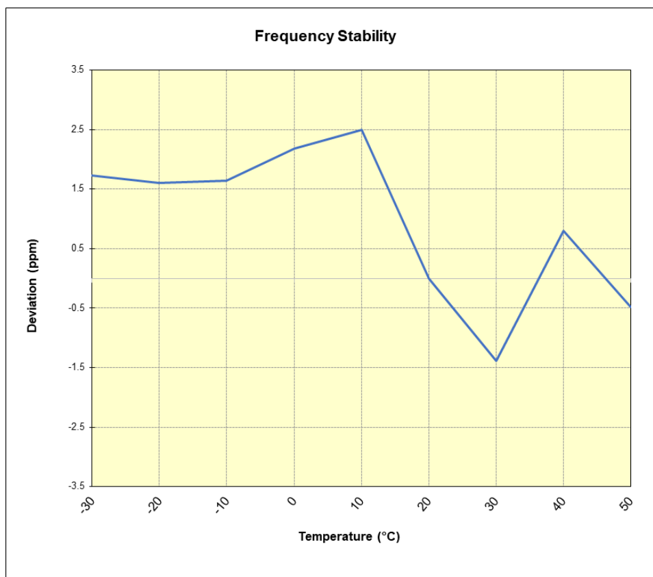
Plot 7-27. LTE Band 41(PC2) Frequency Stability Chart
