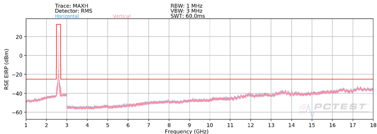
Plot 7-26. Radiated Spurious Plot (LTE Band 41(PC3))
