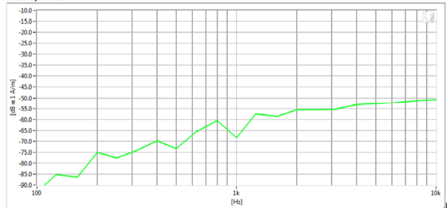
Noise Spectrum
