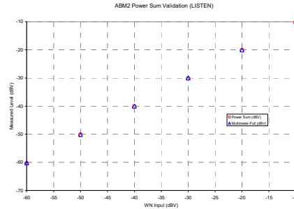
Figure 4-9 ABM2 Power Sum Validation
