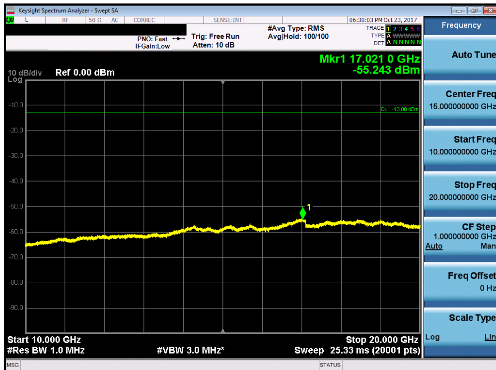
Plot 7-117. Conducted Spurious Plot (Band 2 - 5.0MHz QPSK - RB Size 1, RB Offset 0 - Mid Channel)
