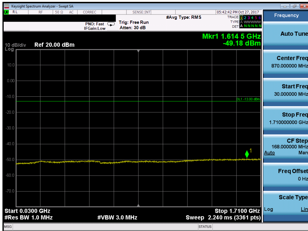
Plot 7-106. Conducted Spurious Plot (Band 66/4 - 15.0MHz QPSK - RB Size 1, RB Offset 0 - Mid Channel)
