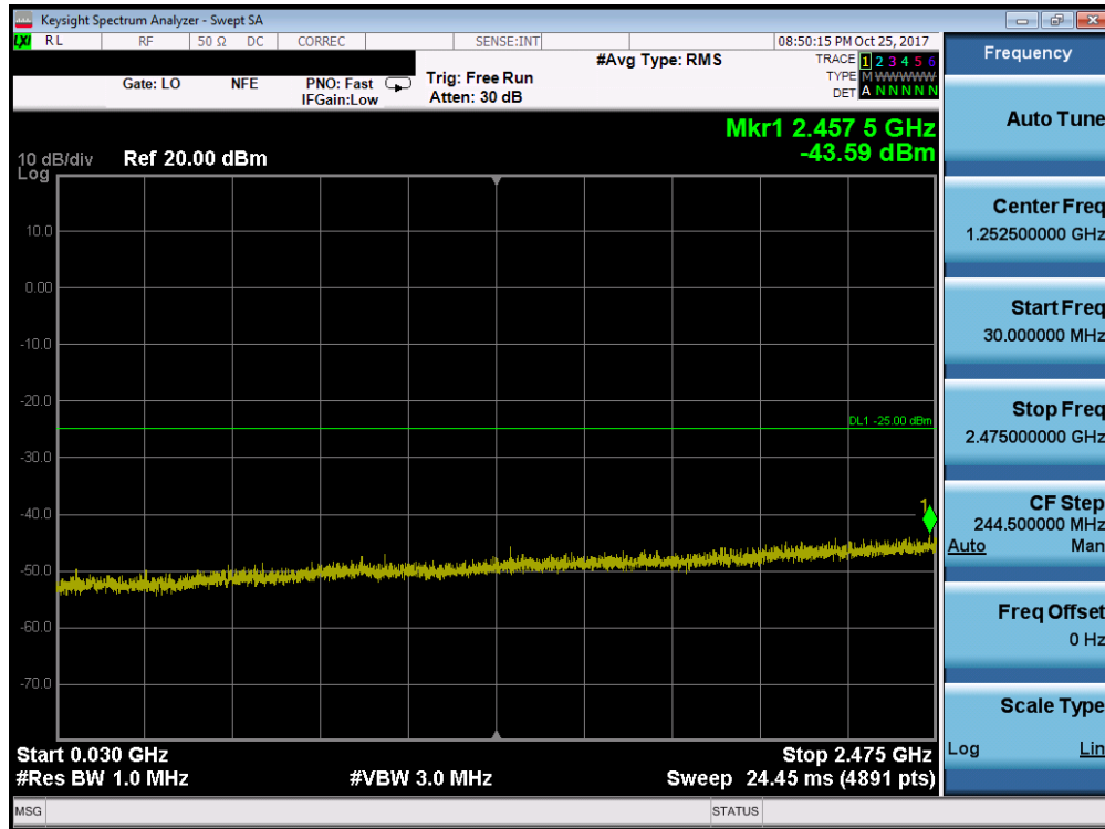
Plot 7-121. Conducted Spurious Plot (Band 41 - 5.0MHz QPSK - RB Size 1, RB Offset 0 - Low Channel)
