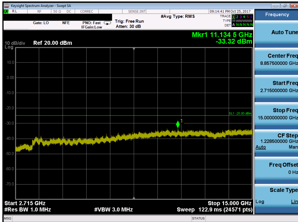
Plot 7-128. Conducted Spurious Plot (Band 41 - 5.0MHz QPSK - RB Size 1, RB Offset 0 - High Channel)
