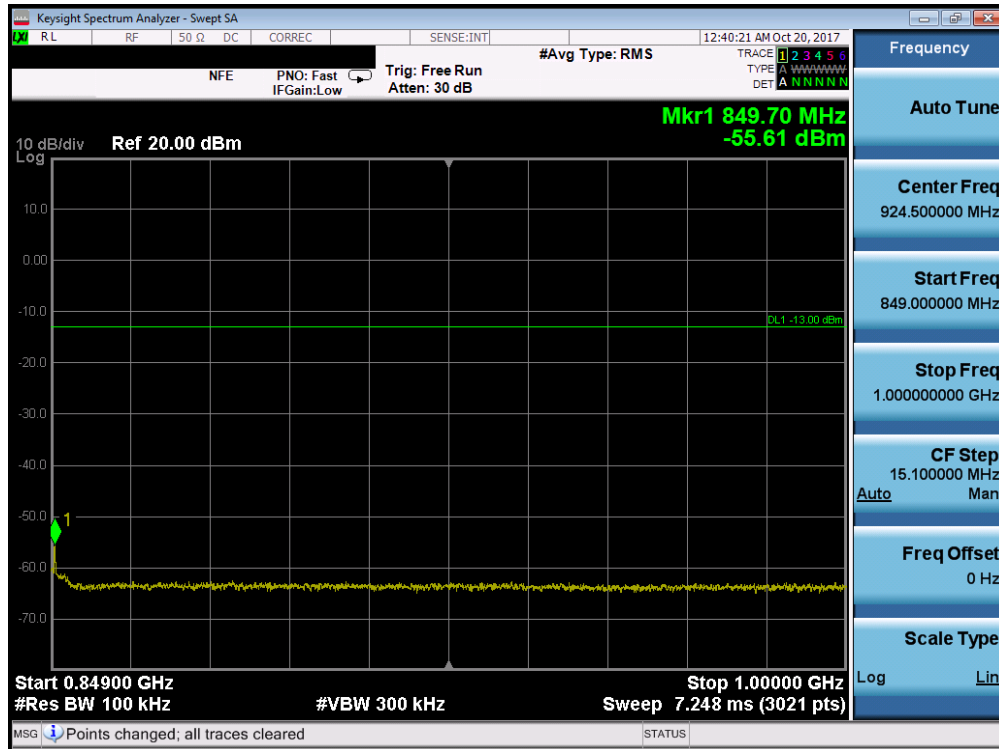
Plot 7-98. Conducted Spurious Plot (Band 26/5 - 5.0MHz QPSK - RB Size 1, RB Offset 0 - Mid Channel)
