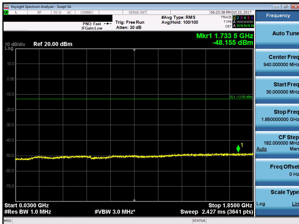
Plot 7-115. Conducted Spurious Plot (Band 2 - 5.0MHz QPSK - RB Size 1, RB Offset 0 - Mid Channel)
