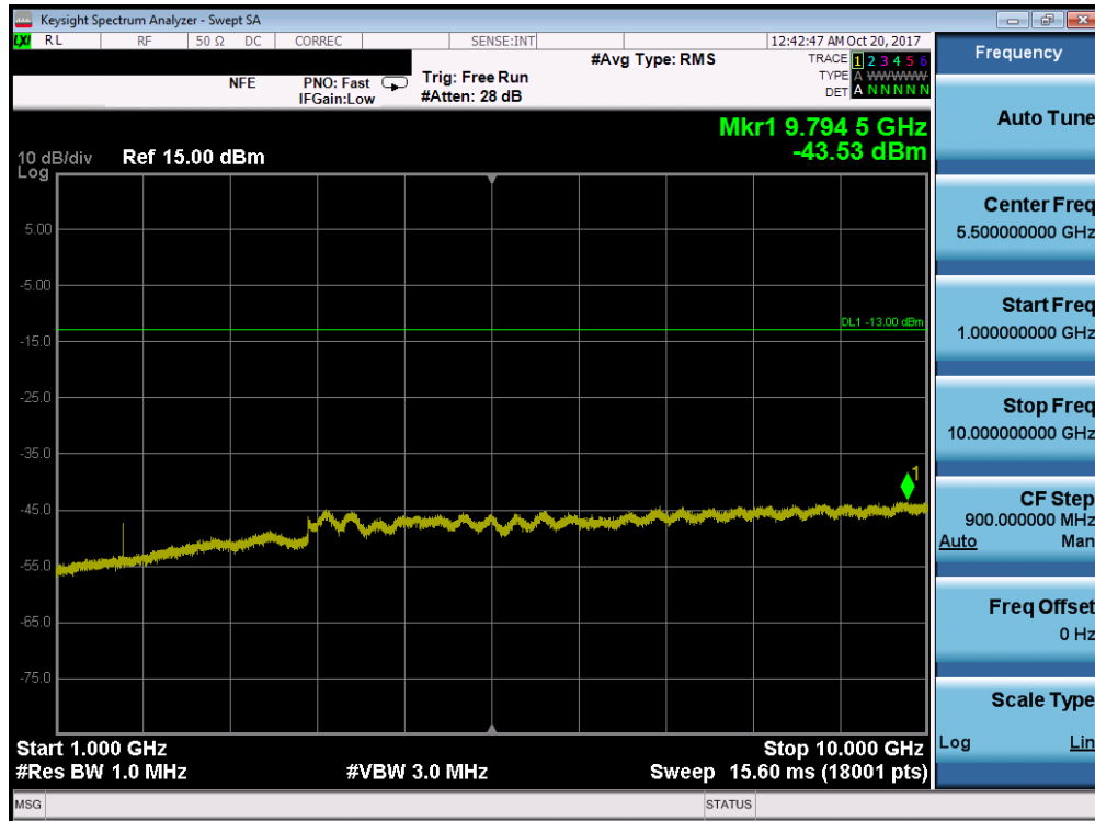
Plot 7-102. Conducted Spurious Plot (Band 26/5 - 5.0MHz QPSK - RB Size 1, RB Offset 0 - High Channel)
