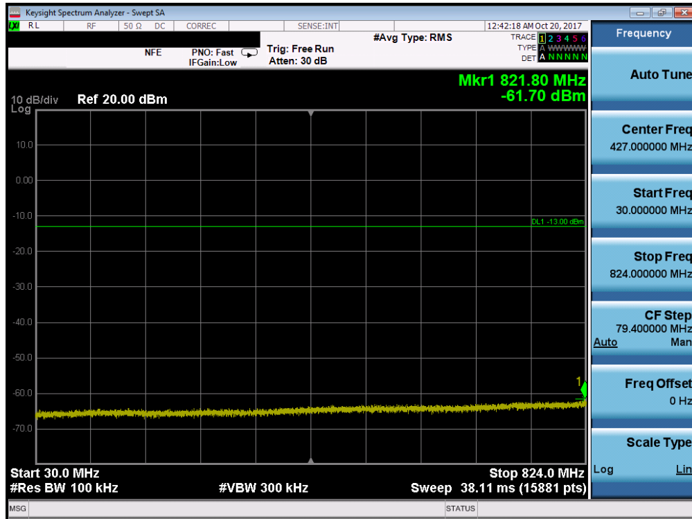
Plot 7-100. Conducted Spurious Plot (Band 26/5 - 5.0MHz QPSK - RB Size 1, RB Offset 0 - High Channel)
