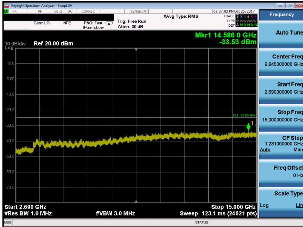
Plot 7-125. Conducted Spurious Plot (Band 41 - 5.0MHz QPSK - RB Size 1, RB Offset 0 - Mid Channel)
