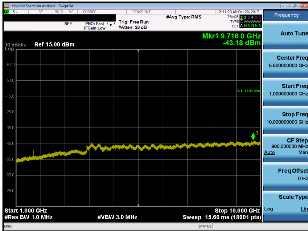
Plot 7-96. Conducted Spurious Plot (Band 26/5 - 5.0MHz QPSK - RB Size 1, RB Offset 0 - Low Channel)
