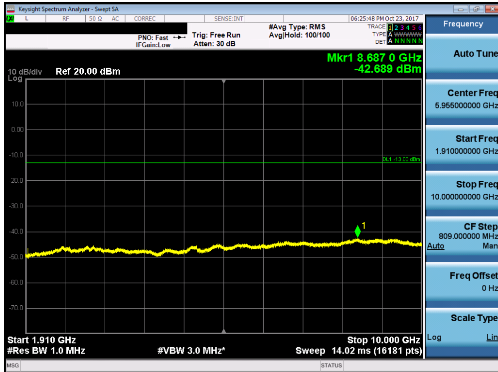
Plot 7-116. Conducted Spurious Plot (Band 2 - 5.0MHz QPSK - RB Size 1, RB Offset 0 - Mid Channel)
