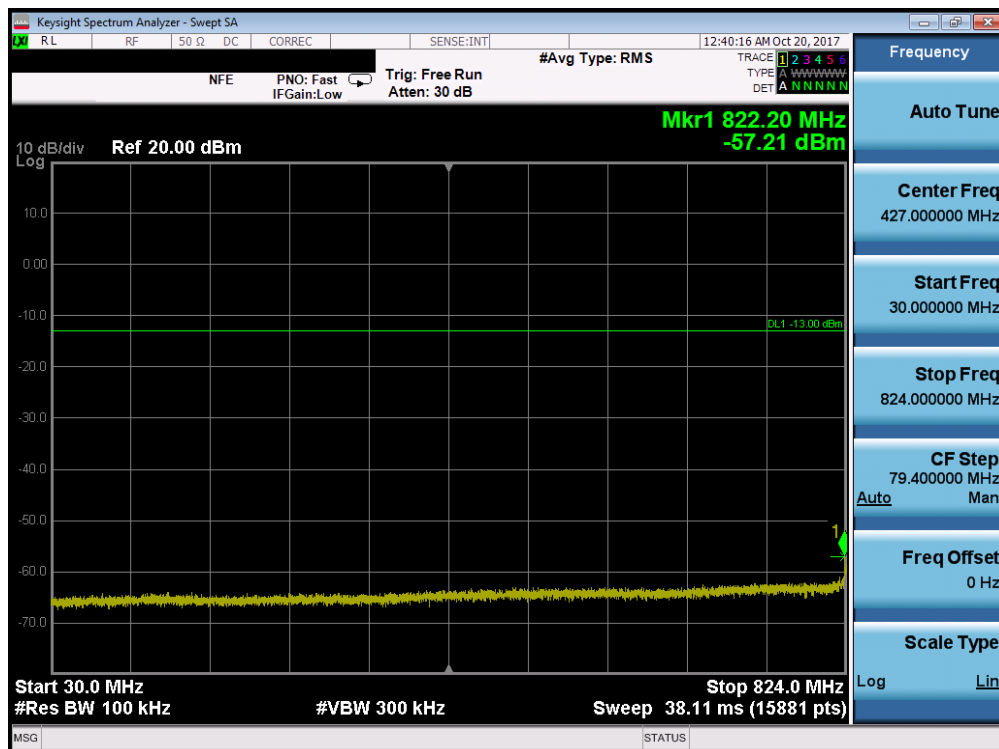
Plot 7-97. Conducted Spurious Plot (Band 26/5 - 5.0MHz QPSK - RB Size 1, RB Offset 0 - Mid Channel)
