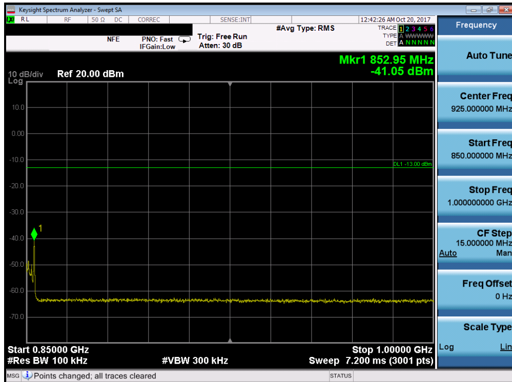
Plot 7-101. Conducted Spurious Plot (Band 26/5 - 5.0MHz QPSK - RB Size 1, RB Offset 0 - High Channel)
