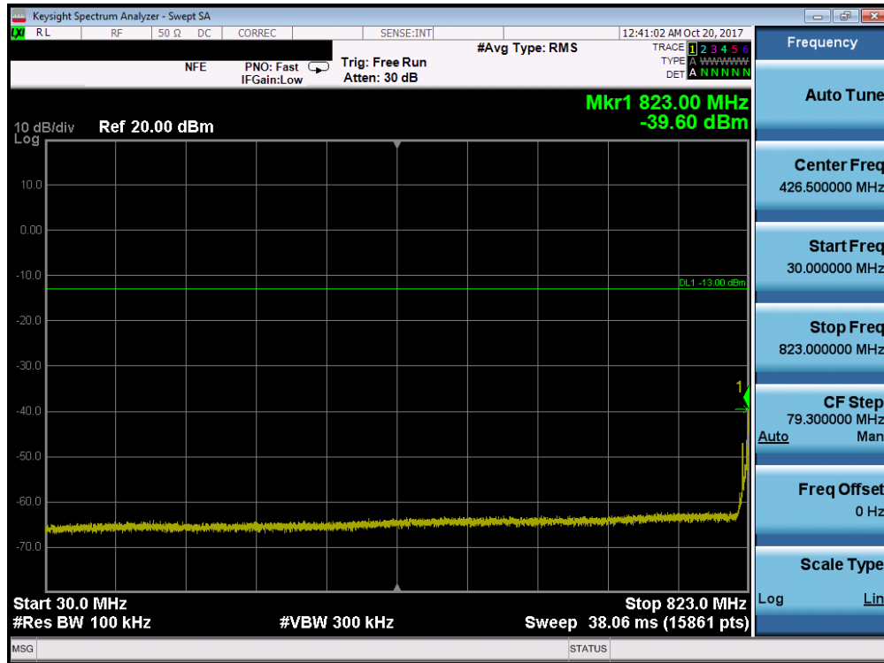
Plot 7-94. Conducted Spurious Plot (Band 26/5 - 5.0MHz QPSK - RB Size 1, RB Offset 0 - Low Channel)
