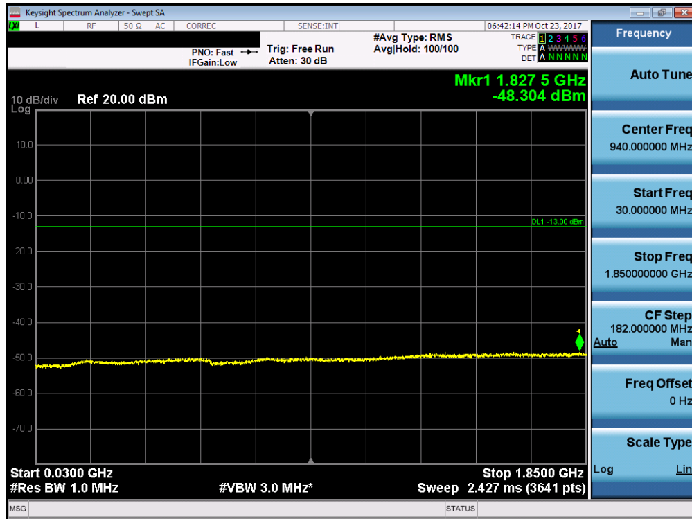
Plot 7-118. Conducted Spurious Plot (Band 2 - 5.0MHz QPSK - RB Size 1, RB Offset 0 - High Channel)
