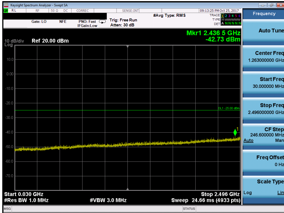
Plot 7-127. Conducted Spurious Plot (Band 41 - 5.0MHz QPSK - RB Size 1, RB Offset 0 - High Channel)
