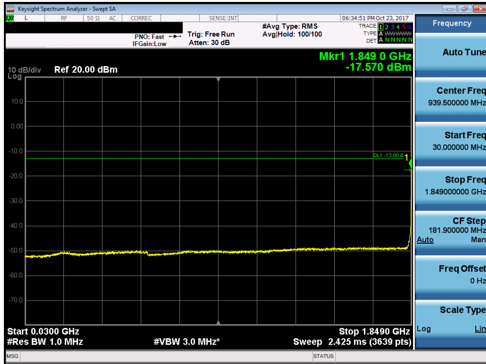
Plot 7-112. Conducted Spurious Plot (Band 2 - 5.0MHz QPSK - RB Size 1, RB Offset 0 - Low Channel)
