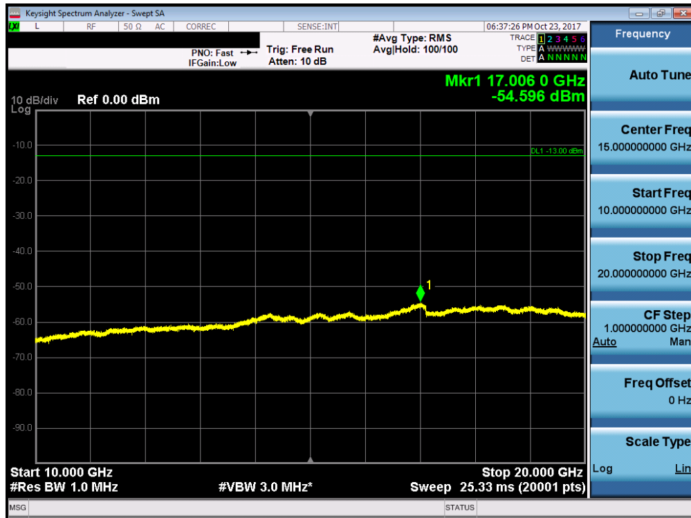
Plot 7-114. Conducted Spurious Plot (Band 2 - 5.0MHz QPSK - RB Size 1, RB Offset 0 - Low Channel)
