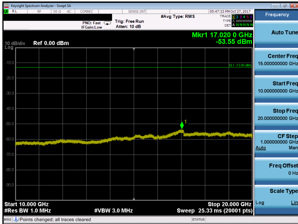
Plot 7-105. Conducted Spurious Plot (Band 66/4 - 15.0MHz QPSK - RB Size 1, RB Offset 0 - Low Channel)
