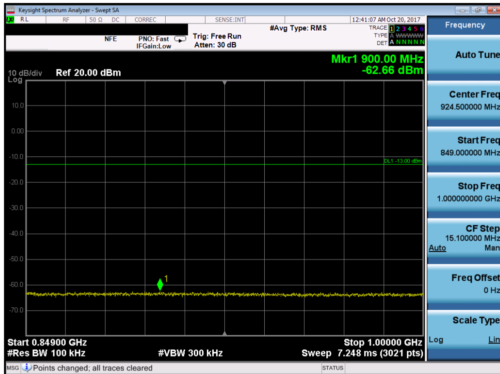
Plot 7-95. Conducted Spurious Plot (Band 26/5 - 5.0MHz QPSK - RB Size 1, RB Offset 0 - Low Channel)
