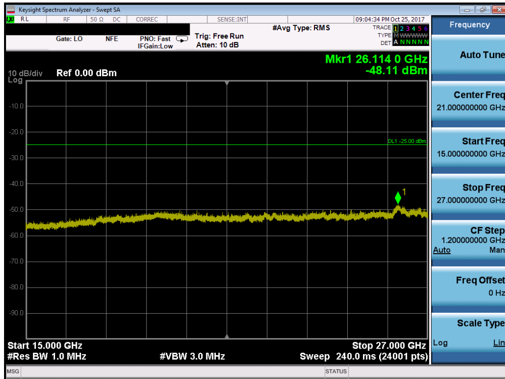
Plot 7-123. Conducted Spurious Plot (Band 41 - 5.0MHz QPSK - RB Size 1, RB Offset 0 - Low Channel)
