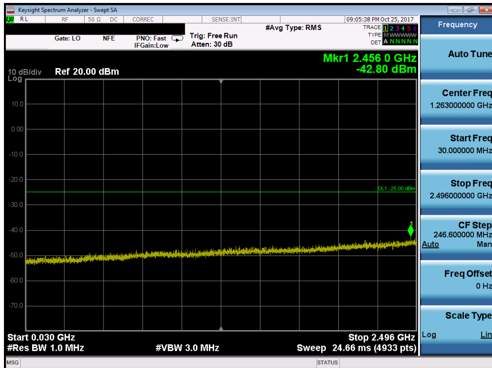
Plot 7-124. Conducted Spurious Plot (Band 41 - 5.0MHz QPSK - RB Size 1, RB Offset 0 - Mid Channel)
