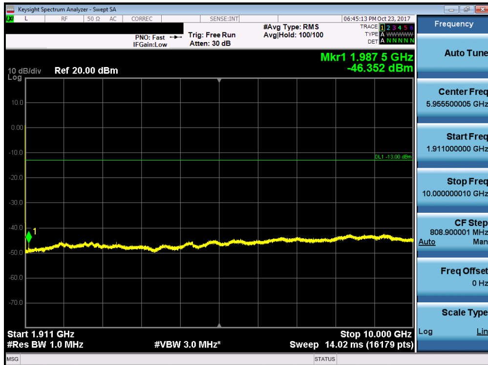
Plot 7-119. Conducted Spurious Plot (Band 2 - 5.0MHz QPSK - RB Size 1, RB Offset 0 - High Channel)
