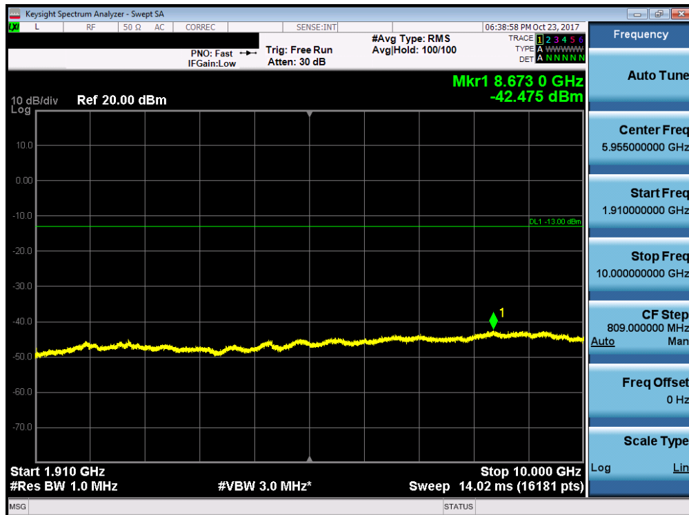
Plot 7-113. Conducted Spurious Plot (Band 2 - 5.0MHz QPSK - RB Size 1, RB Offset 0 - Low Channel)
