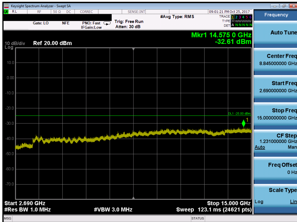
Plot 7-122. Conducted Spurious Plot (Band 41 - 5.0MHz QPSK - RB Size 1, RB Offset 0 - Low Channel)
