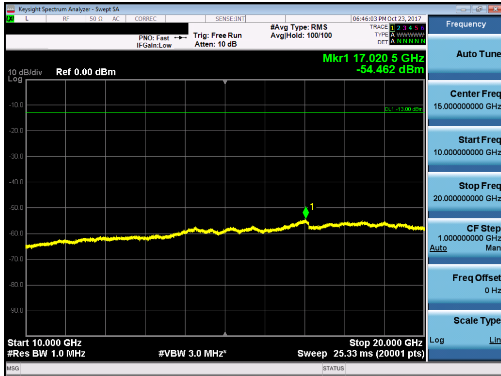
Plot 7-120. Conducted Spurious Plot (Band 2 - 5.0MHz QPSK - RB Size 1, RB Offset 0 - High Channel)
