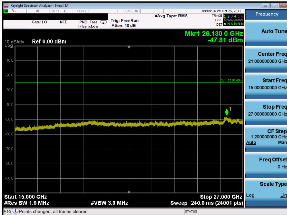
Plot 7-126. Conducted Spurious Plot (Band 41 - 5.0MHz QPSK - RB Size 1, RB Offset 0 - Mid Channel)
