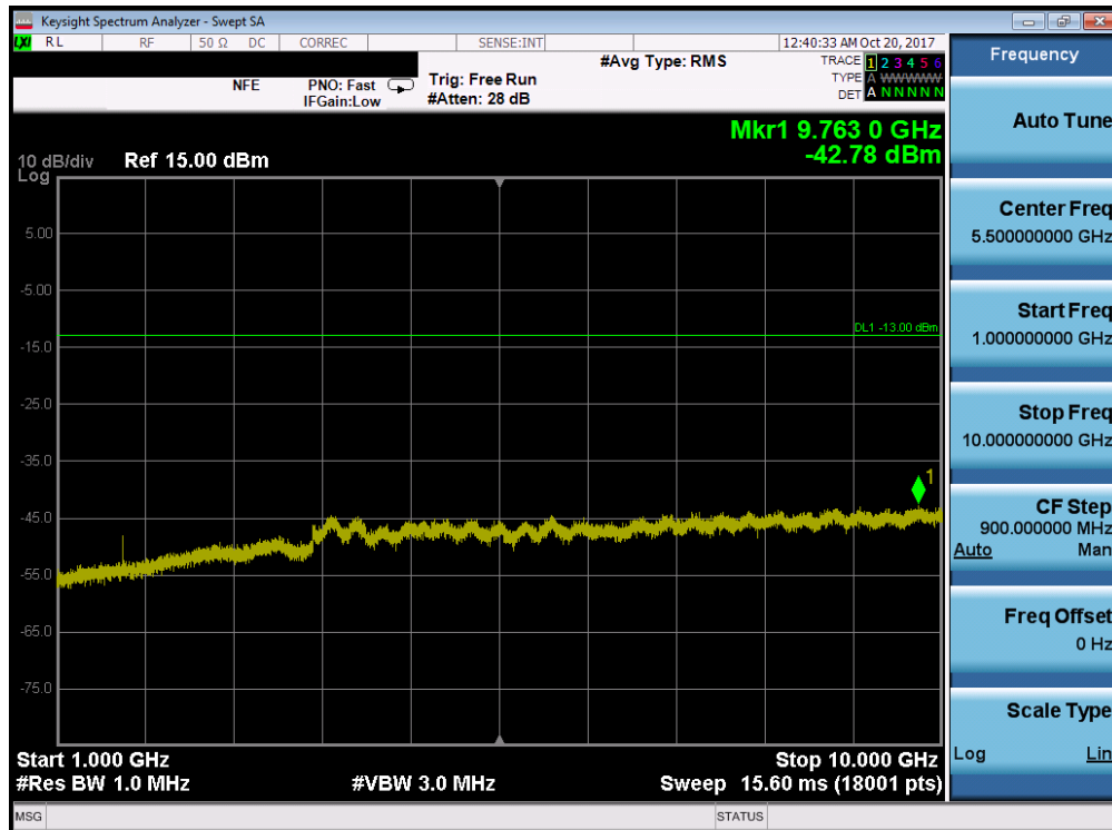
Plot 7-99. Conducted Spurious Plot (Band 26/5 - 5.0MHz QPSK - RB Size 1, RB Offset 0 - Mid Channel)
