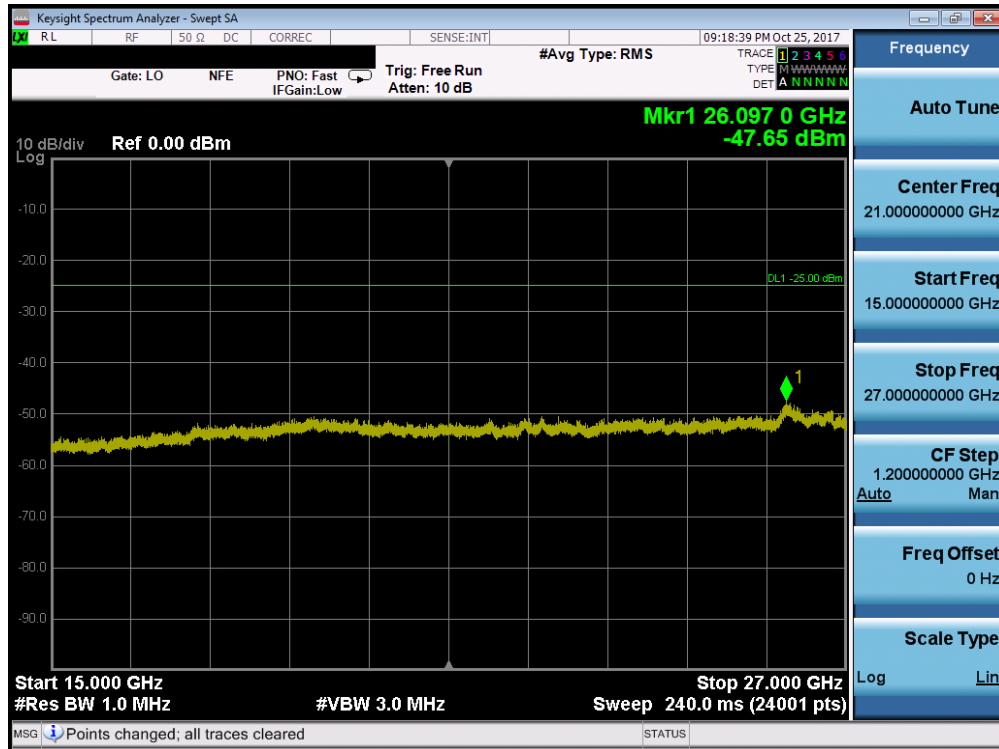
Plot 7-129. Conducted Spurious Plot (Band 41 - 5.0MHz QPSK - RB Size 1, RB Offset 0 - High Channel)
