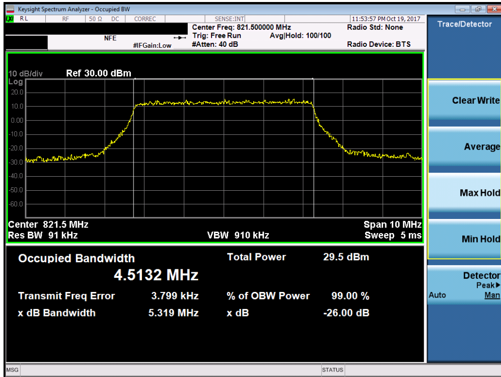
Plot 7-9. Occupied Bandwidth Plot (5MHz 64-QAM – RB Size 25– High Channel)
