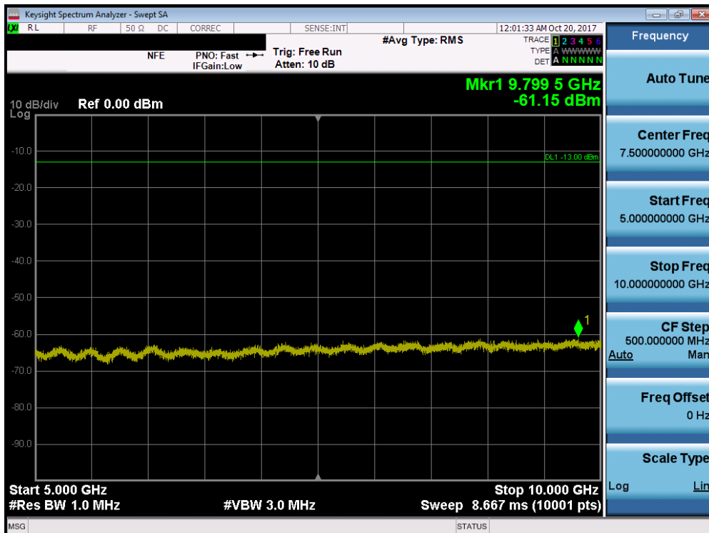
Plot 7-17. Conducted Spurious Plot (10.0MHz QPSK – RB Size 1, RB Offset 0 – High Channel)
