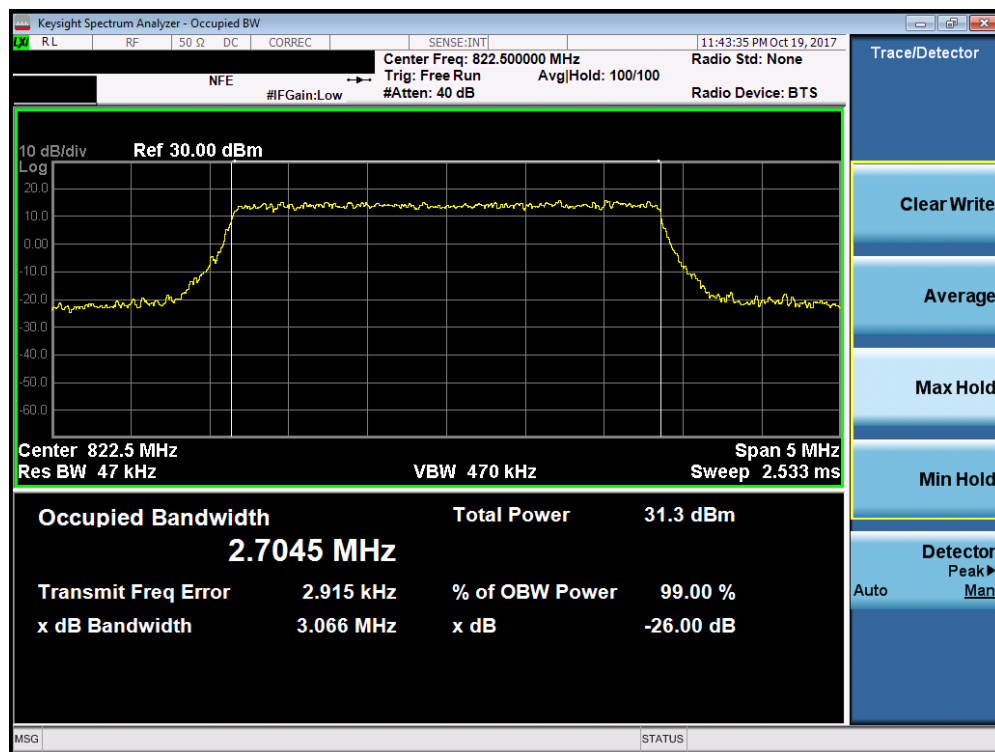
Plot 7-4. Occupied Bandwidth Plot (3MHz QPSK – RB Size 15– High Channel)
