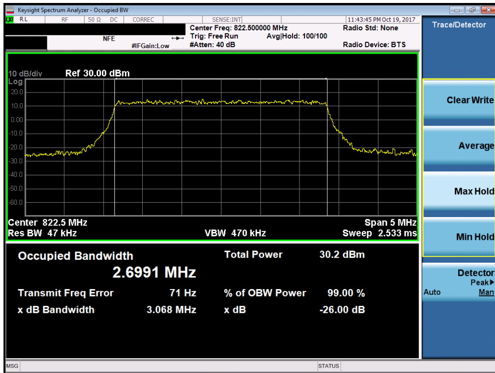
Plot 7-5. Occupied Bandwidth Plot (3MHz 16-QAM – RB Size 15– High Channel)
