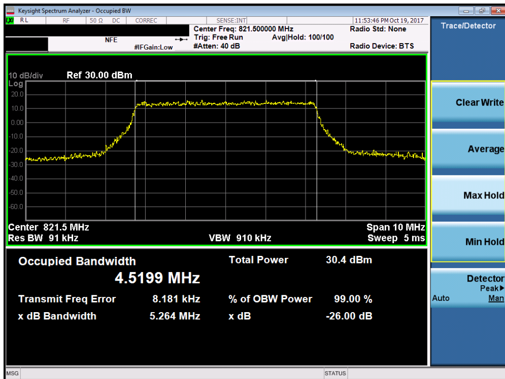
Plot 7-8. Occupied Bandwidth Plot (5MHz 16-QAM – RB Size 25– High Channel)
