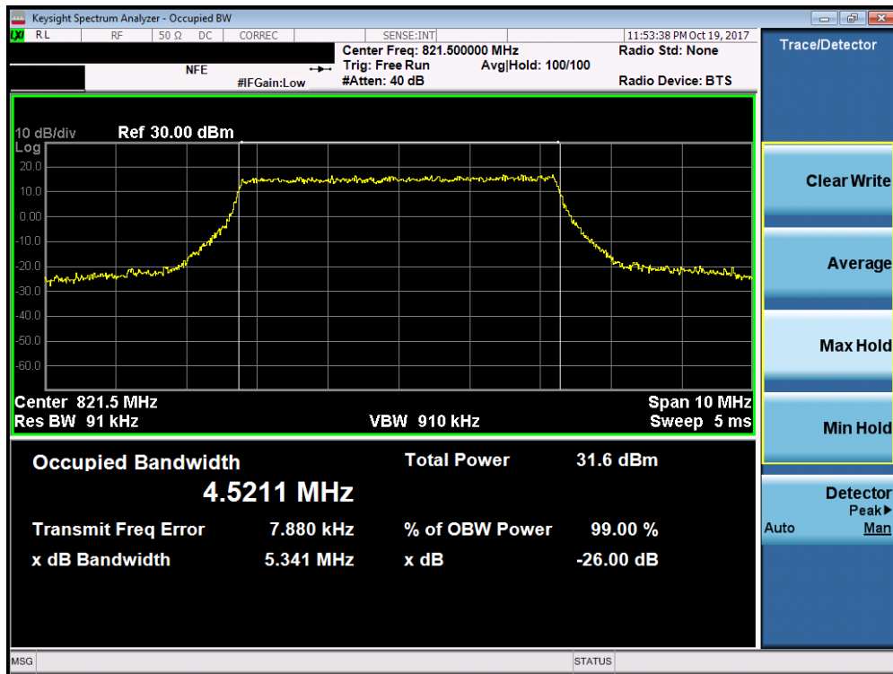
Plot 7-7. Occupied Bandwidth Plot (5MHz QPSK – RB Size 25– High Channel)
