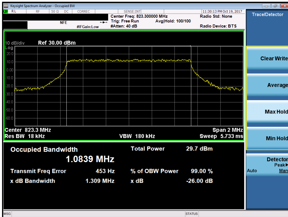
Plot 7-2. Occupied Bandwidth Plot (1.4MHz 16-QAM – RB Size 6– High Channel)
