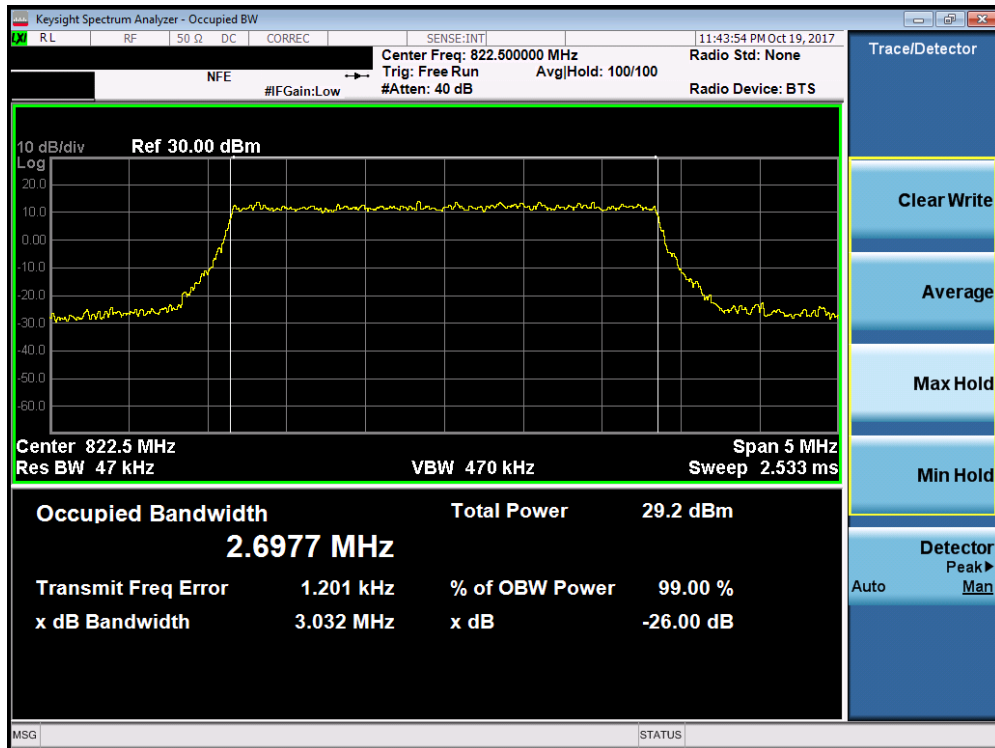
Plot 7-6. Occupied Bandwidth Plot (3MHz 64-QAM – RB Size 15– High Channel)
