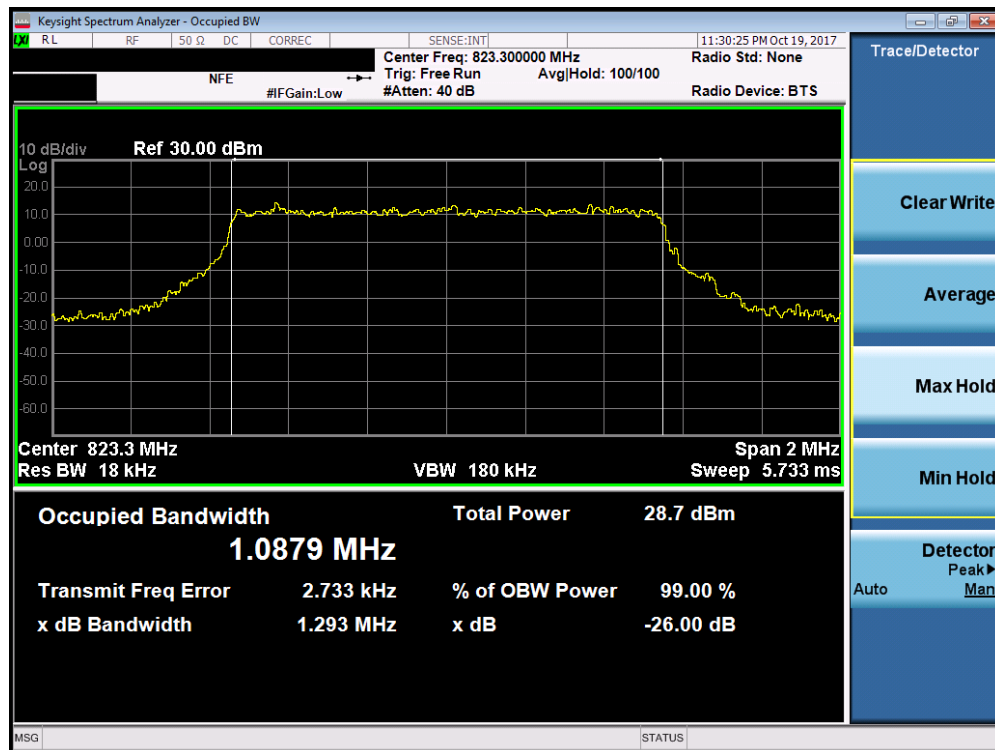
Plot 7-3. Occupied Bandwidth Plot (1.4MHz 64-QAM – RB Size 6– High Channel)
