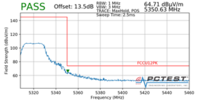
Plot 7-94. Radiated Upper Band Edge Plot (Peak – UNII Band 2A)
