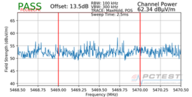
Plot 7-96. Radiated Lower Band Edge Plot (Peak – UNII Band 2C)
