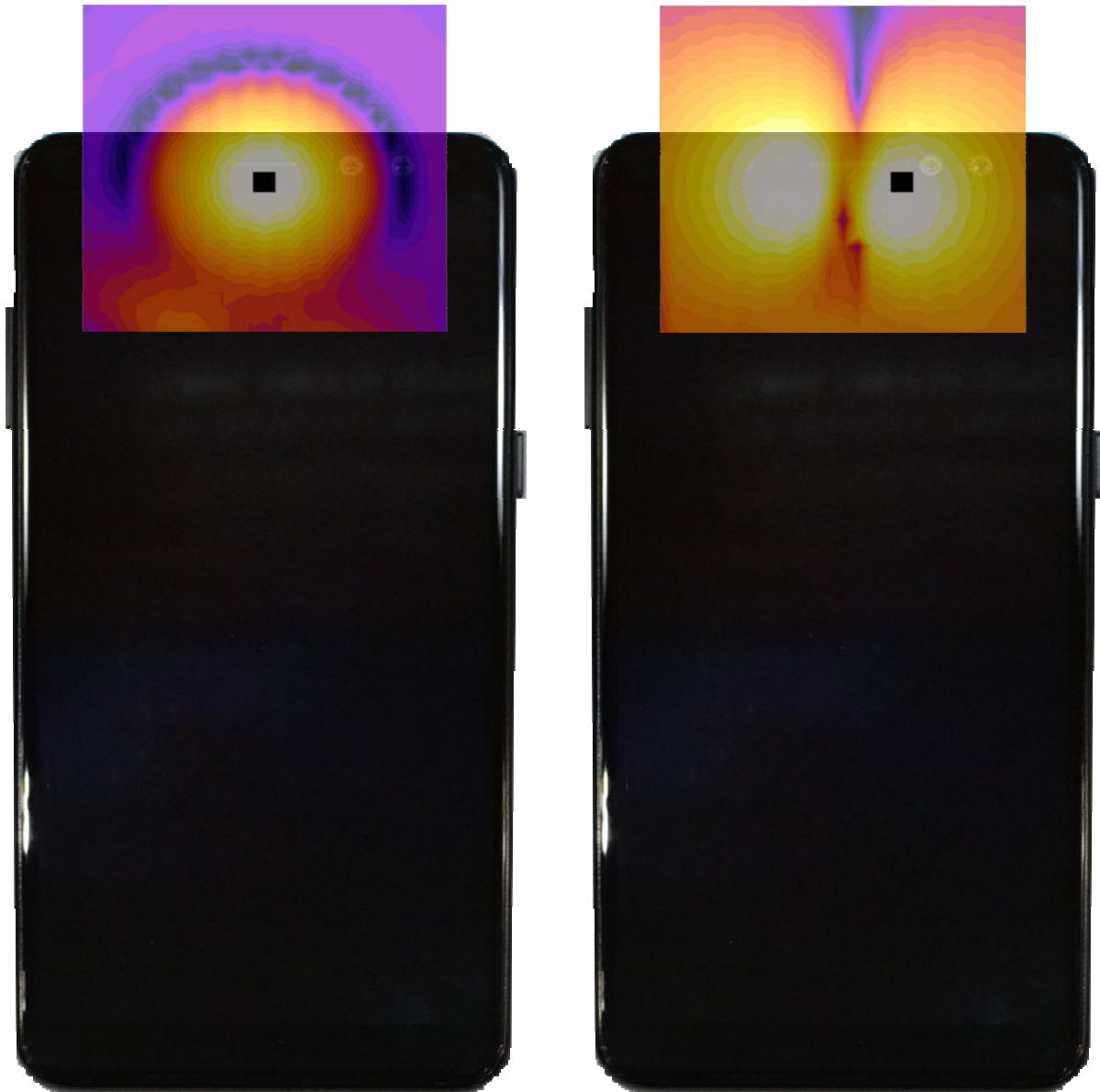
Figure 14-3 T-Coil Scan Overlay Magnetic Field Distributions
