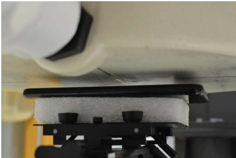
SAR Test Photo 6 – Back Side at 1.0 cm
