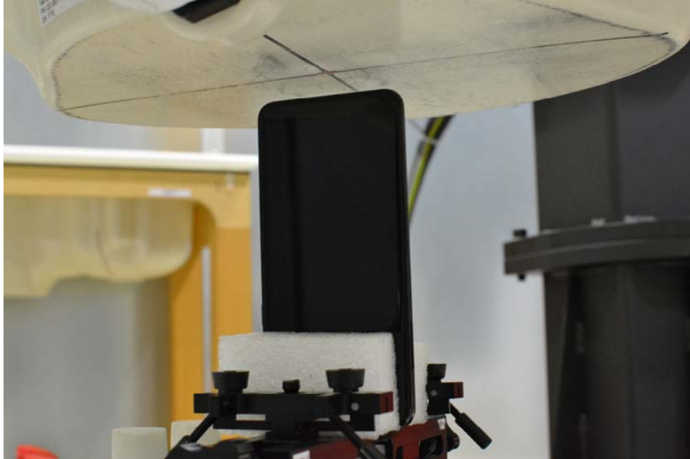
SAR Test Photo 9 – Bottom Edge at 1.0 cm
