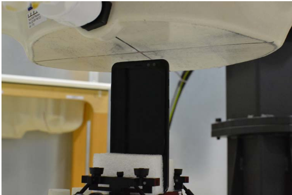
SAR Test Photo 8 – Top Edge at 1.0 cm
