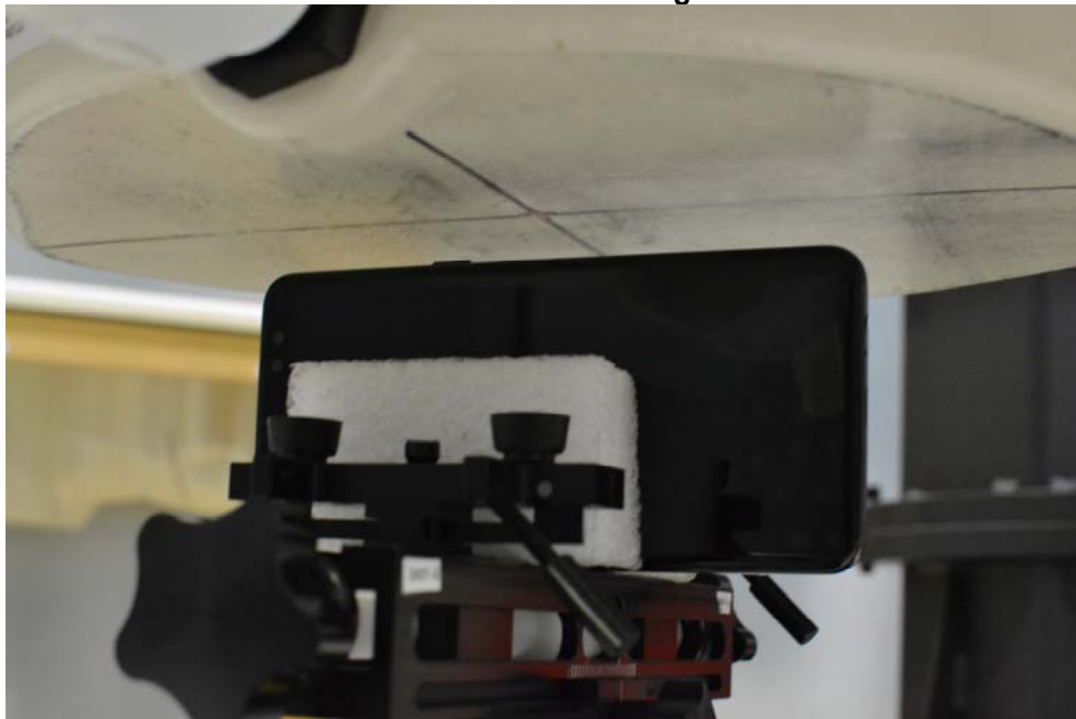
SAR Test Photo 10 – Right Edge at 1.0 cm
