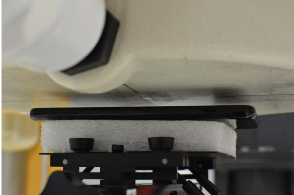
SAR Test Photo 7 – Front Side at 1.0 cm
