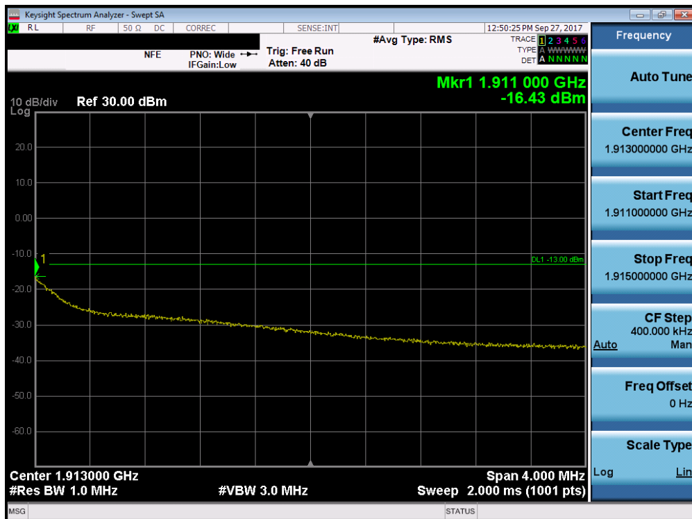
Plot 7-41. 4MHz Span Plot (PCS WCDMA Mode - High Channel)
