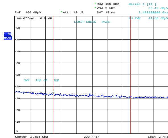
Plot 7-35. Radiated Restricted Upper Band Edge Measurement (Average)
