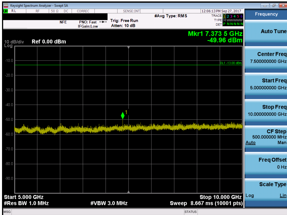
Plot 7-14. Conducted Spurious Plot (5.0MHz QPSK – RB Size 1, RB Offset 0 – High Channel)
