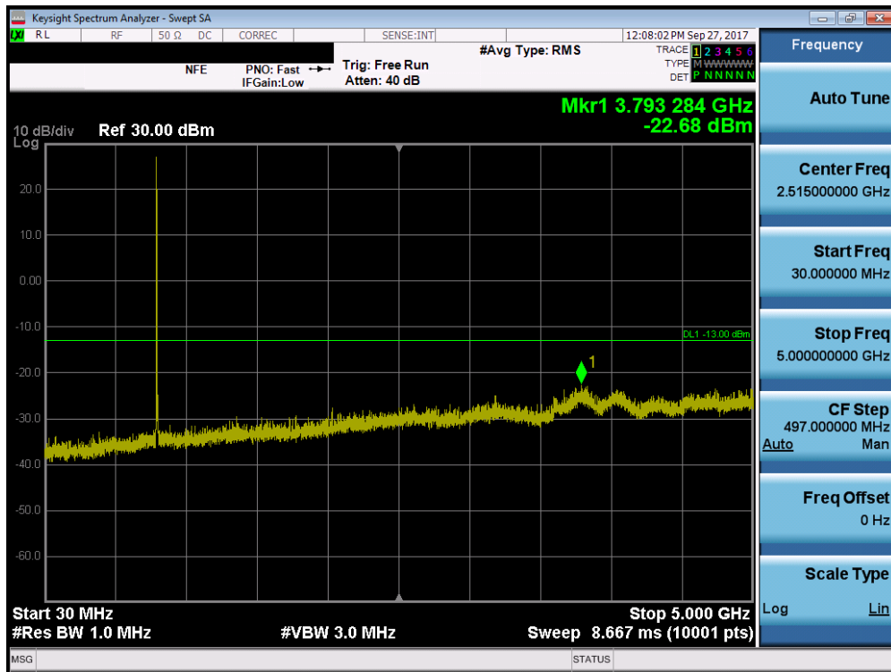
Plot 7-11. Conducted Spurious Plot (5.0MHz QPSK – RB Size 1, RB Offset 0 – Low Channel)
