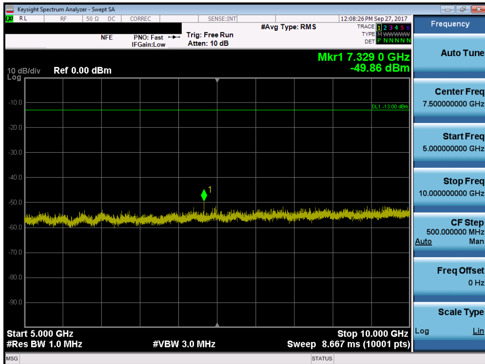
Plot 7-12. Conducted Spurious Plot 5.0MHz QPSK – RB Size 1, RB Offset 0 – Low Channel)
