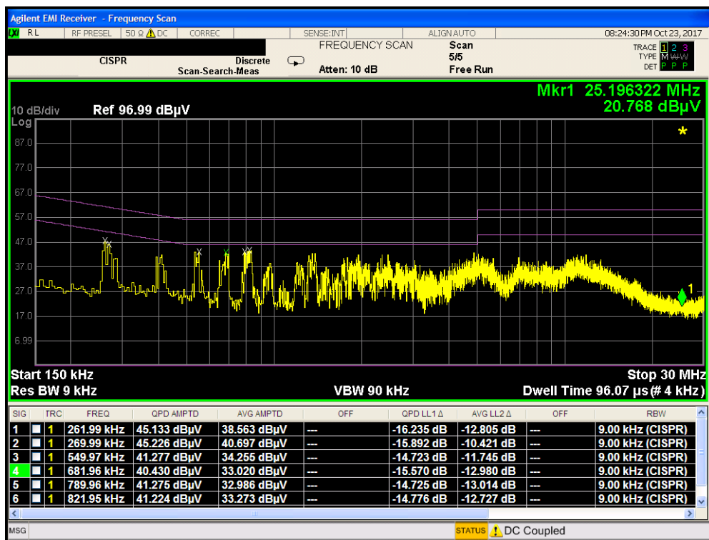
Plot 7-38. Line Conducted Plot with Bluetooth LE (N)
