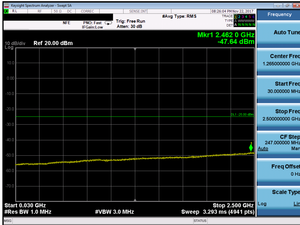
Plot 7-127. Conducted Spurious Plot (Band 7 - 10.0MHz QPSK - RB Size 1, RB Offset 0 - High Channel)
