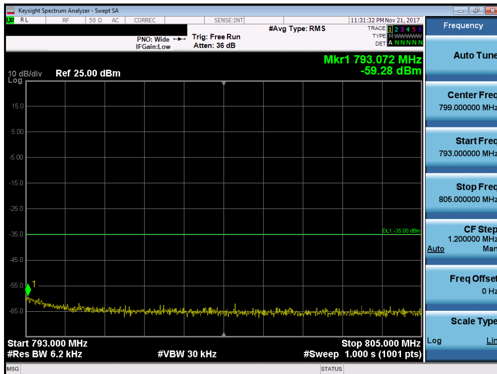
Plot 7-143. Upper Emission Mask Edge Plot (Band 13 - 5.0MHz QPSK - Full RB Configuration)
