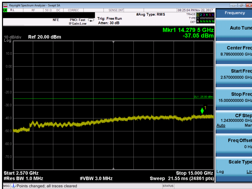
Plot 7-122. Conducted Spurious Plot (Band 7 - 10.0MHz QPSK - RB Size 1, RB Offset 0 - Low Channel)
