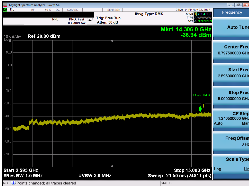
Plot 7-128. Conducted Spurious Plot (Band 7 - 10.0MHz QPSK - RB Size 1, RB Offset 0 - High Channel)
