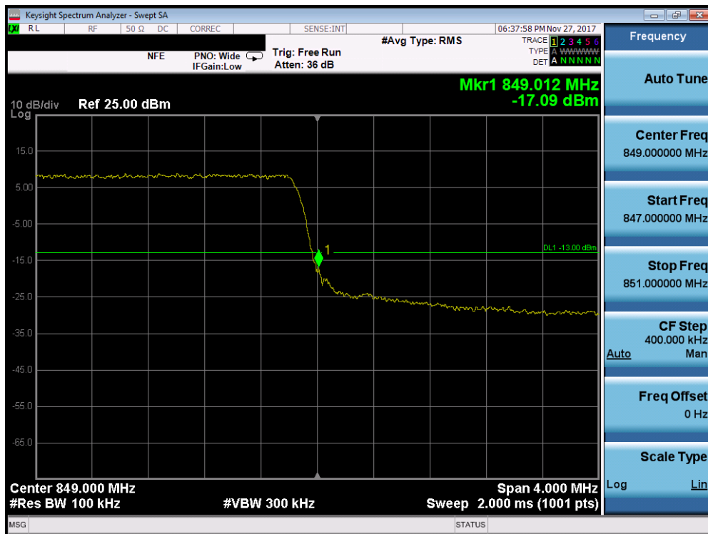
Plot 7-151. Upper Band Edge Plot (Band 26/5 - 3.0MHz QPSK - Full RB Configuration)
