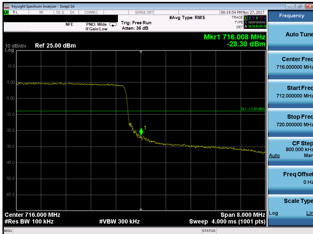
Plot 7-139. Upper Band Edge Plot (Band 12/17 - 10.0MHz QPSK - Full RB Configuration)
