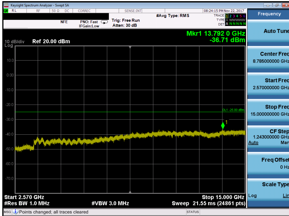
Plot 7-125. Conducted Spurious Plot (Band 7 - 10.0MHz QPSK - RB Size 1, RB Offset 0 - Mid Channel)
