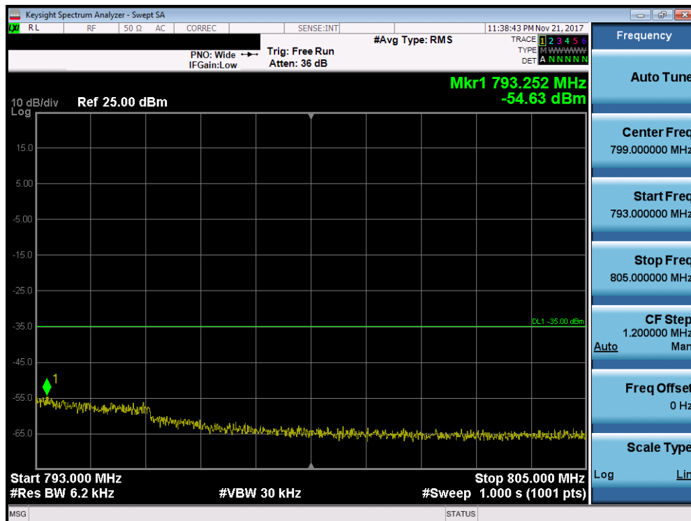
Plot 7-147. Upper Emission Mask Edge Plot (Band 13 - 10.0MHz QPSK - Full RB Configuration)
