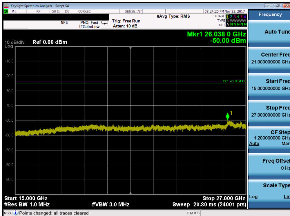
Plot 7-126. Conducted Spurious Plot (Band 7 - 10.0MHz QPSK - RB Size 1, RB Offset 0 - Mid Channel)
