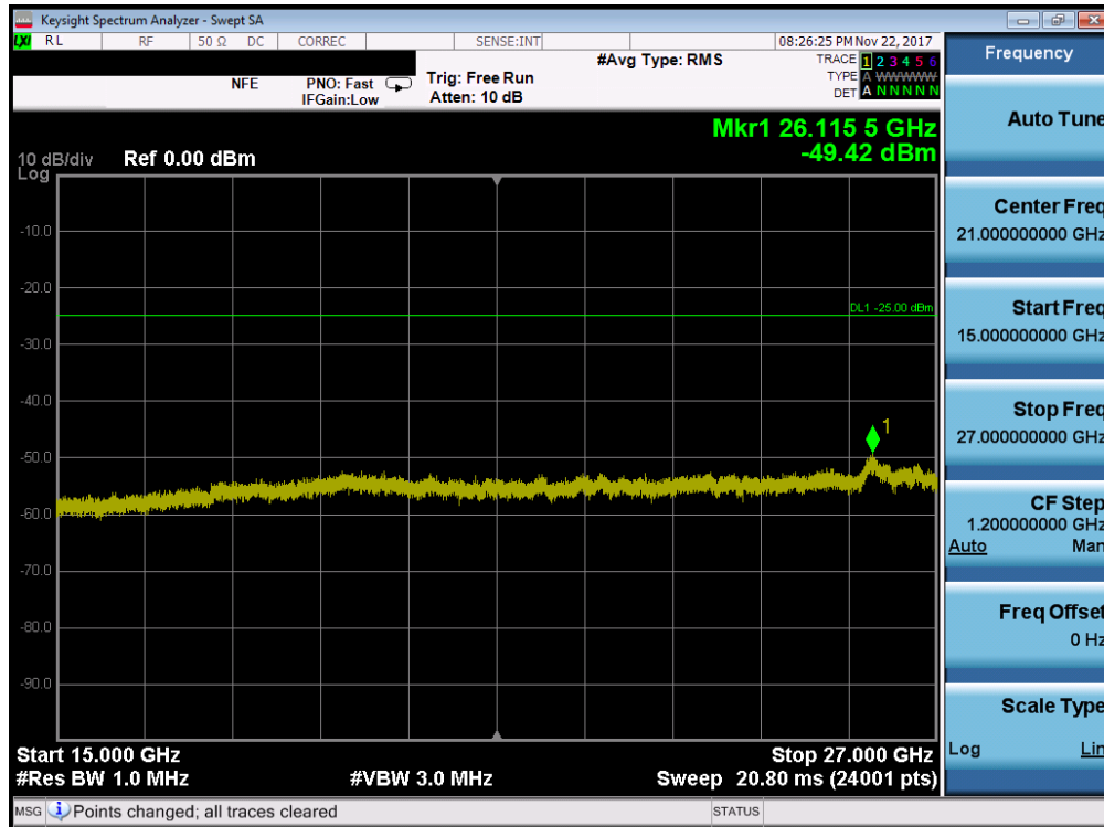
Plot 7-129. Conducted Spurious Plot (Band 7 - 10.0MHz QPSK - RB Size 1, RB Offset 0 - High Channel)
