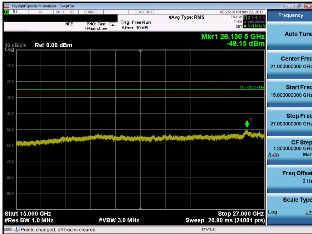
Plot 7-123. Conducted Spurious Plot (Band 7 - 10.0MHz QPSK - RB Size 1, RB Offset 0 - Low Channel)
