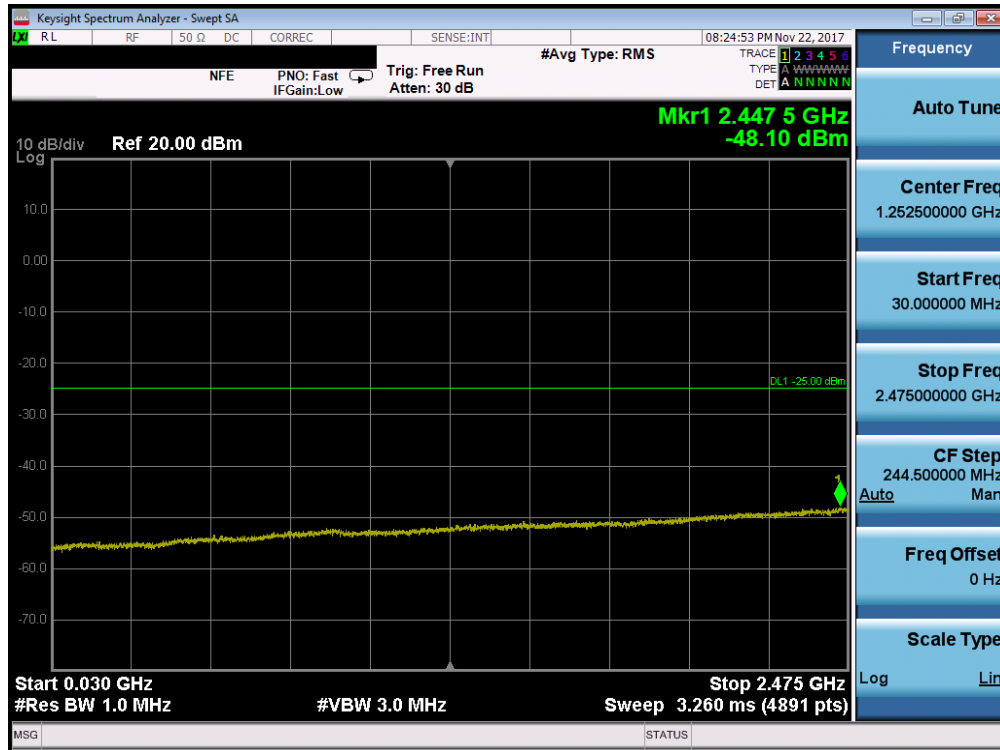
Plot 7-121. Conducted Spurious Plot (Band 7 - 10.0MHz QPSK - RB Size 1, RB Offset 0 - Low Channel)
