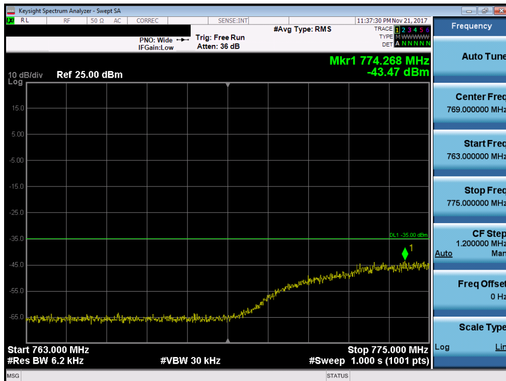
Plot 7-145. Lower Emission Mask Edge Plot (Band 13 - 10.0MHz QPSK - Full RB Configuration)
