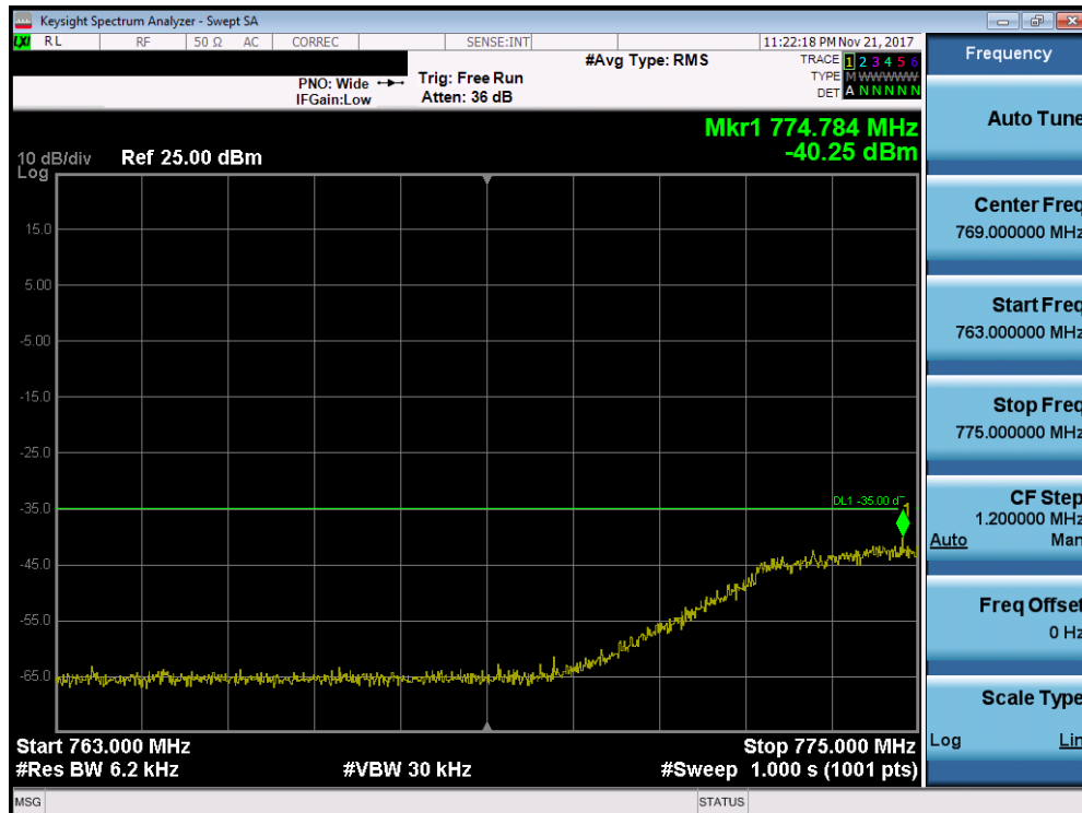
Plot 7-141. Lower Emission Mask Edge Plot (Band 13 - 5.0MHz QPSK - Full RB Configuration)
