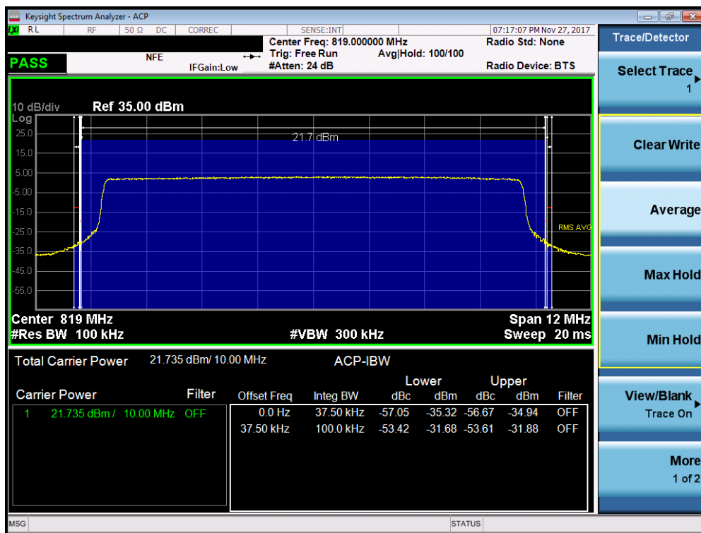
Plot 7-26. Channel Edge Plot (10MHz QPSK – RB Size 50)
