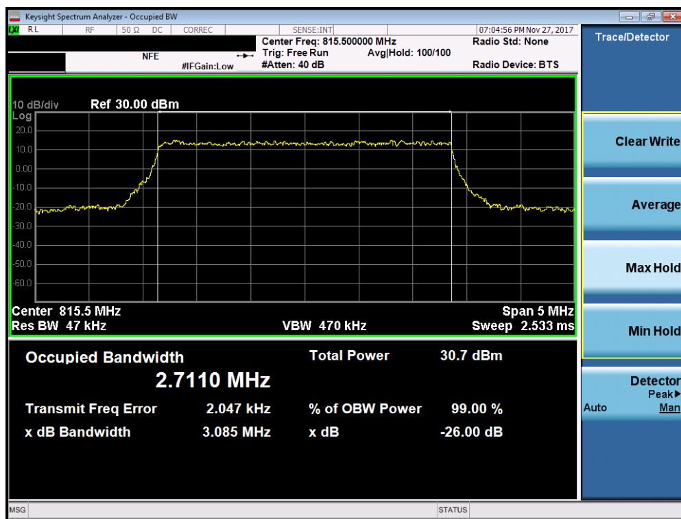
Plot 7-4. Occupied Bandwidth Plot (3MHz QPSK – RB Size 15– Low Channel)
