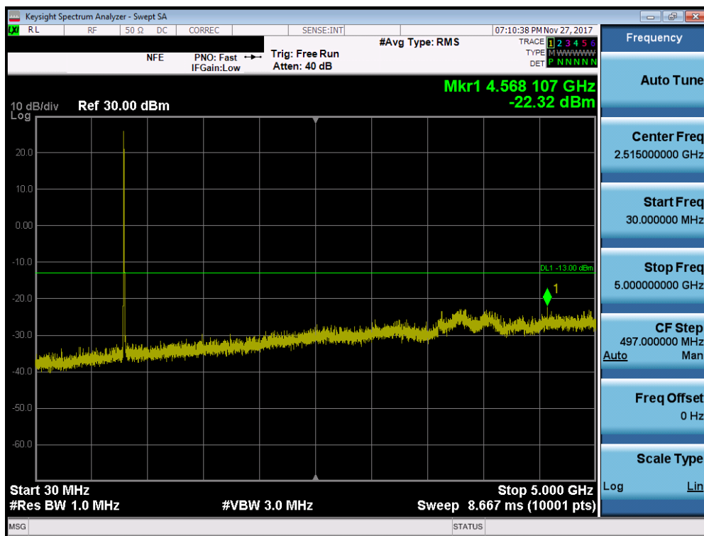
Plot 7-16. Conducted Spurious Plot (5MHz QPSK – RB Size 1, RB Offset 0 – Low Channel)
