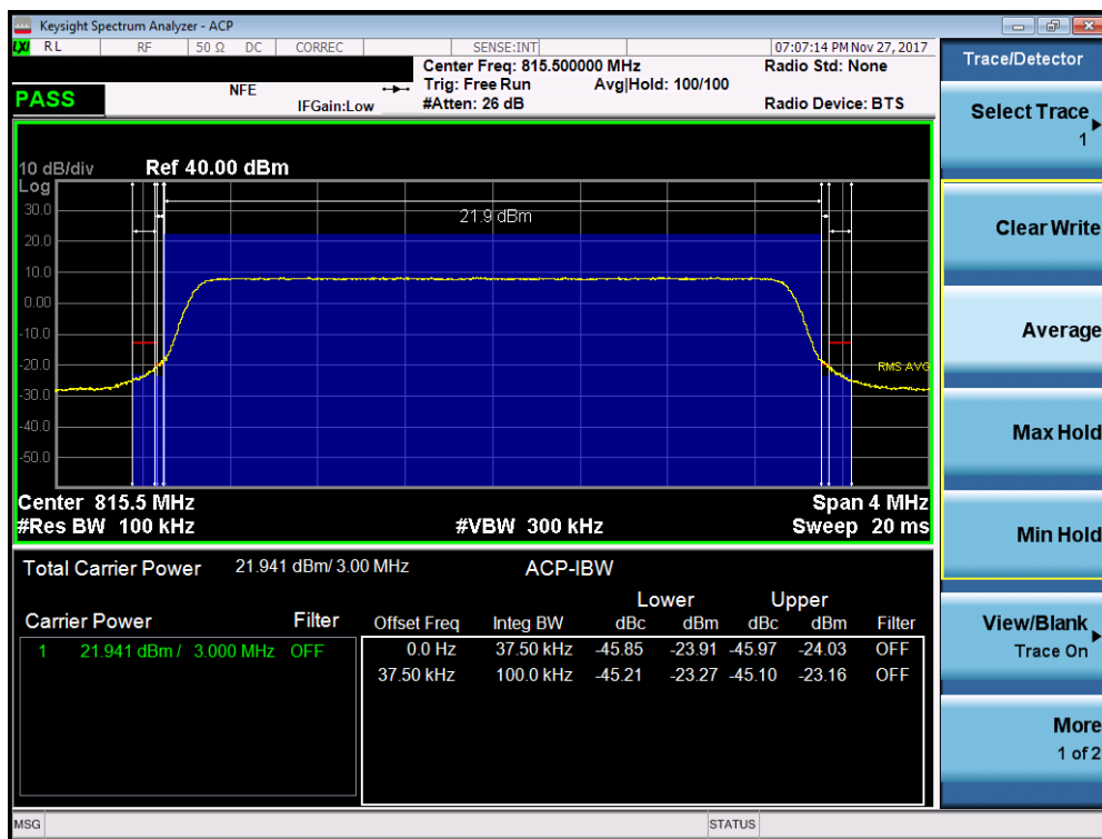
Plot 7-22. Channel Edge Plot (3MHz QPSK – RB Size 15– Low Channel)
