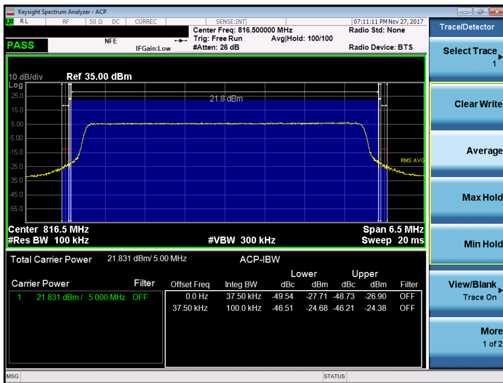
Plot 7-24. Channel Edge Plot (5MHz QPSK – RB Size 25– Low Channel)
