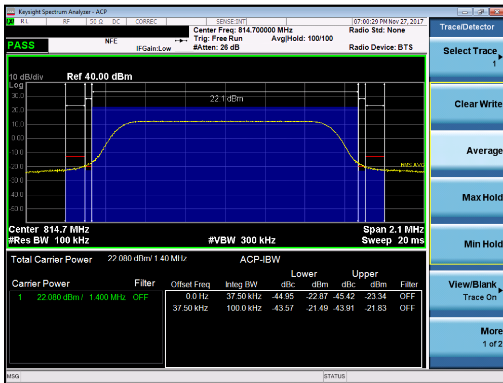
Plot 7-20. Channel Edge Plot (1.4MHz QPSK - RB Size 6- Low Channel)
