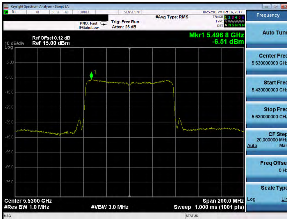
Plot 7-66. Power Spectral Density Plot (80MHz BW 802.11ac (UNII Band 2C) – Ch. 106)
