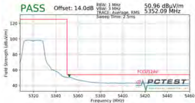
Plot 7-91. Radiated Upper Band Edge Plot (Average – UNII Band 2A)
