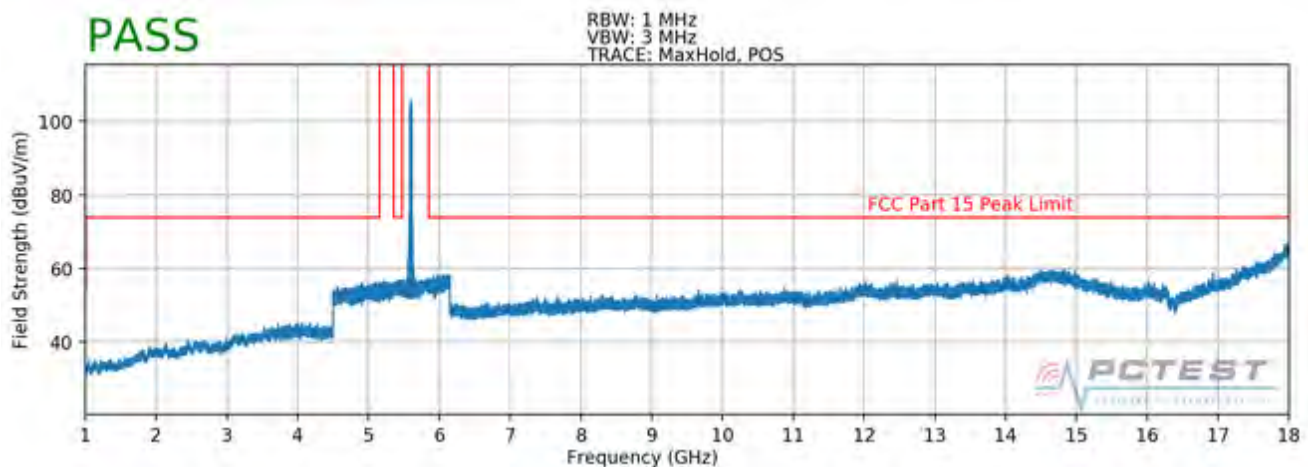
Plot 7-82. Radiated Spurious Plot above 1GHz (802.11a – U2C Ch. 116, Ant. Pol. V)
