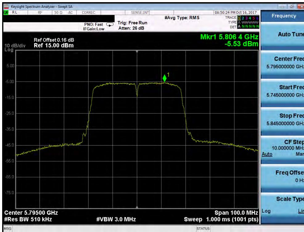
Plot 7-75. Power Spectral Density Plot (40MHz BW 802.11n (UNII Band 3) – Ch. 159)
