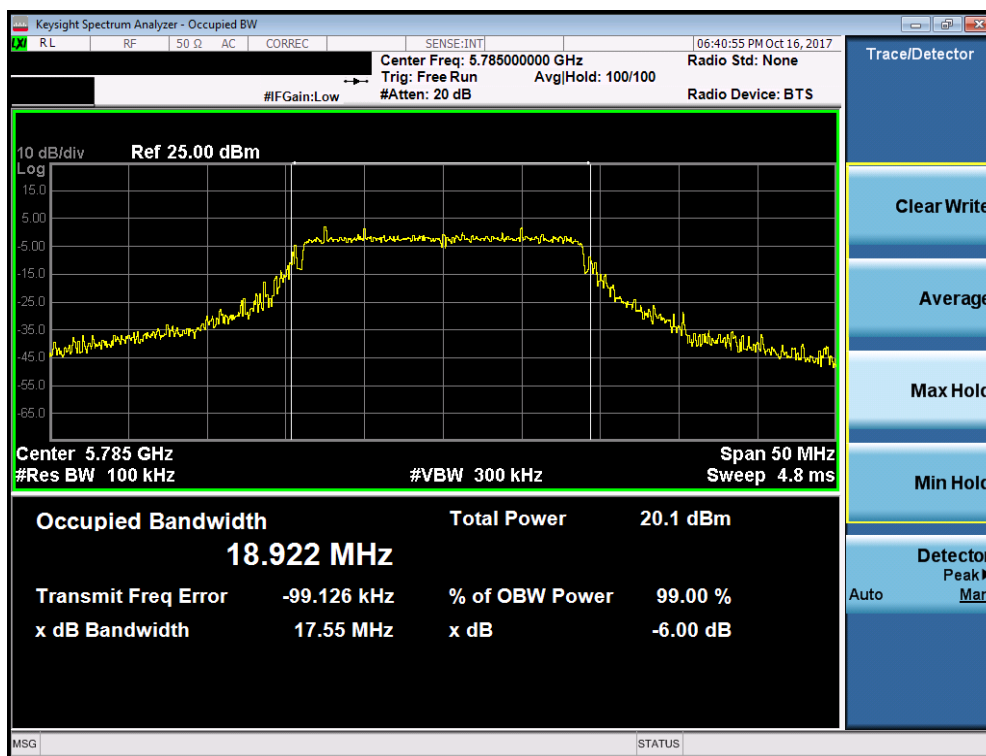
Plot 7-34. 6dB Bandwidth Plot (20MHz BW 802.11n (UNII Band 3) – Ch. 157)
