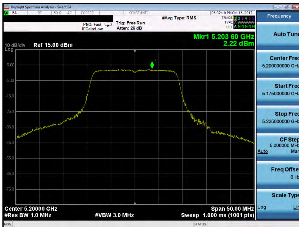
Plot 7-43. Power Spectral Density Plot (20MHz BW 802.11n (UNII Band 1) – Ch. 40)
