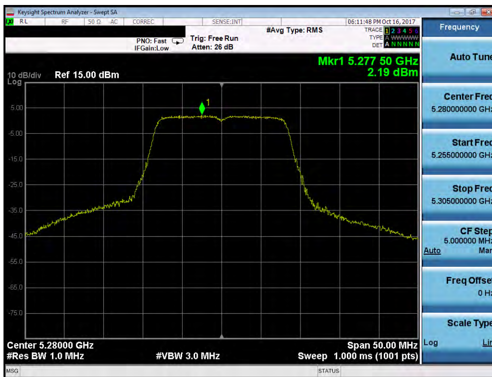
Plot 7-49. Power Spectral Density Plot (802.11a (UNII Band 2A) – Ch. 56)
