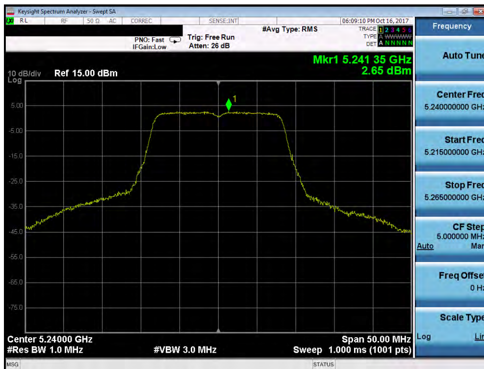
Plot 7-41. Power Spectral Density Plot (802.11a (UNII Band 1) – Ch. 48)
