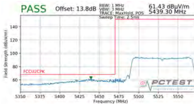
Plot 7-108. Radiated Lower Band Edge Plot (Peak – UNII Band 2C)
