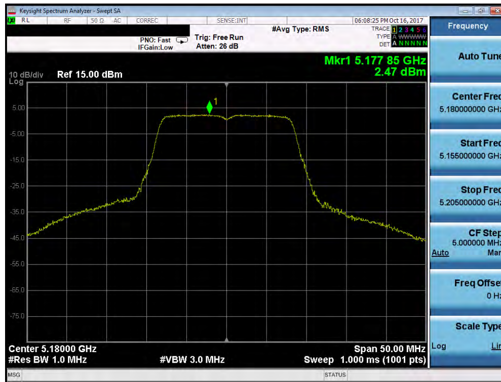
Plot 7-39. Power Spectral Density Plot (802.11a (UNII Band 1) – Ch. 36)
