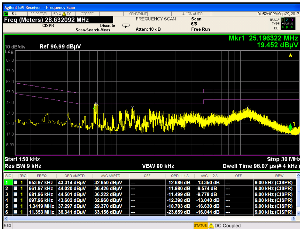
Plot 7-118. Line Conducted Plot with 802.11a UNII Band 3 (L1)
