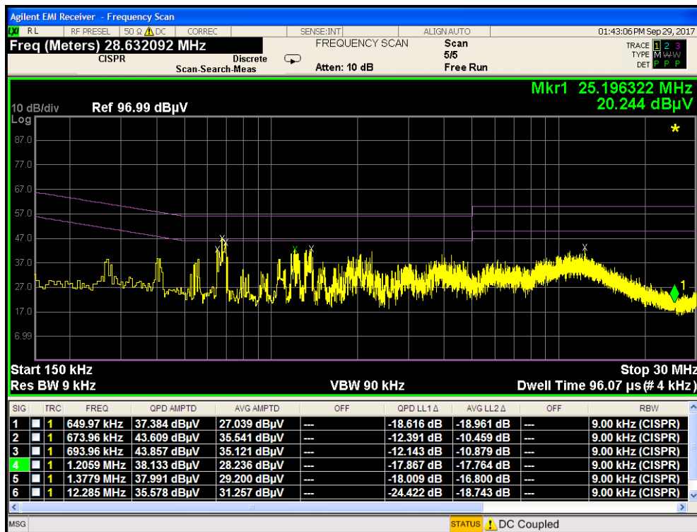
Plot 7-116. Line Conducted Plot with 802.11a UNII Band 2C (L1)
