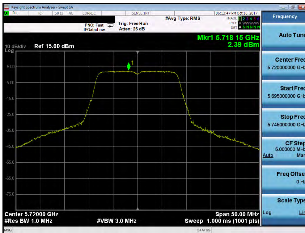
Plot 7-59. Power Spectral Density Plot (802.11a (UNII Band 2C) – Ch. 144)
