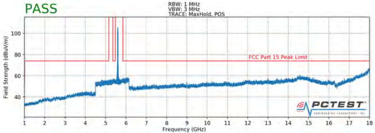
Plot 7-81. Radiated Spurious Plot above 1GHz (802.11a – U2C Ch. 116, Ant. Pol. H)
