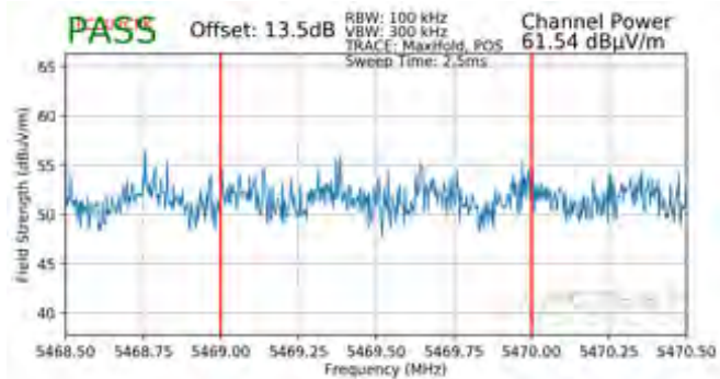
Plot 7-101. Radiated Lower Band Edge Plot (Peak – UNII Band 2C)
