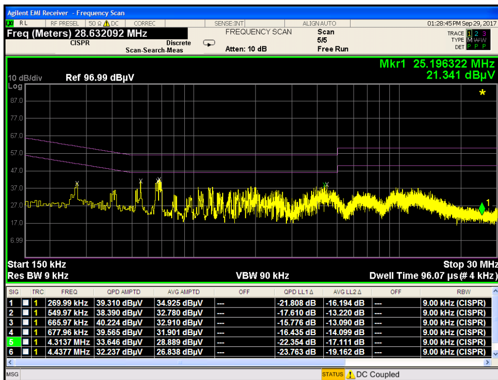
Plot 7-113. Line Conducted Plot with 802.11a UNII Band 1 (N)
