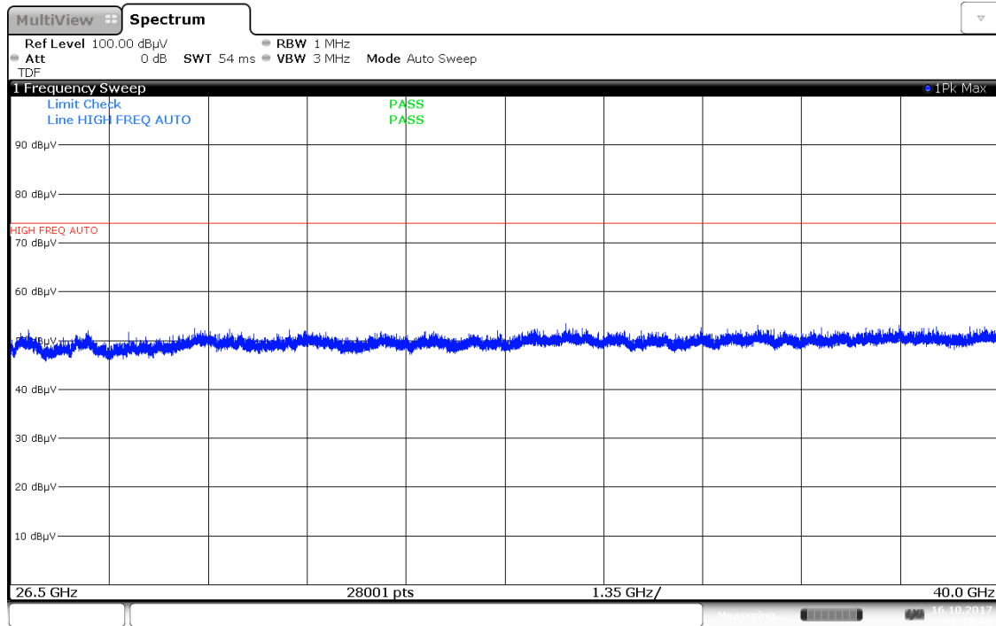
Plot 7-88. Radiated Spurious Plot above 26.5GHz - 40GHz (802.11a – Ant. Pol. V)
