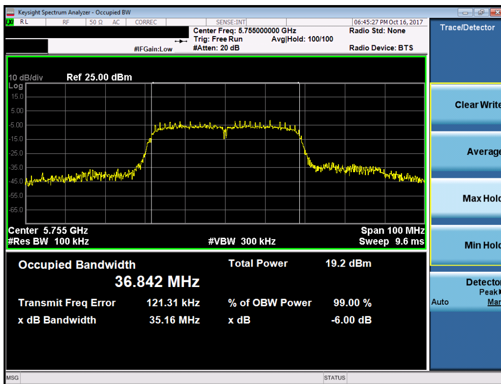
Plot 7-36. 6dB Bandwidth Plot (40MHz BW 802.11n (UNII Band 3) – Ch. 151)
