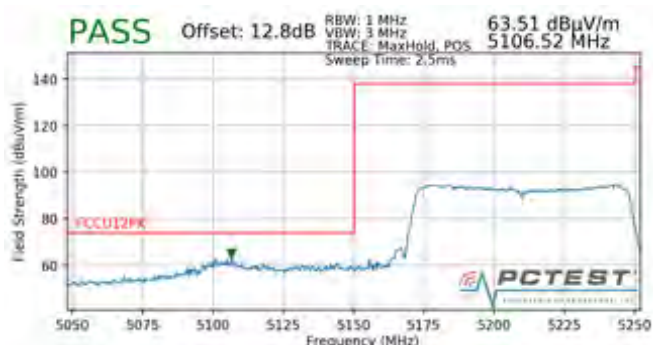
Plot 7-104. Radiated Lower Band Edge Plot (Peak – UNII Band 1)
