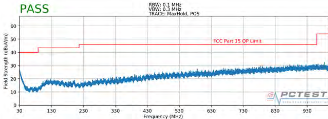
Plot 7-111. Radiated Spurious Plot below 1GHz (802.11a – U3 Ch. 157, Ant. Pol. V)
