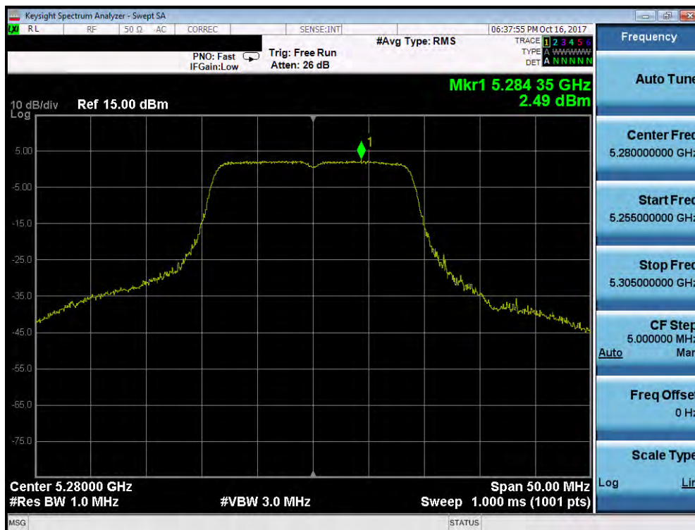
Plot 7-52. Power Spectral Density Plot (20MHz BW 802.11n (UNII Band 2A) – Ch. 56)
