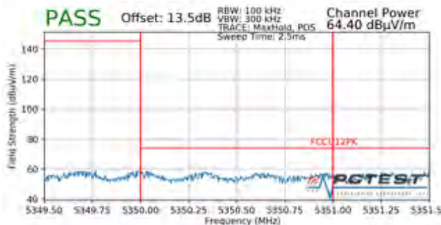
Plot 7-99. Radiated Upper Band Edge Plot (Peak – UNII Band 2A)
