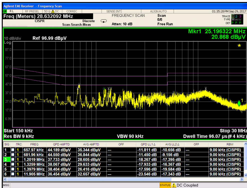
Plot 7-114. Line Conducted Plot with 802.11a UNII Band 2A (L1)
