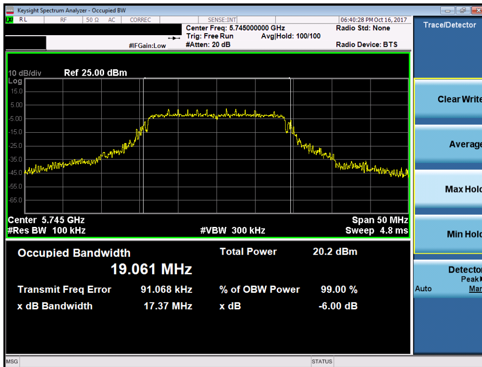
Plot 7-33. 6dB Bandwidth Plot (20MHz BW 802.11n (UNII Band 3) – Ch. 149)
