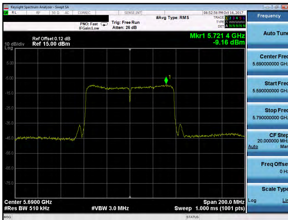
Plot 7-67. Power Spectral Density Plot (80MHz BW 802.11ac (UNII Band 2C) – Ch. 138)
