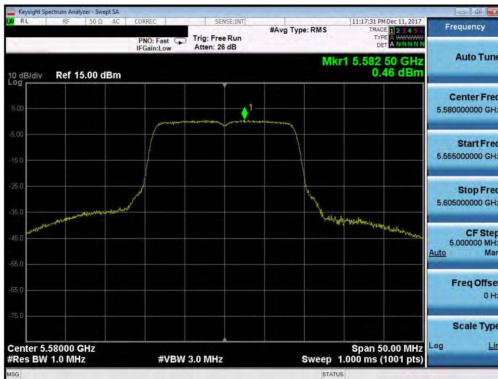
Plot 7-61. Power Spectral Density Plot (20MHz BW 802.11n (UNII Band 2C) – Ch. 116)
