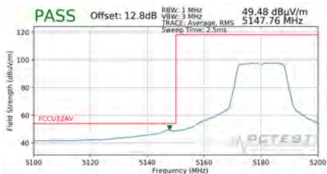
Plot 7-89. Radiated Lower Band Edge Plot (Average – UNII Band 1)
