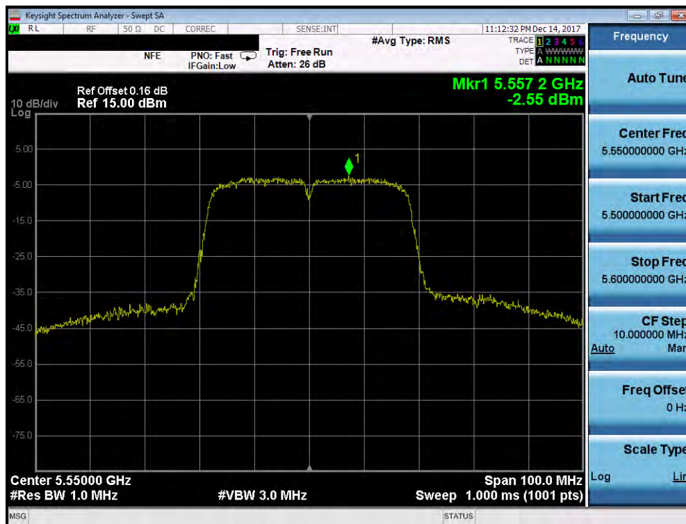
Plot 7-64. Power Spectral Density Plot (40MHz BW 802.11n (UNII Band 2C) – Ch. 110)
