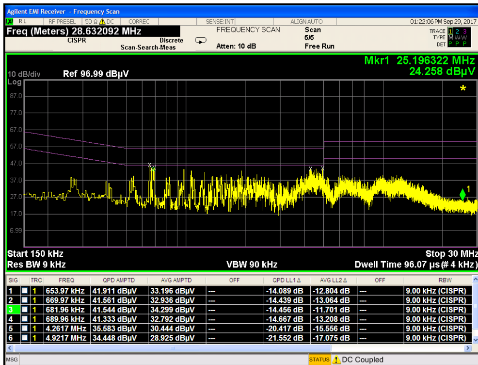
Plot 7-112. Line Conducted Plot with 802.11a UNII Band 1 (L1)
