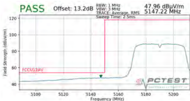
Plot 7-96. Radiated Lower Band Edge Plot (Average – UNII Band 1)
