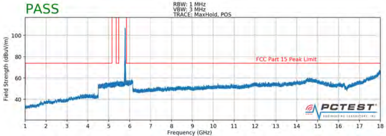
Plot 7-83. Radiated Spurious Plot above 1GHz (802.11a – U3 Ch. 157, Ant. Pol. H)
