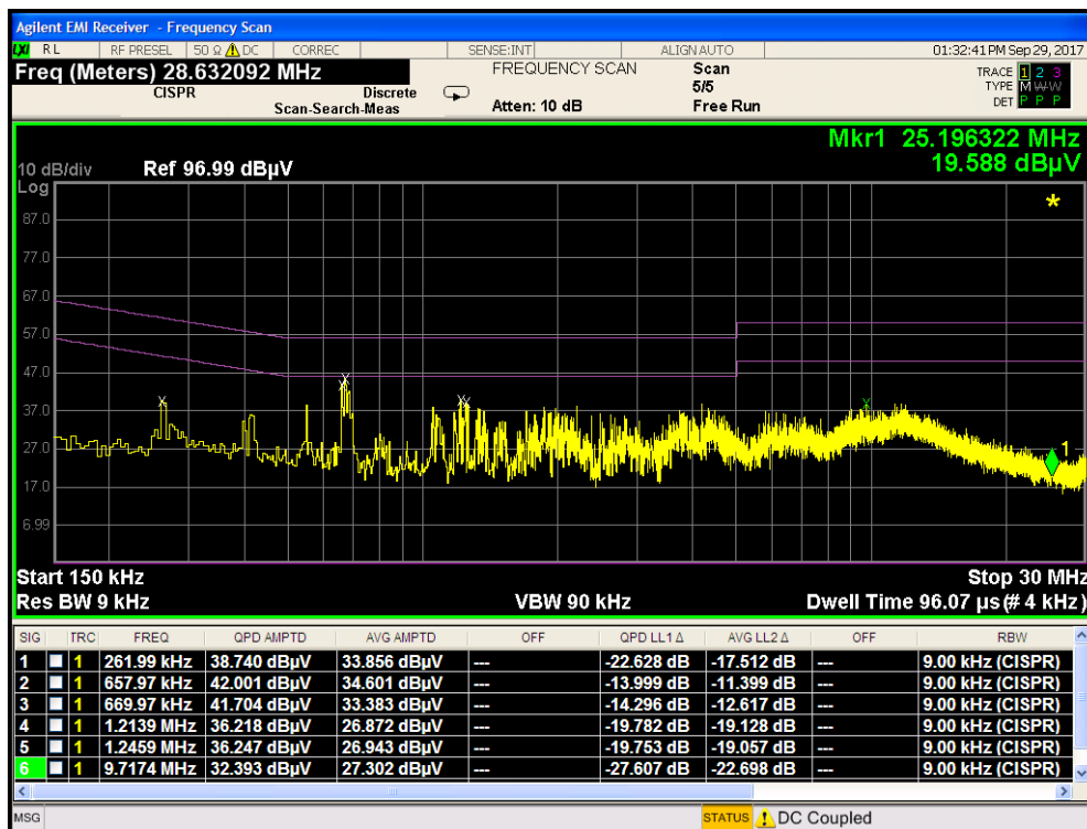
Plot 7-115. Line Conducted Plot with 802.11a UNII Band 2A (N)
