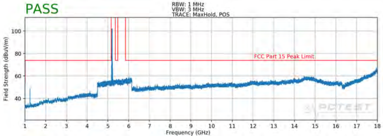
Plot 7-78. Radiated Spurious Plot above 1GHz (802.11a – U1 Ch. 40, Ant. Pol. V)
