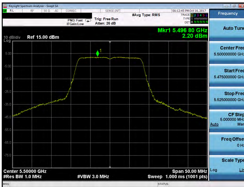
Plot 7-57. Power Spectral Density Plot (802.11a (UNII Band 2C) – Ch. 100)
