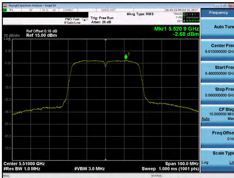
Plot 7-63. Power Spectral Density Plot (40MHz BW 802.11n (UNII Band 2C) – Ch. 102)
