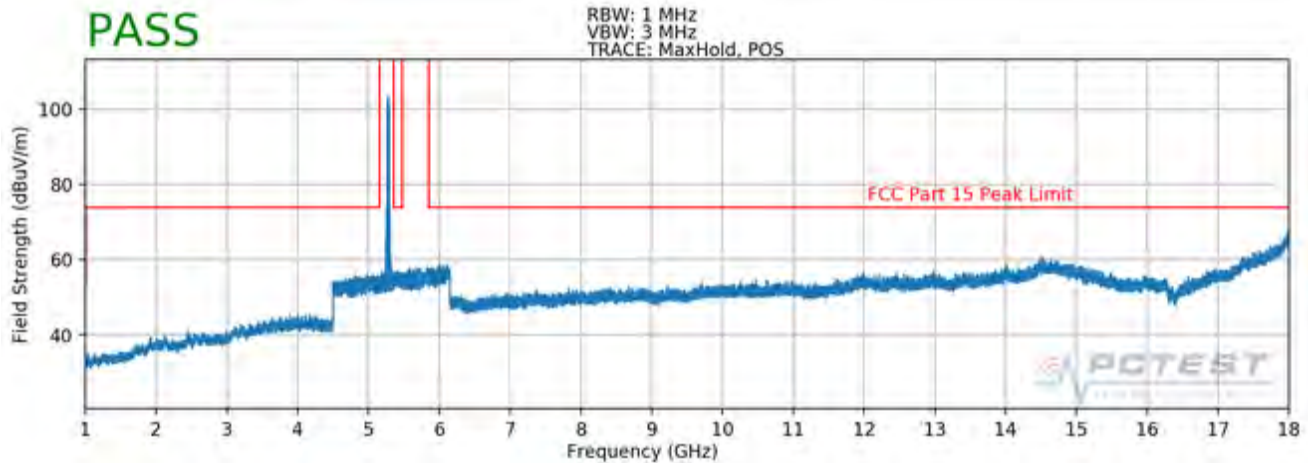
Plot 7-80. Radiated Spurious Plot above 1GHz (802.11a – U2A Ch. 56, Ant. Pol. V)
