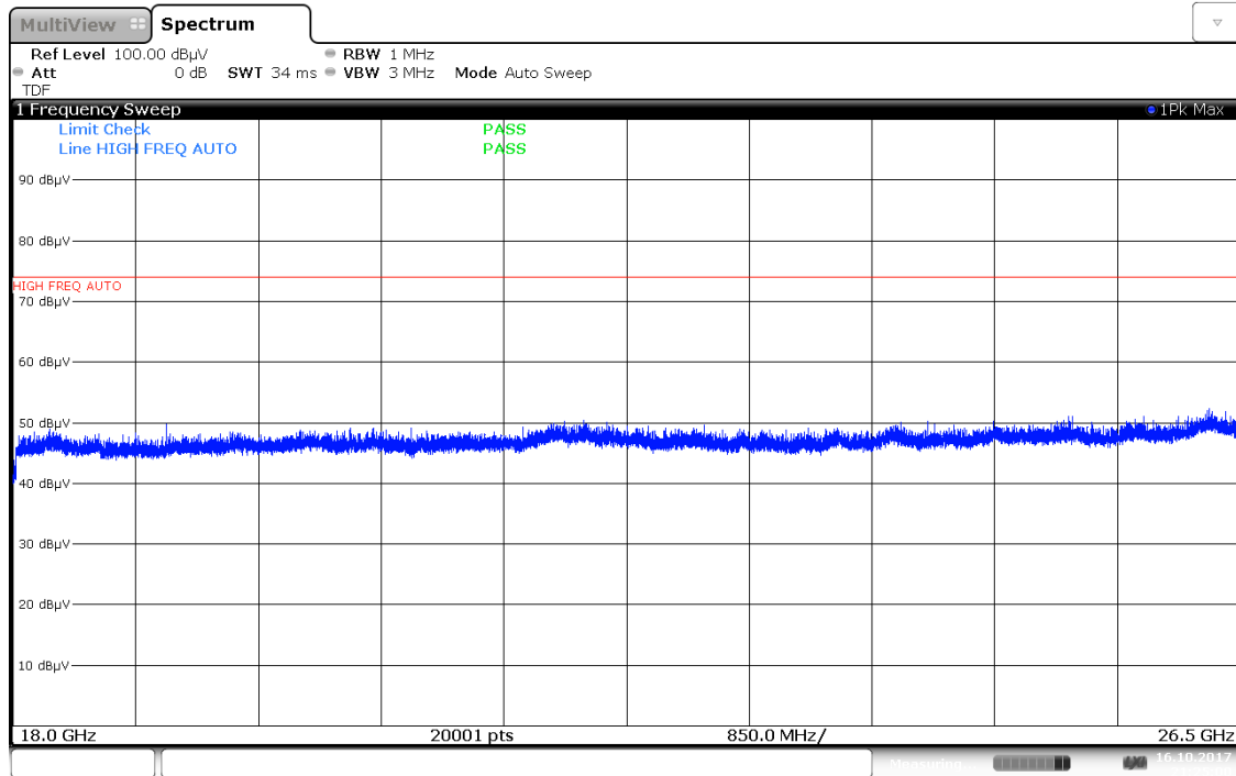
Plot 7-85. Radiated Spurious Plot 18GHz - 26.5GHz (802.11a – Ant. Pol. H)
