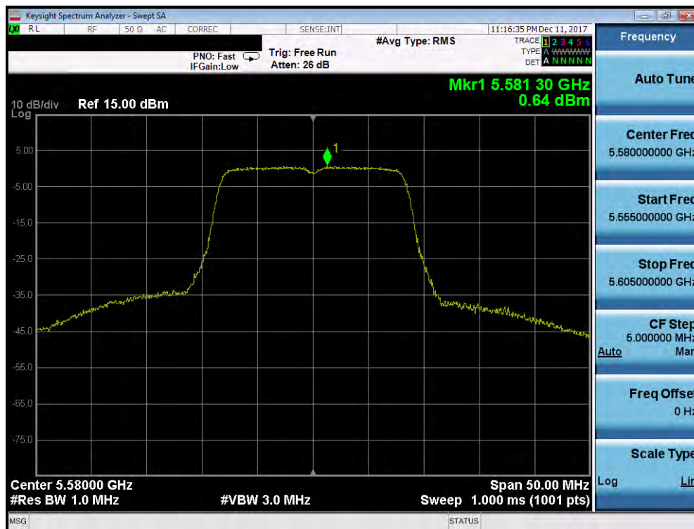
Plot 7-58. Power Spectral Density Plot (802.11a (UNII Band 2C) – Ch. 116)
