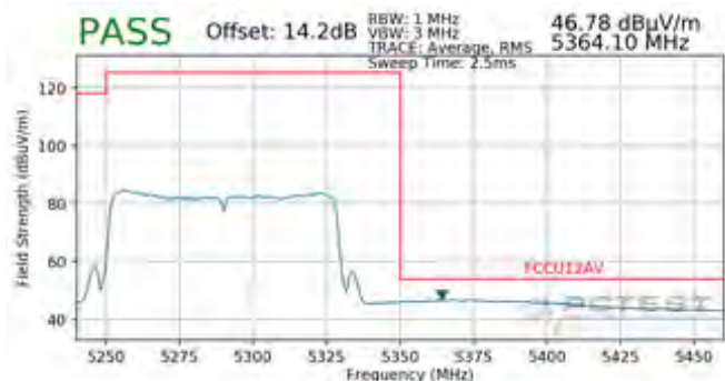
Plot 7-105. Radiated Upper Band Edge Plot (Average – UNII Band 2A)
