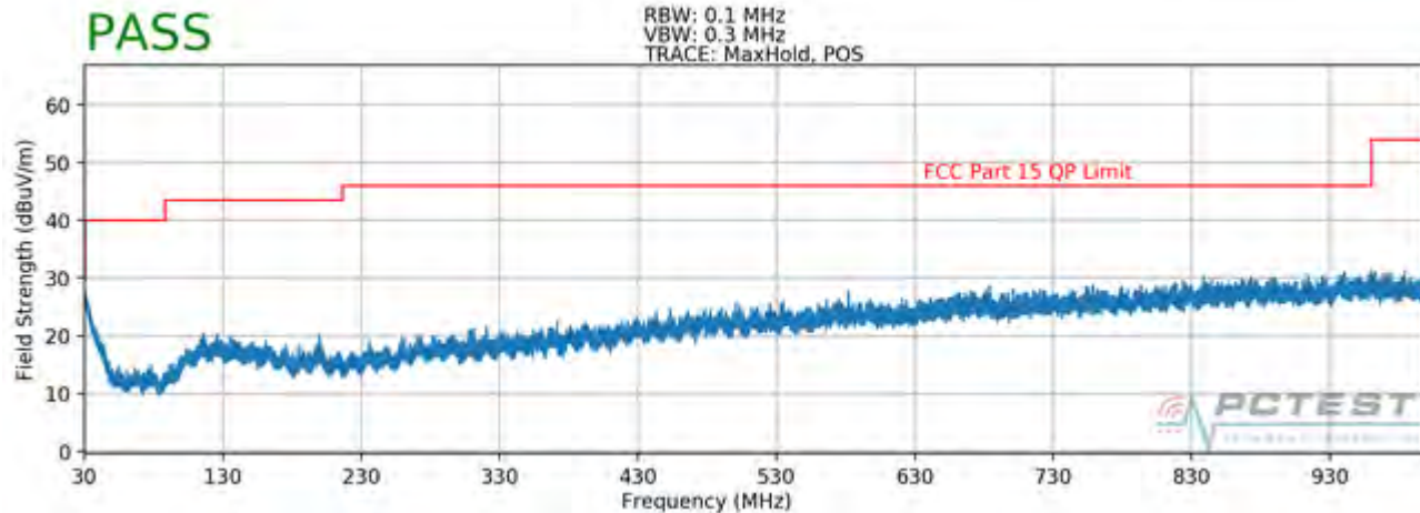
Plot 7-110. Radiated Spurious Plot below 1GHz (802.11a – U3 Ch. 157, Ant. Pol. H)
