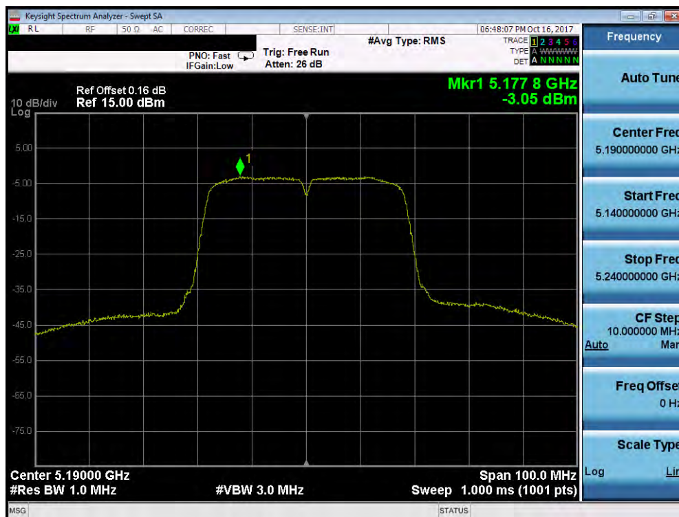
Plot 7-45. Power Spectral Density Plot (40MHz BW 802.11n (UNII Band 1) – Ch. 38)
