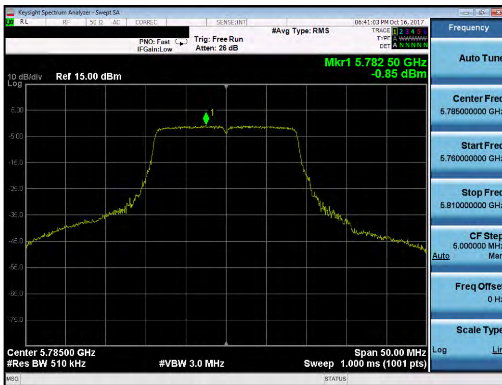
Plot 7-72. Power Spectral Density Plot (20MHz BW 802.11n (UNII Band 3) – Ch. 157)
