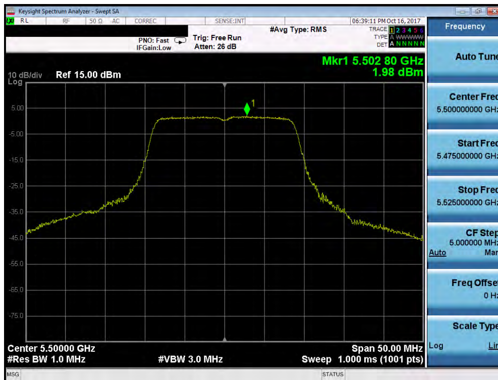
Plot 7-60. Power Spectral Density Plot (20MHz BW 802.11n (UNII Band 2C) – Ch. 100)
