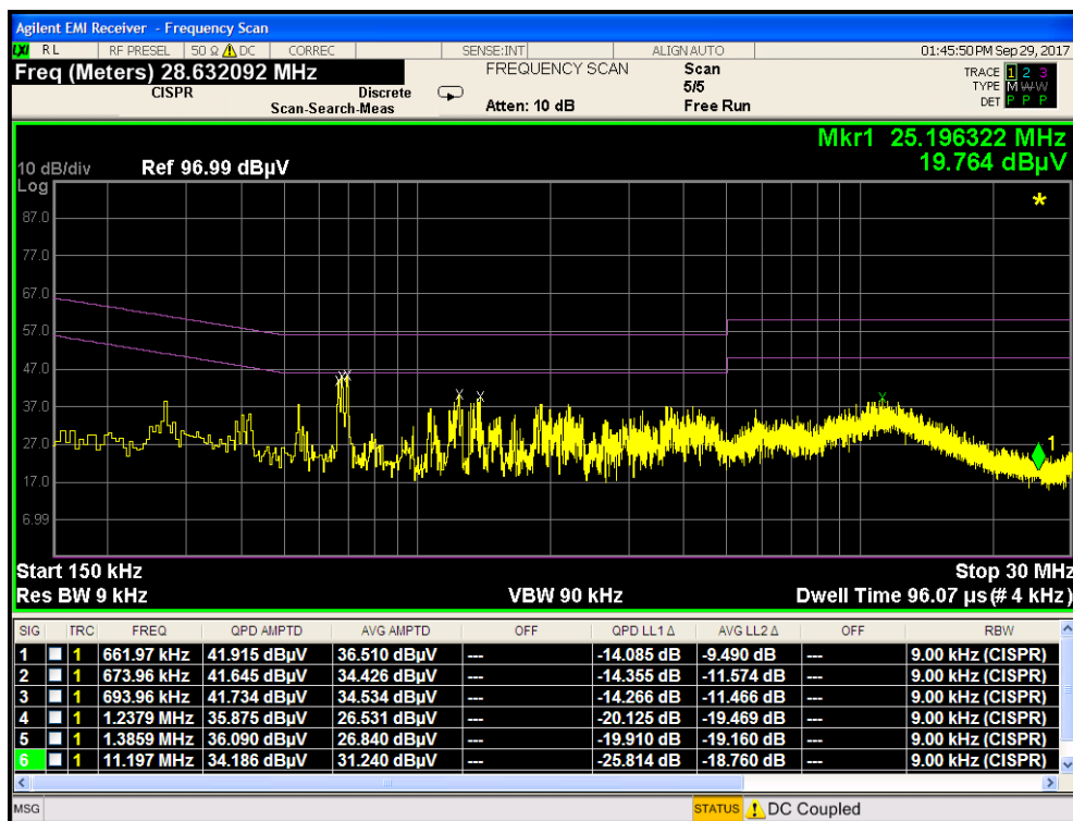
Plot 7-117. Line Conducted Plot with 802.11a UNII Band 2C (N)
