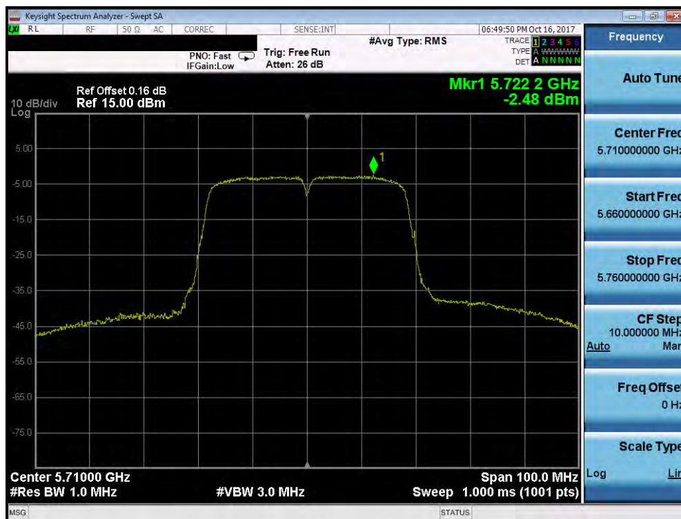
Plot 7-65. Power Spectral Density Plot (40MHz BW 802.11n (UNII Band 2C) – Ch. 142)
