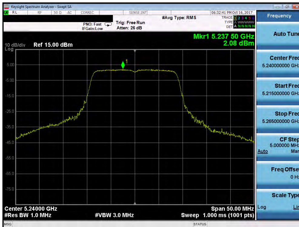
Plot 7-44. Power Spectral Density Plot (20MHz BW 802.11n (UNII Band 1) – Ch. 48)
