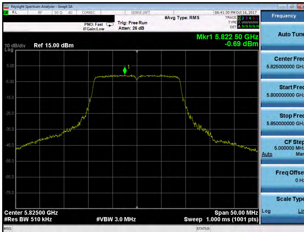
Plot 7-73. Power Spectral Density Plot (20MHz BW 802.11n (UNII Band 3) – Ch. 165)
