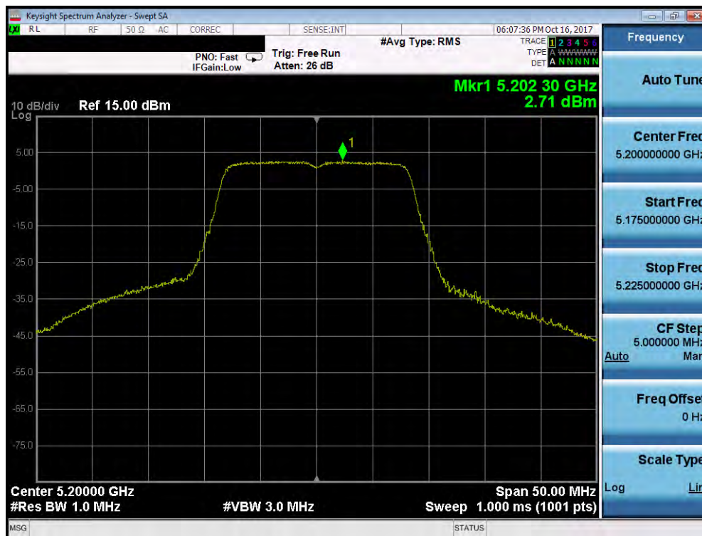
Plot 7-40. Power Spectral Density Plot (802.11a (UNII Band 1) – Ch. 40)
