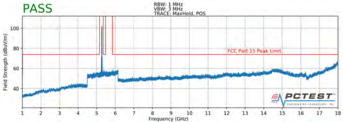
Plot 7-79. Radiated Spurious Plot above 1GHz (802.11a – U2A Ch. 56, Ant. Pol. H)
