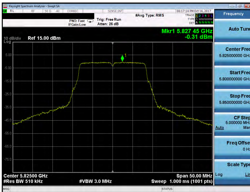
Plot 7-70. Power Spectral Density Plot (802.11a (UNII Band 3) – Ch. 165)
