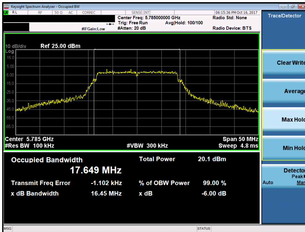
Plot 7-31. 6dB Bandwidth Plot (802.11a (UNII Band 3) – Ch. 157)
