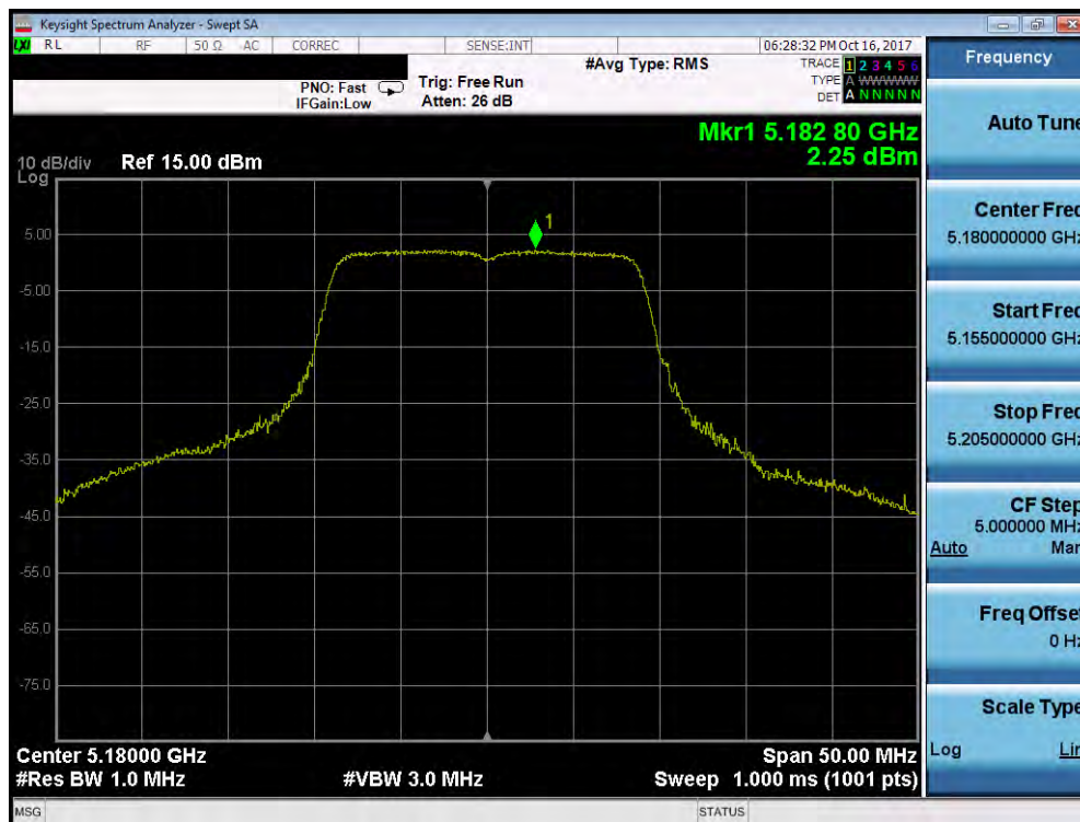
Plot 7-42. Power Spectral Density Plot (20MHz BW 802.11n (UNII Band 1) – Ch. 36)
