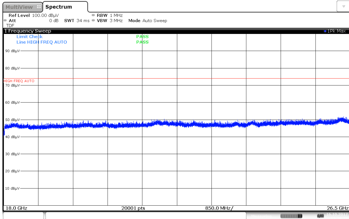
Plot 7-86. Radiated Spurious Plot above 18GHz - 26.5GHz (802.11a – Ant. Pol. V)
