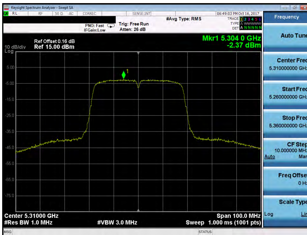
Plot 7-55. Power Spectral Density Plot (40MHz BW 802.11n (UNII Band 2A) – Ch. 62)
