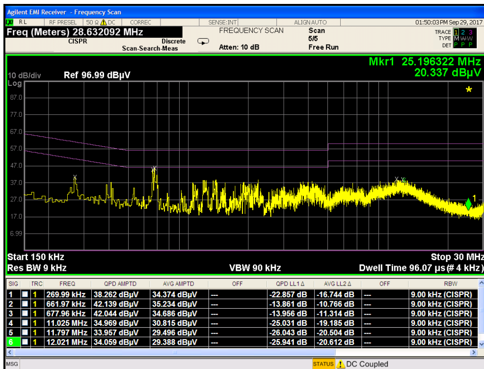
Plot 7-119. Line Conducted Plot with 802.11a UNII Band 3 (N)
