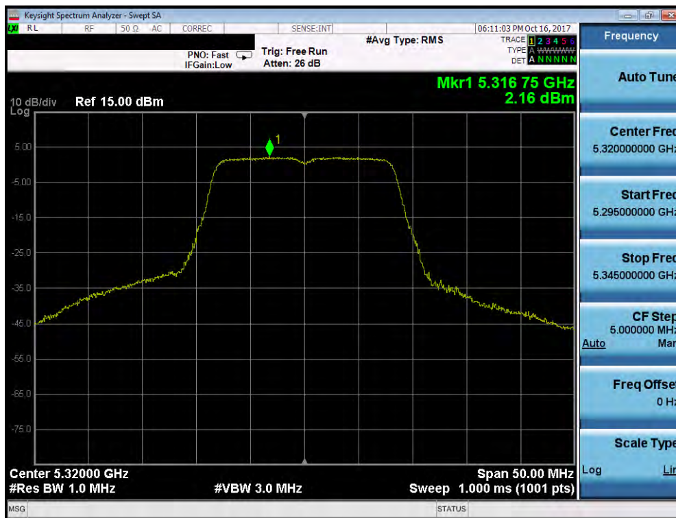
Plot 7-50. Power Spectral Density Plot (802.11a (UNII Band 2A) – Ch. 64)
