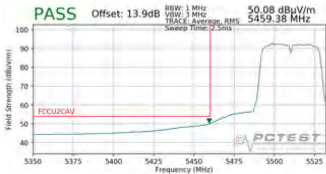
Plot 7-100. Radiated Lower Band Edge Plot (Average – UNII Band 2C)
