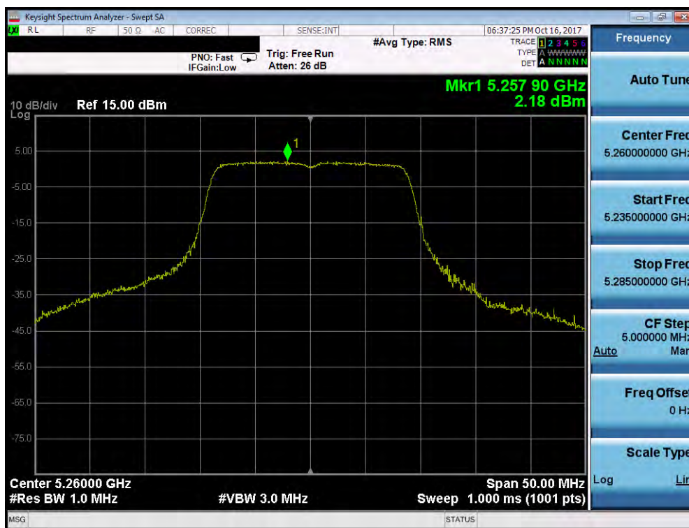
Plot 7-51. Power Spectral Density Plot (20MHz BW 802.11n (UNII Band 2A) – Ch. 52)
