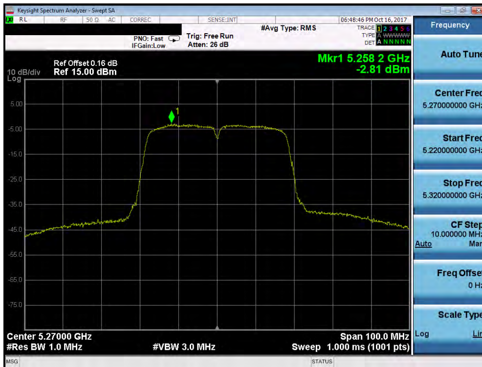
Plot 7-54. Power Spectral Density Plot (40MHz BW 802.11n (UNII Band 2A) – Ch. 54)
