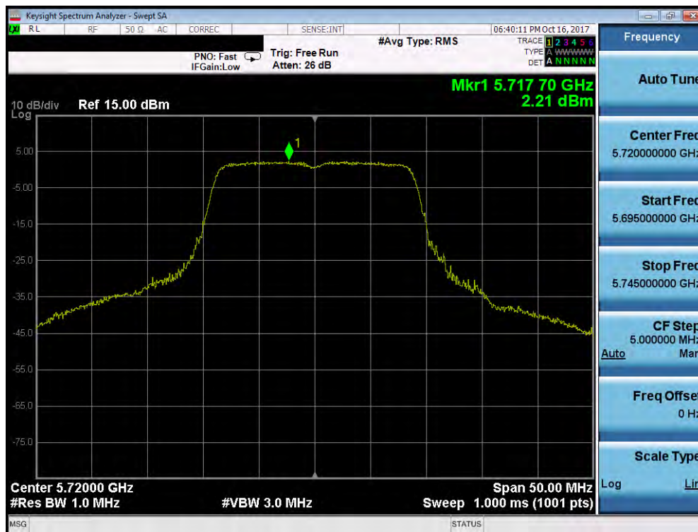
Plot 7-62. Power Spectral Density Plot (20MHz BW 802.11n (UNII Band 2C) – Ch. 144)
