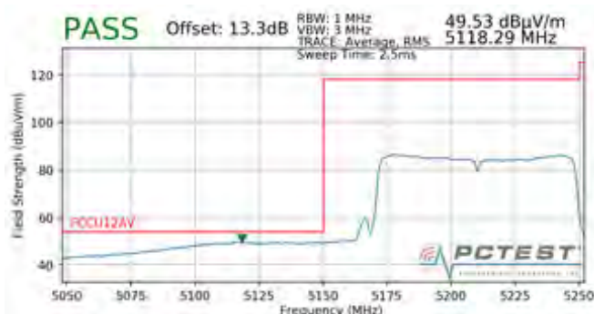
Plot 7-103. Radiated Lower Band Edge Plot (Average – UNII Band 1)
