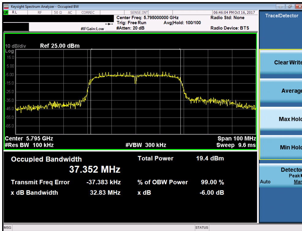
Plot 7-37. 6dB Bandwidth Plot (40MHz BW 802.11n (UNII Band 3) – Ch. 159)
