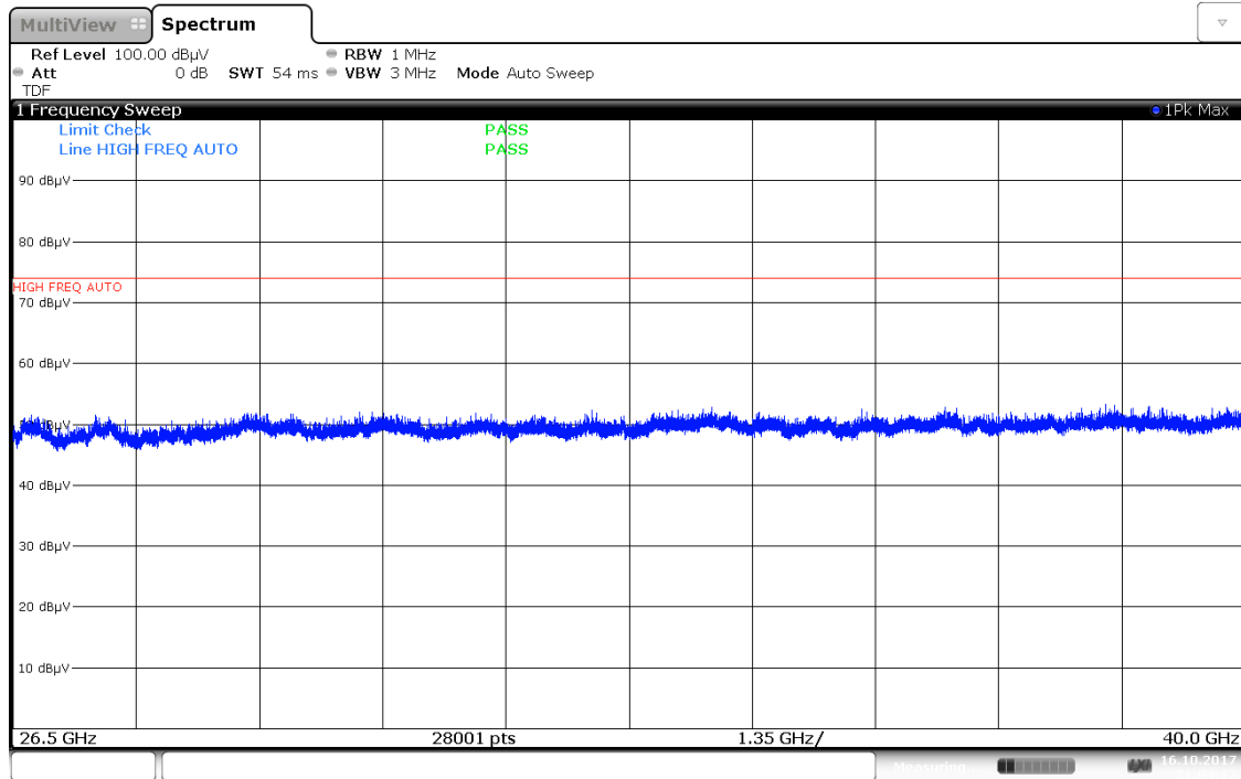
Plot 7-87. Radiated Spurious Plot 26.5GHz - 40GHz (802.11a – Ant. Pol. H)
