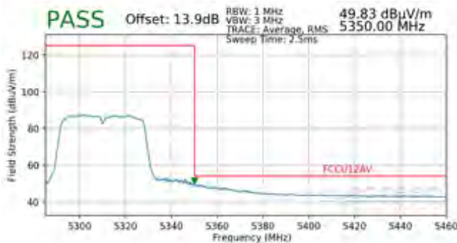
Plot 7-98. Radiated Upper Band Edge Plot (Average – UNII Band 2A)
