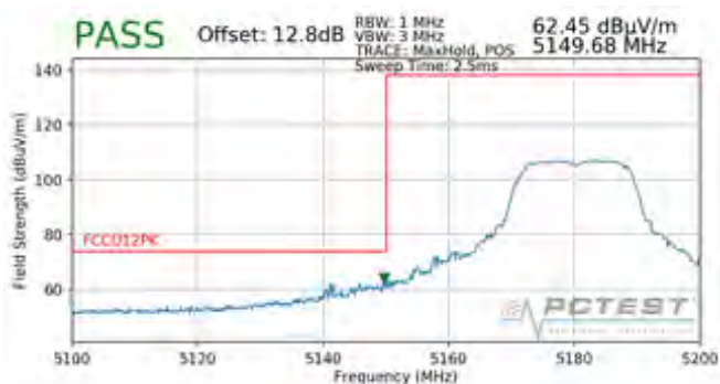
Plot 7-90. Radiated Lower Band Edge Plot (Peak – UNII Band 1)
