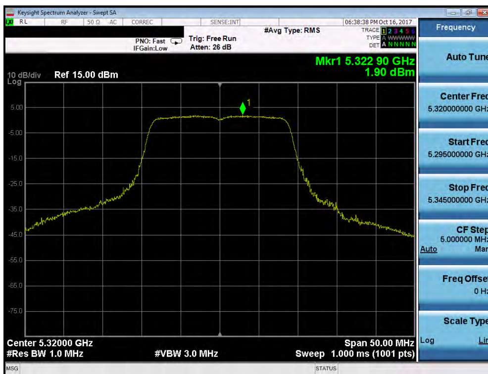
Plot 7-53. Power Spectral Density Plot (20MHz BW 802.11n (UNII Band 2A) – Ch. 64)
