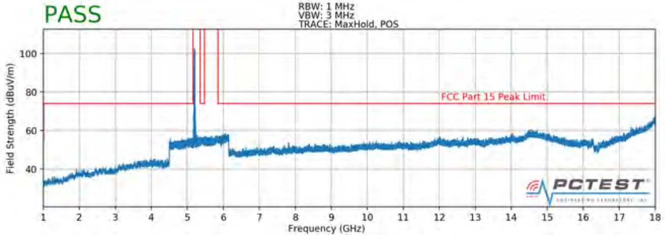
Plot 7-77. Radiated Spurious Plot above 1GHz (802.11a – U1 Ch. 40, Ant. Pol. H)
