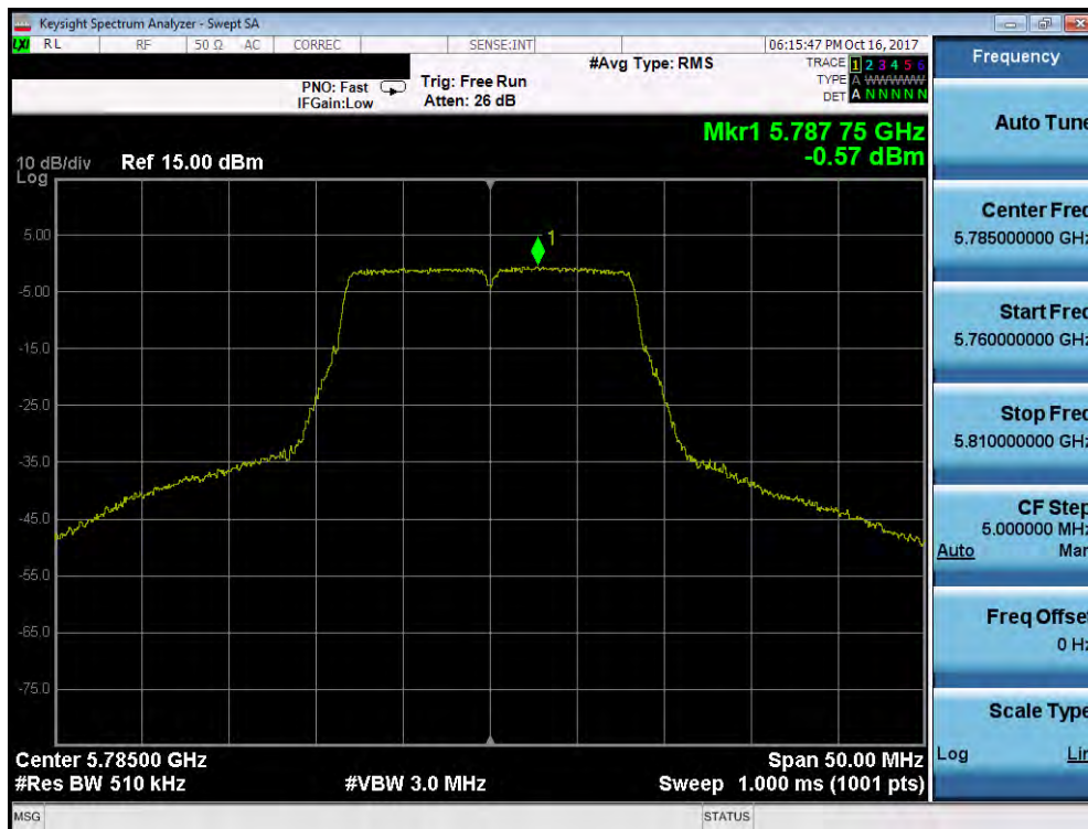
Plot 7-69. Power Spectral Density Plot (802.11a (UNII Band 3) – Ch. 157)
