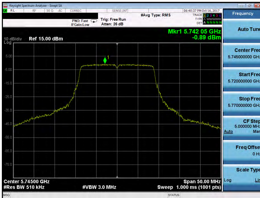
Plot 7-71. Power Spectral Density Plot (20MHz BW 802.11n (UNII Band 3) – Ch. 149)
