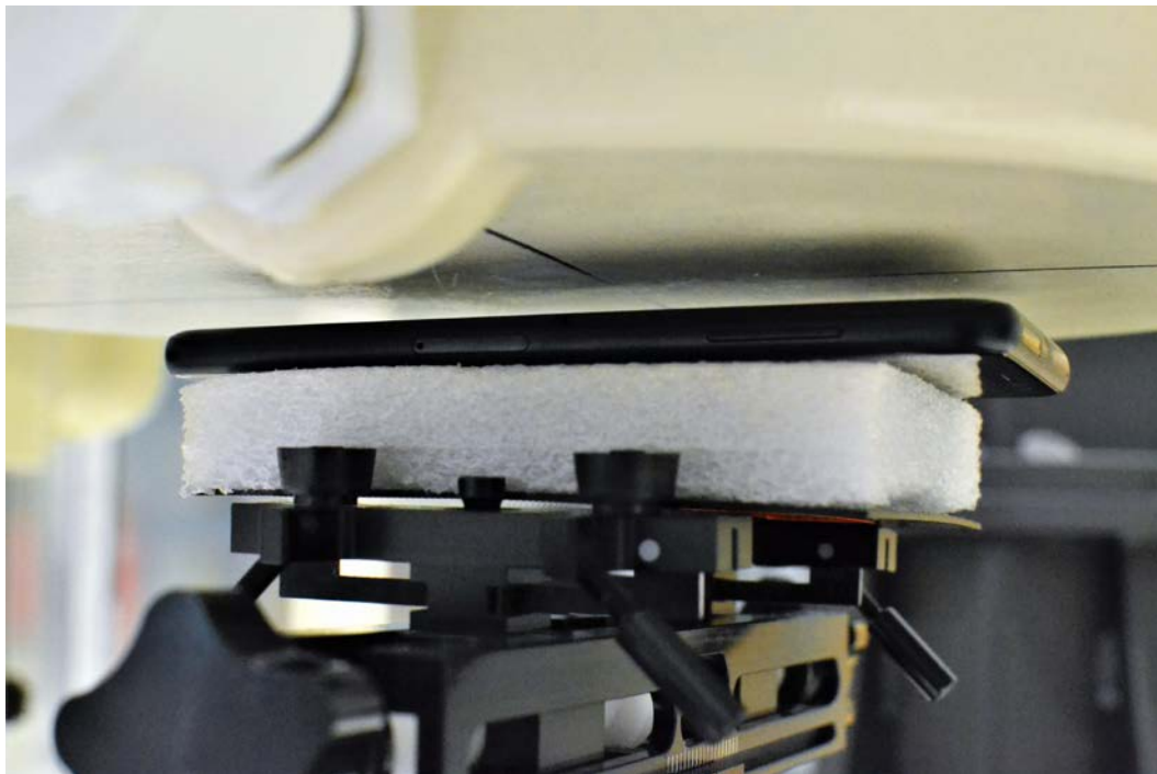
SAR Test Photo 6 – Back Side at 1.0 cm
