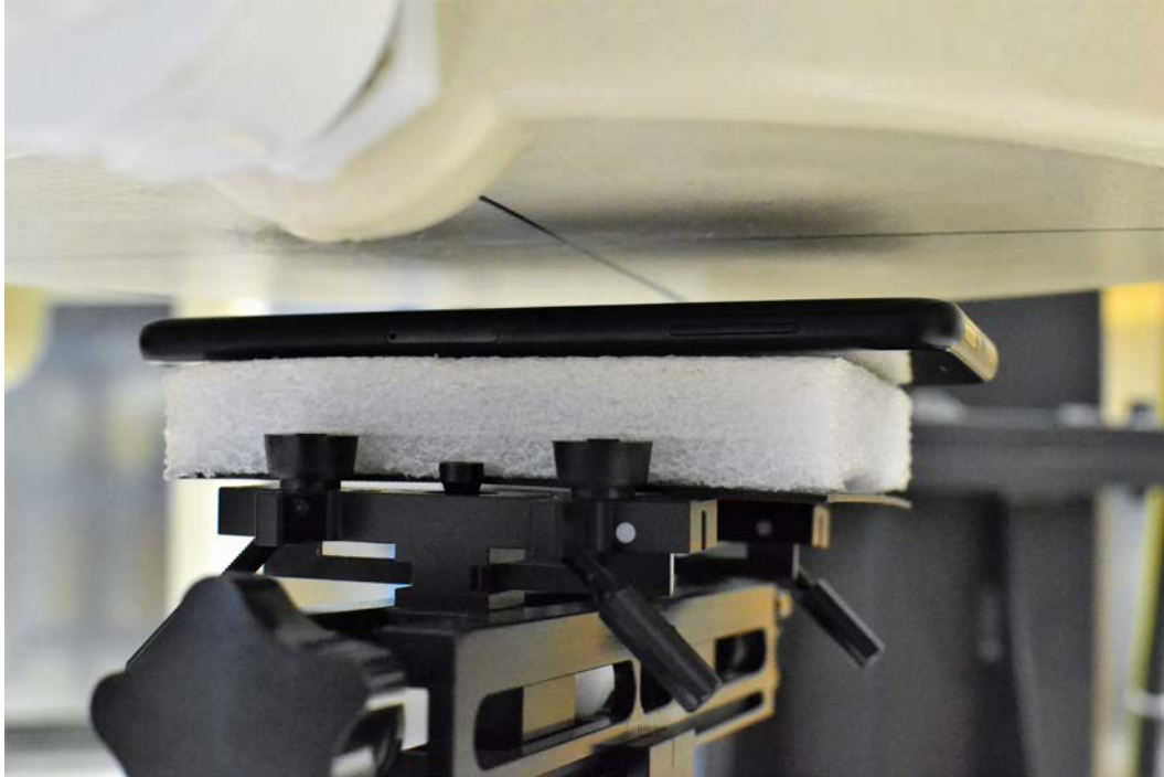
SAR Test Photo 5- Back Side at 1.5 cm
