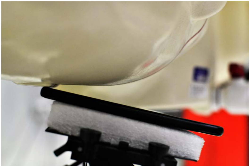
SAR Test Photo 2- Right Tilt
