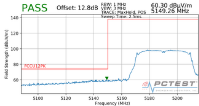
Plot 7-99. Radiated Lower Band Edge Plot (Peak – UNII Band 1)
