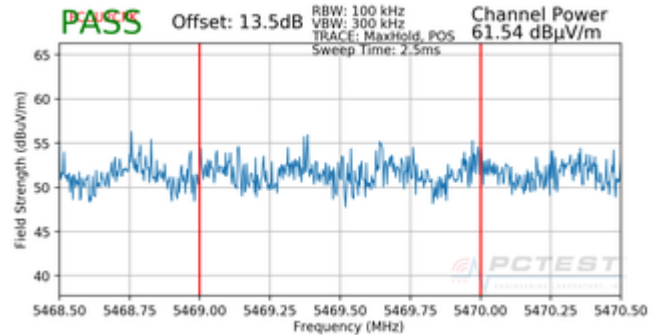
Plot 7-103. Radiated Lower Band Edge Plot (Peak – UNII Band 2C)
