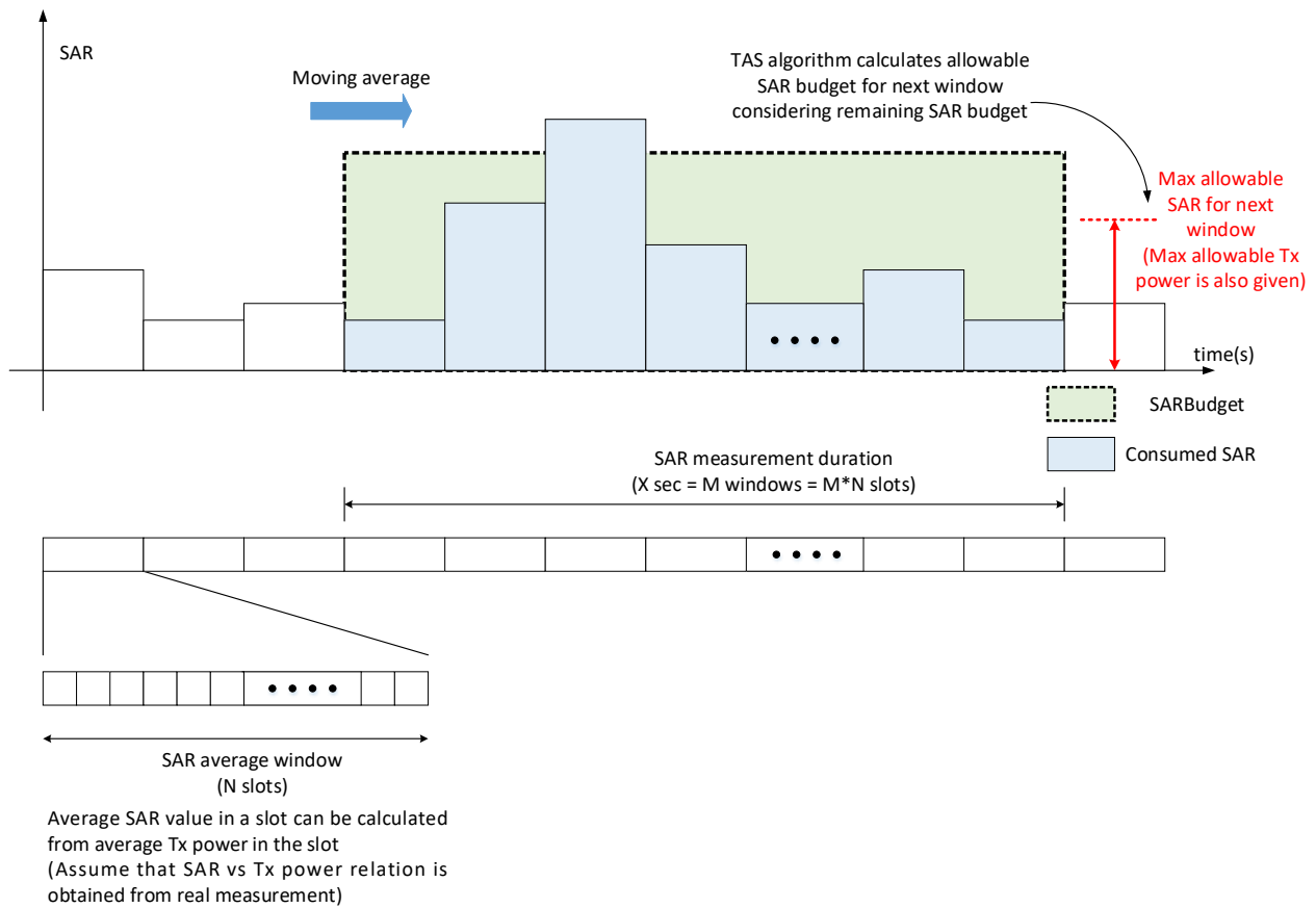
Figure 2.2-1 SAR measurement from Tx power using block-wise processing
