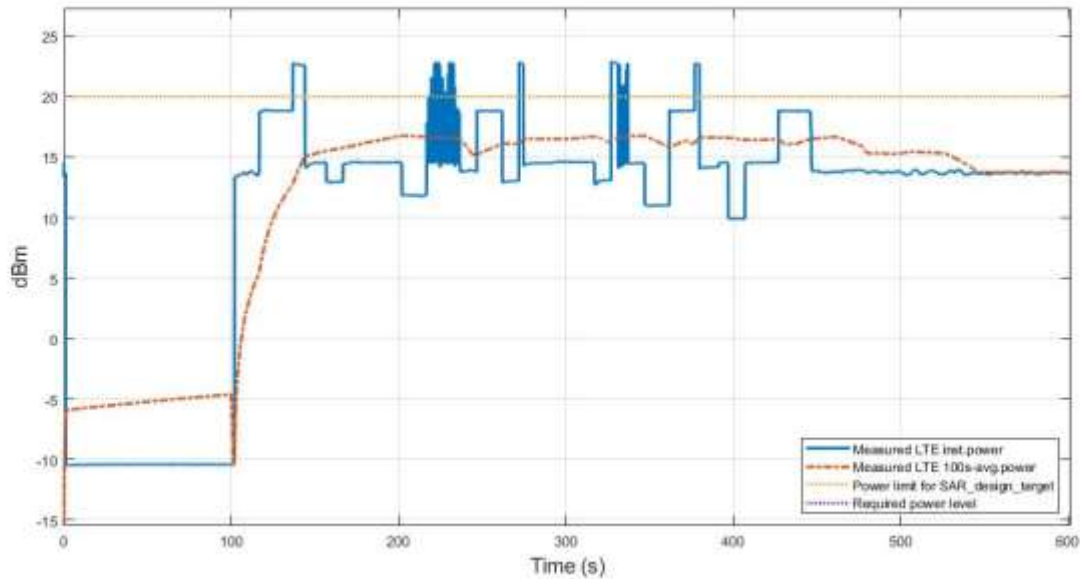
Figure 6.3-9 Conducted Tx power of LTE B7 in TC03
