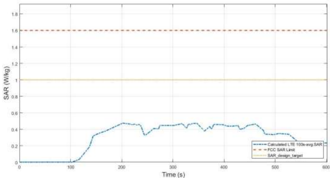
Figure 6.3-10 Total time-averaged SAR in TC03
