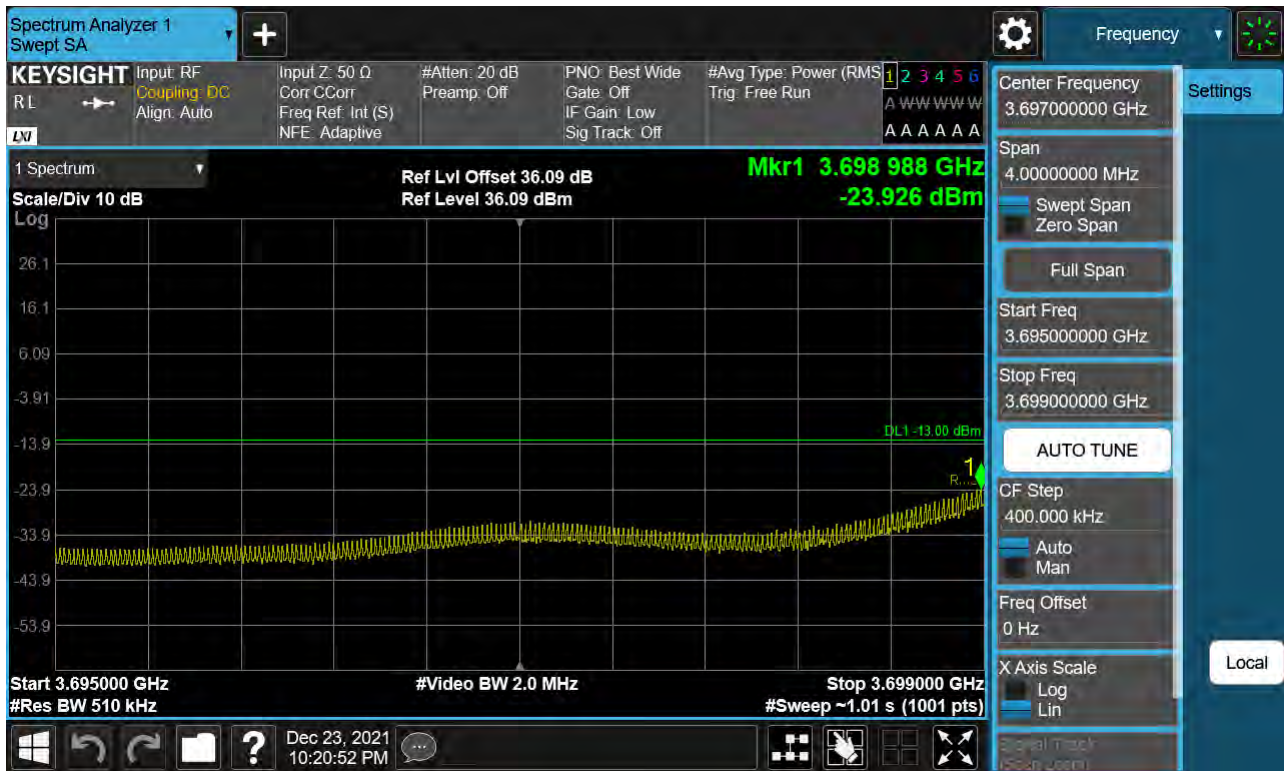
Sub6 n77. Low Band Edge Plot (50 M BW Ch.648334 BPSK 1RB)(2)
