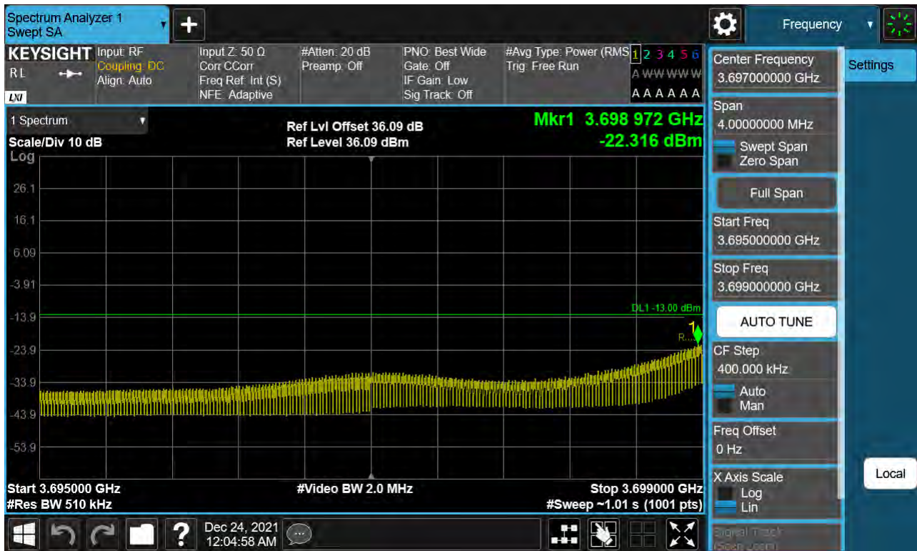
Sub6 n77. Low Band Edge Plot (70 M BW Ch.649000 BPSK 1RB)(2)
