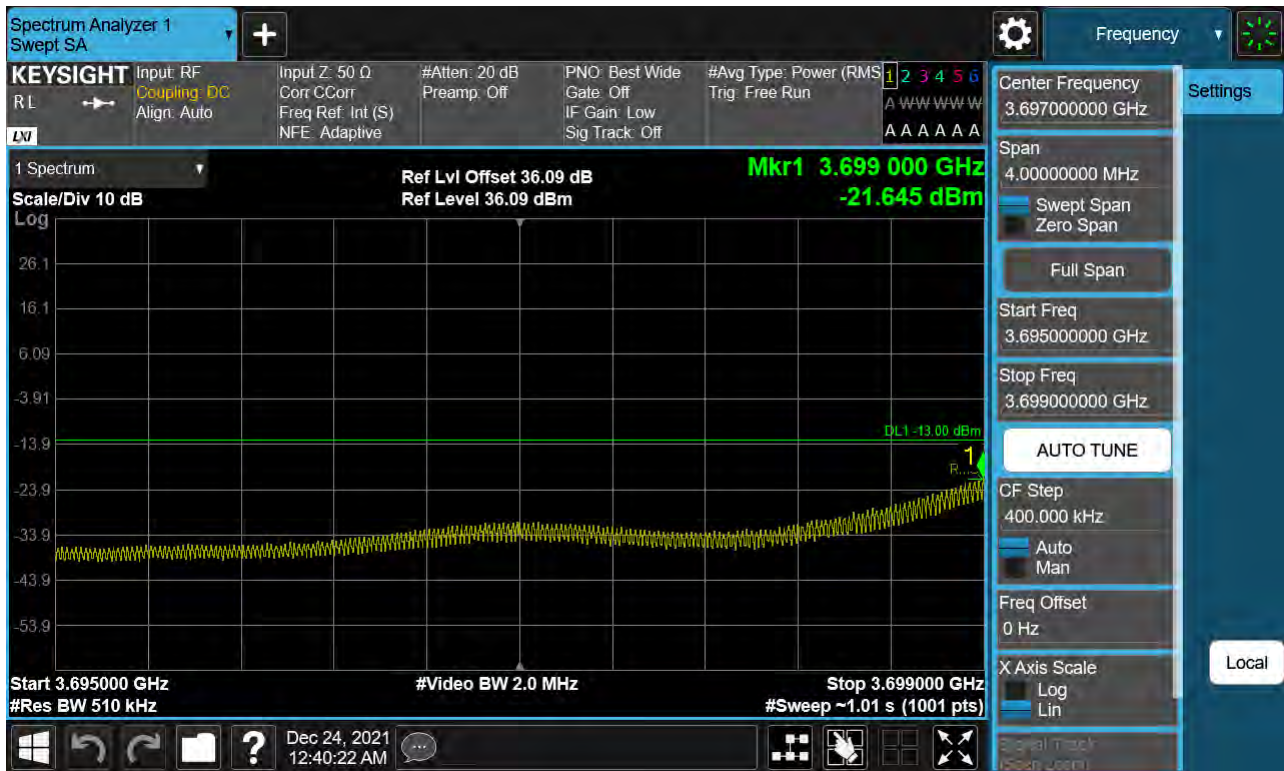
Sub6 n77. Low Band Edge Plot (90 M BW Ch.649668 BPSK 1RB)(2)
