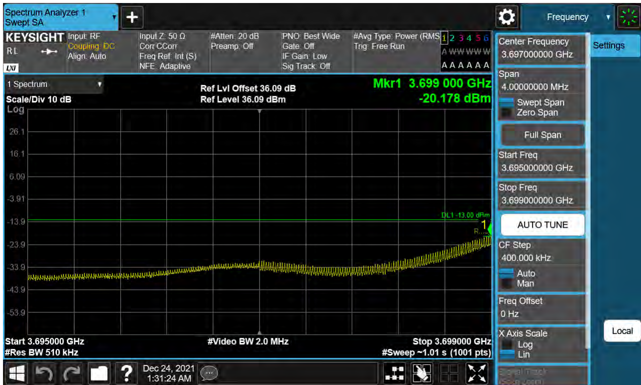
Sub6 n77. Low Band Edge Plot (60 M BW Ch.648668 BPSK 1RB)(2)
