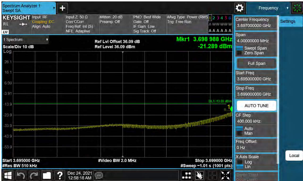
Sub6 n77. Low Band Edge Plot (100 M BW Ch.650000 BPSK 1RB)(2)
