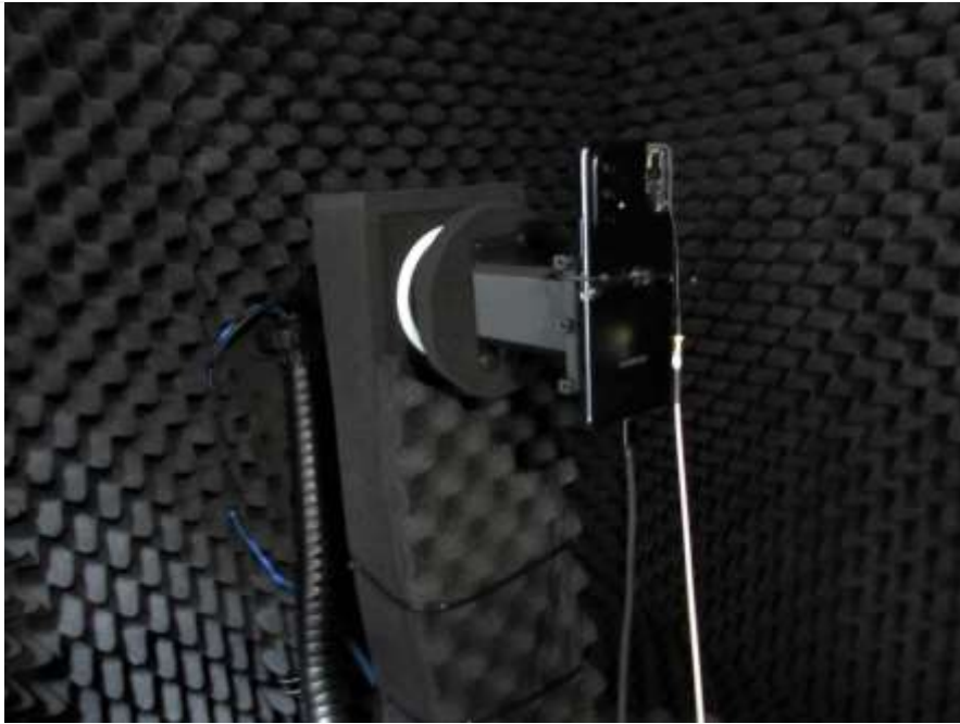
Test setup photo-7 (mmW NR radiated power measurement)
