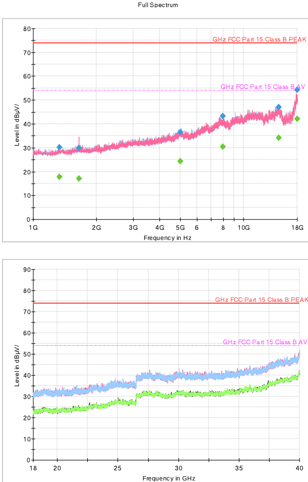
Figure 6: Radiated Emission (1 to 40) GHz, [EUT+Earphone] LTE B5+5G NR n5 High ch Idle
