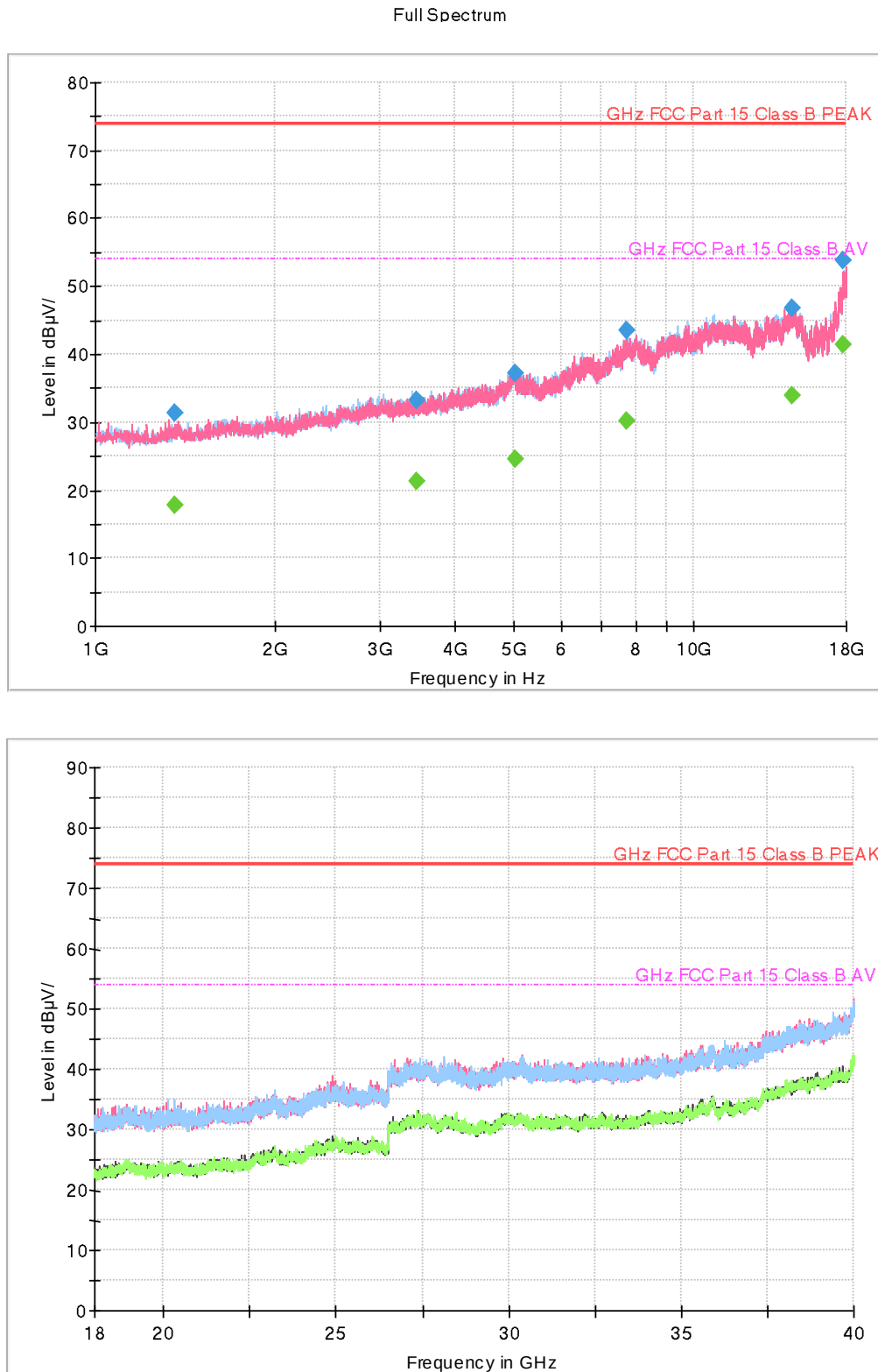
Figure 5: Radiated Emission (1 to 40) GHz, [EUT+TA] LTE B5+5G NR n5 High ch Idle
