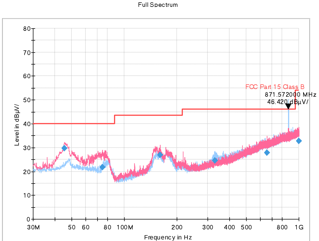
Figure 1: Radiated Emission (30 to 1 000) MHz, [EUT+TA] LTE B5 Low ch Idle
