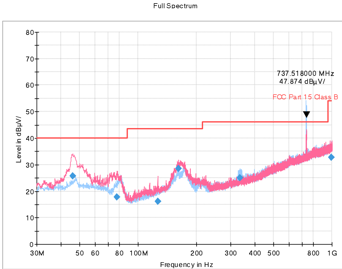
Figure 2: Radiated Emission (30 to 1 000) MHz, [EUT+TA] LTE B12 Middle ch Idle
