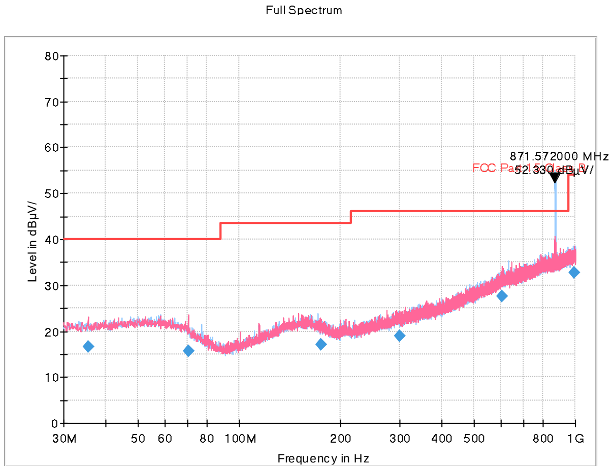
Figure 4: Radiated Emission (30 to 1 000) MHz, [EUT+Earphone] LTE B5 Low ch Idle
