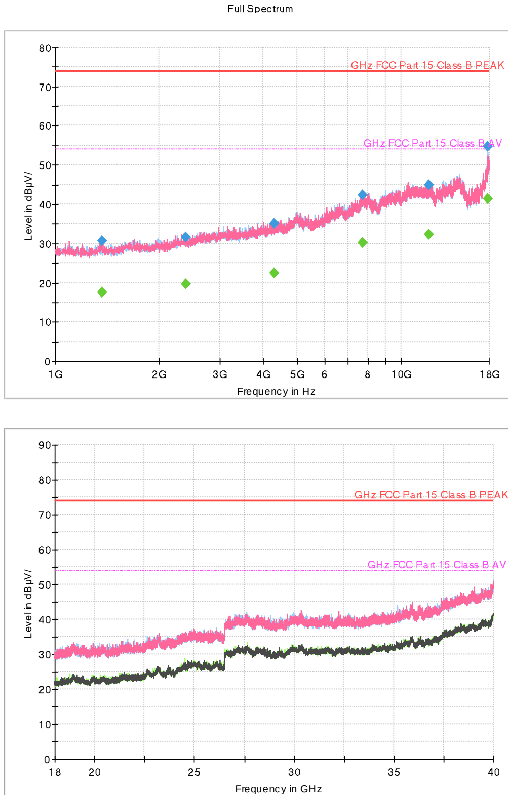
Figure 5: Radiated Emission (1 to 40) GHz, [EUT+TA] LTE B5 Low ch Idle
