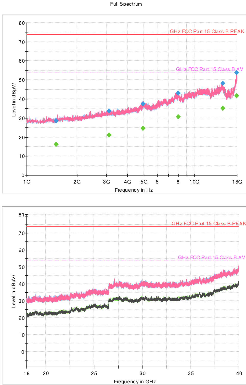
Figure 6: Radiated Emission (1 to 40) GHz, [EUT+Earphone] LTE B5 Low ch Idle
